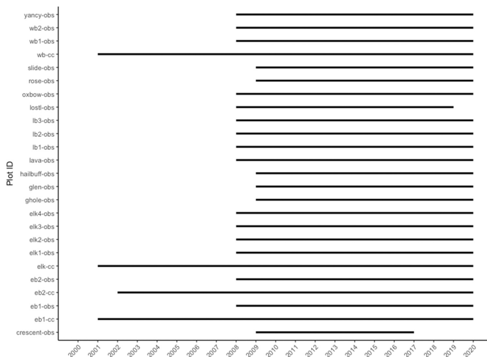
Fig. 2. Monitoring history for the 25 plots included in Ripple et al.’s (2025) analysis, based on data originally collected by Hobbs et al. (2024). Each horizontal line indicates the years during which a specific plot was sampled. Plot identifiers on the y-axis follow Hobbs et al.’s naming convention: “obs” indicates an observational plot and “cc” indicates a control plot at one of four experimental sites. The x-axis spans the full duration of the study period (2001–2020). Although Ripple et al. describe their analysis as a 20-year trend across 25 plots, only 22 plots were sampled in 2020, and just 3 of those had corresponding measurements from 2001. The lack of plot-level continuity undermines the validity of log response ratio estimates that assume matched or equivalent sampling units over time.
