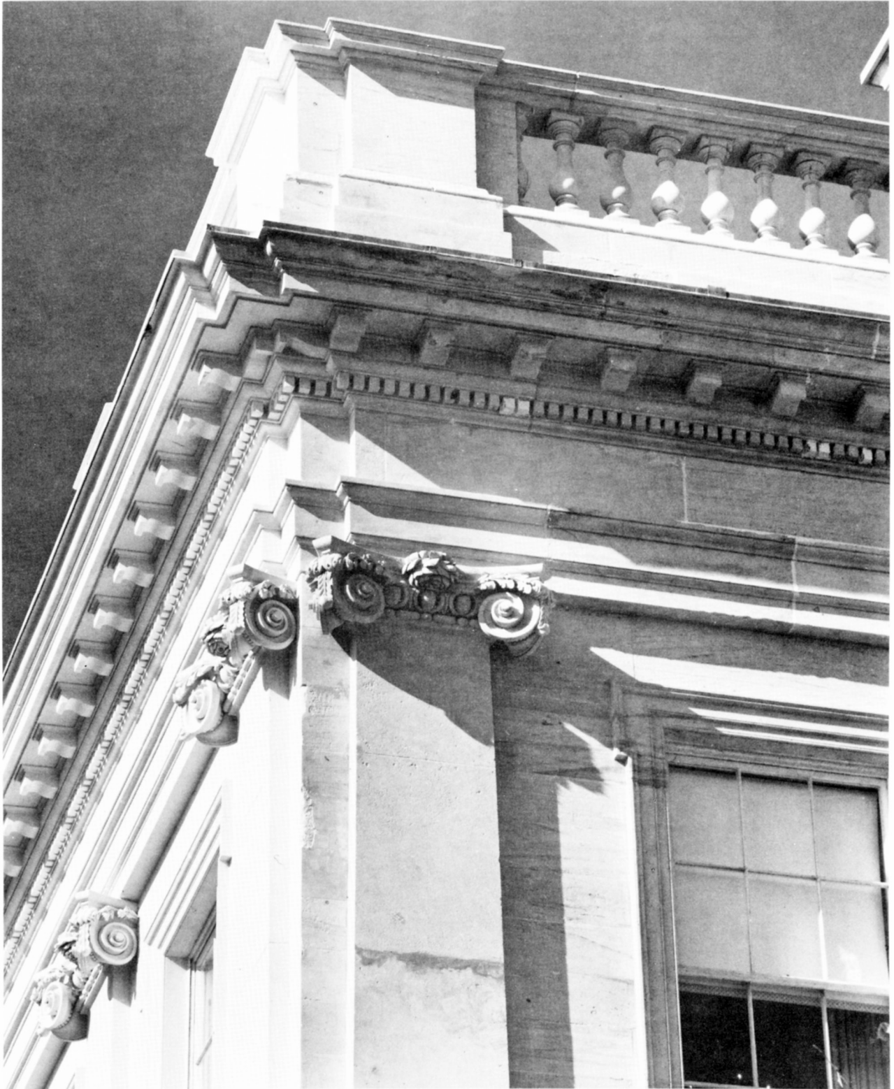
Fig. 8 General view of the upper reaches of the White House at the southeast corner, showing the most concentrated array of stone carving on the building. It encompasses the pilaster capitals and the entire entablature with its architrave, dentils, modillions and overhanging cornice. All of this is topped with the stone balustrade composed of piers, round balusters, and top rail. Some of the individual pieces in the cornice weigh over 3000 pounds and rest over 50 feet above the ground. photo: Jack Boucher, HABS.
