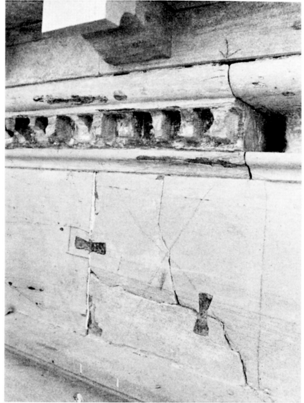
Fig. 26 Close-up of the entablature, just below the cornice. In the frieze area, a pair of cracks were repaired (probably at an early date) with iron cramps. The iron cramps extend into the face of the stone at each end to hold the stones together and keep the loose pieces from falling out. Also note the extensive erosion of the dentils. photo: Bill Allman, Office of the Curator, The White House.
