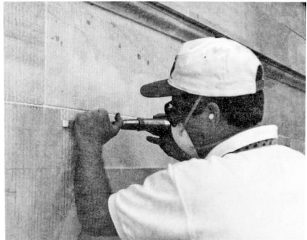
Fig. 33 A stonecutter is chiseling furrows, called tooling, into the new stonework. Only the ground floor walls of the White House have tooled surfaces as opposed to the smooth upper walls which have dressed stone faces. During the repair work, the new tooling is made to match the texture of the adjacent original stonework. photo: Patrick Plunkett.
