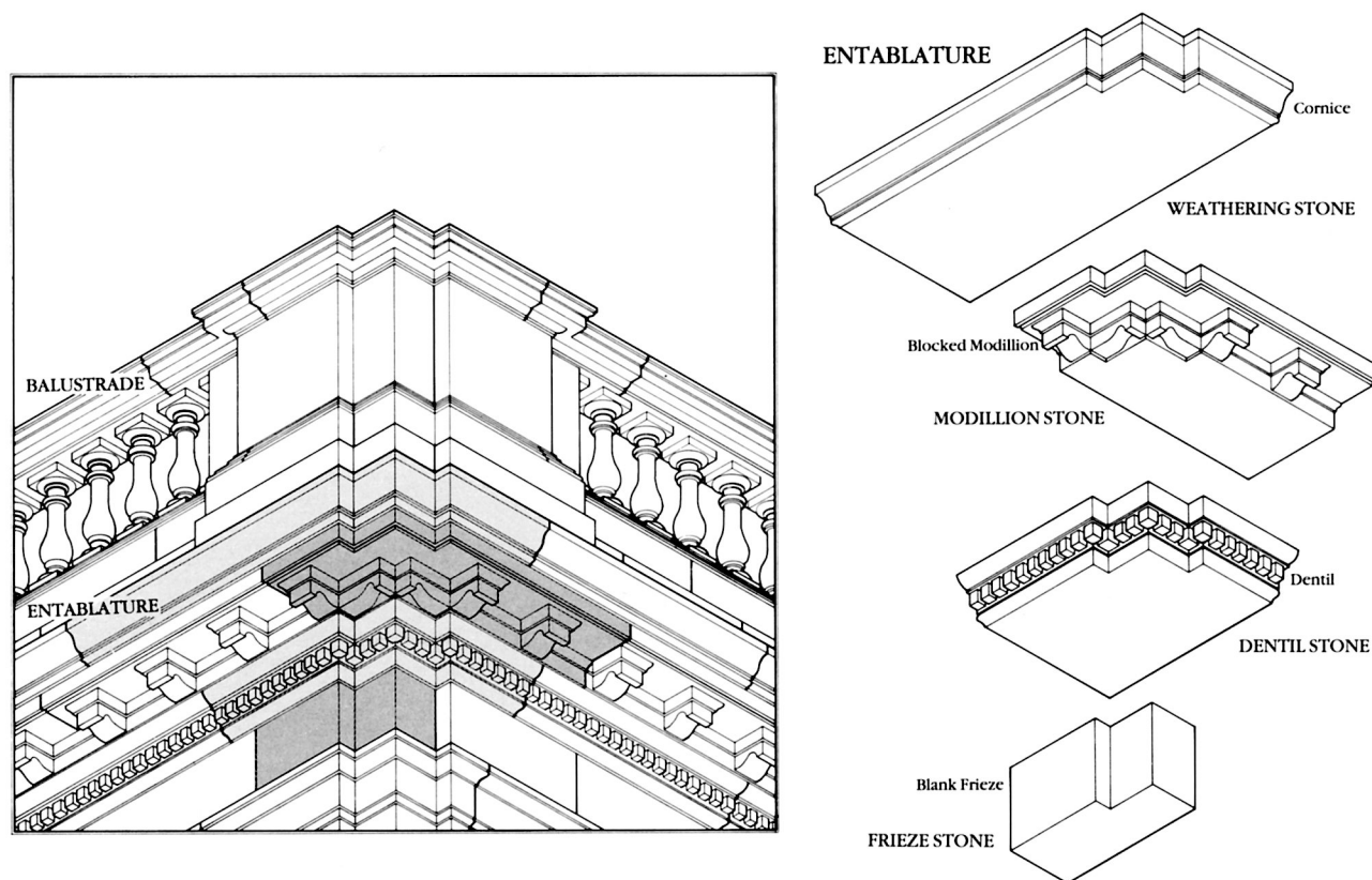
Fig. 32 Isometric drawing looking up at the entablature and roof balustrade of the southwest corner of the White House. A serious crack extending through several layers of stone in the entablature was discovered during the present restoration. While this situation required analysis and repair, it also provided the opportunity to study some of the original construction details. This area is complicated, partly because the stones at the corner have architectural features on both faces of the building, and partly because there are five layers of large stones that comprise the entablature: the weathering stone creating the cornice, the modillion stone, the dentil stone, the blank frieze, and the architrave. The details of four of these stones are drawn off to the side, and show how the original stone carvers planned and executed the overlapping stones to carry the projecting weight. The weathering stone, the upper stone, weighs over 3000 pounds. illustration: Tim Buebner, NPS.
