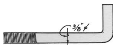
~ TOP PLATE BOLTS ~ Scale 1/2" = 1"
