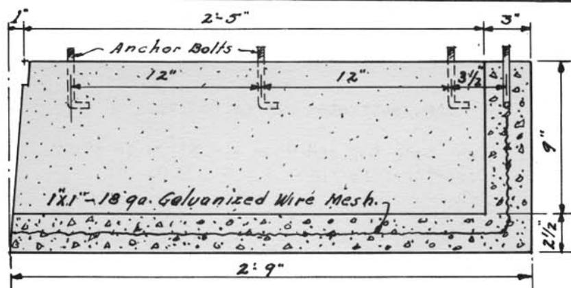
- LONGITUDINAL SECTION OF FIREBOX - Scale - 1 1/2" = 1'-0"
