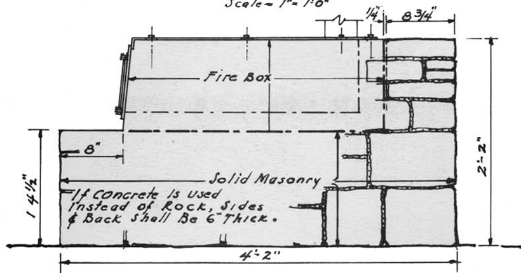
- SIDE ELEVATION - Scale - 1" = 1'-0"
