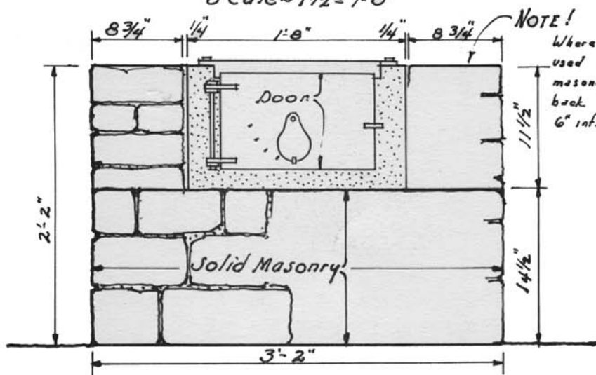
- FRONT ELEVATION - Scale - 1" = 1'-0"
