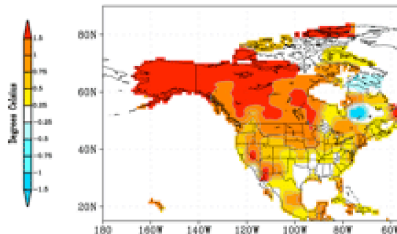
Figure 1. The 1950 to 2007 trend in observed annual averaged North American surface temperature (left). Time series of the annual values of surface temperature averaged over the whole of North America (right). Curve highlights the lower frequency variations after applying a 9-point Gaussian filter to the annual values. Data is the UK Hadley Center's CRUv3 global monthly gridded values. Annual departures are with respect to a 1971–2000 reference.
