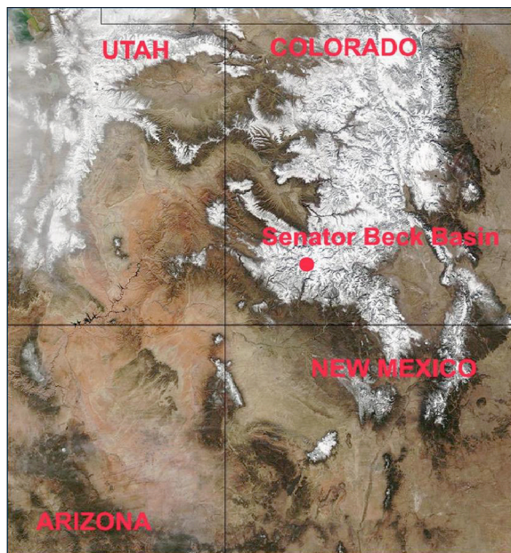
Figure 1. The Four Corners region showing the Senator Beck Basin Study Area location in the San Juan Mountains of Southwestern Colorado, with early winter snowcover. Photo courtesy of NASA.
