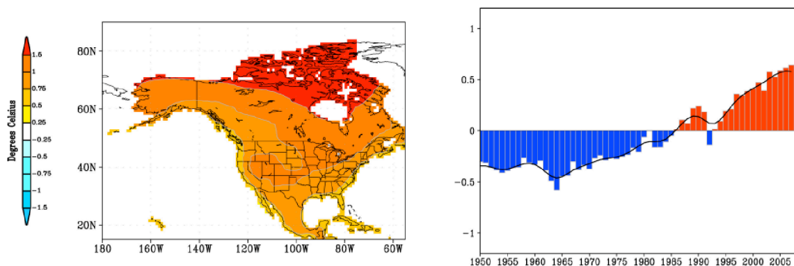
Figure 3. The 1950 to 2007 trend in annual averaged North American surface temperature from 22 IPCC model simulations forced with the estimated greenhouse gas, aerosol, solar and volcanic forcing from 1950–1999, and the business-as-usual emissions scenario (A1B) afterwards. Time series (right) shows the annual values of surface temperature averaged over the whole of North America. Curve highlights the lower frequency variations after applying a 9-point Gaussian filter to the annual values. Annual departures are with respect to a 1971–2000 reference.
