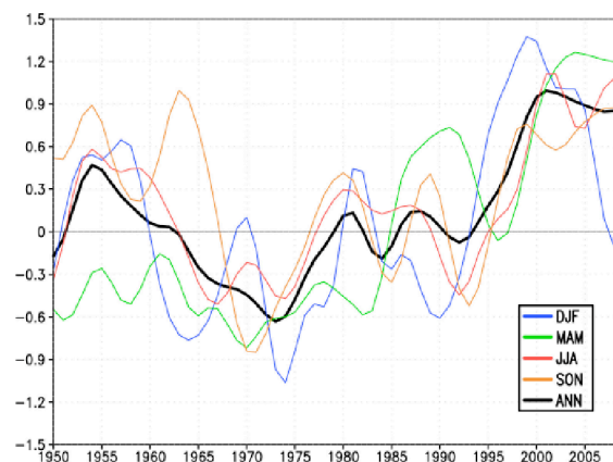
Figure 2. Time series of the annual (black curve) and seasonal (colored curves) values of surface temperature anomalies averaged over the State of Colorado for 1950–2007. Curves are of the 9-point Gaussian filter applied to the raw values in order to highlight lower frequency variations. Data is from the U.S. National Climate Data Center. Departures are relative to a 1971–2000 reference.
