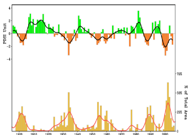
Figure 4. Time series of estimated drought conditions during 1895–2007 averaged over the 11 western states. Top panel is the area-averaged Palmer Drought Severity Index (PDSI), with negative departures indicating dry conditions compared to the region's normal moisture balance. Bottom panel is the % area of the 11 western states experiencing severe drought (PDSI < -3 ). Smooth curves are 9-point Gaussian filters applied to the raw annual values. Data from the National Climate Data Center.
