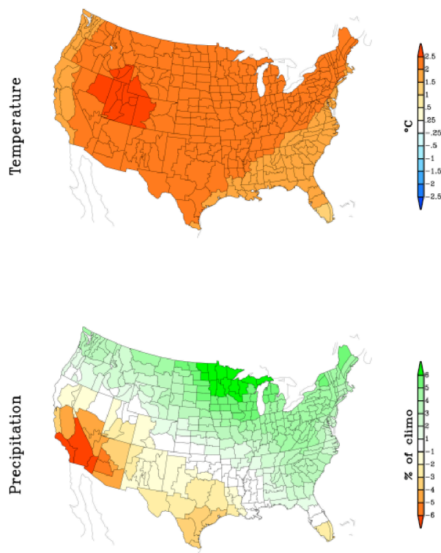
Figure 6. The projected North American surface temperature and precipitation responses at 2050 to business-as-usual emissions scenarios of greenhouse gases and aerosols. Data are from the average of 22 IPCC model simulations forced with the business-as-usual emissions scenario. The anomalies are compared relative to a 1971–2000 reference.
