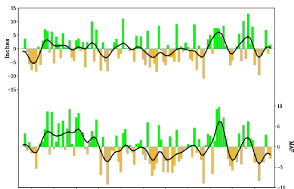
Figure 5. Observed time series of annually averaged precipitation departures during 1895–2007 area-averaged over the Upper Colorado drainage basin (top) and annually averaged Colorado streamflow departures measured at Lee Ferry (bottom). The precipitation data is based on 4-km gridded PRISM data, and the streamflow data is of the “natural” unregulated flows provided by the U.S. Bureau of Reclamation. Smooth curves are 9-point Gaussian filters applied to the raw annual values.
