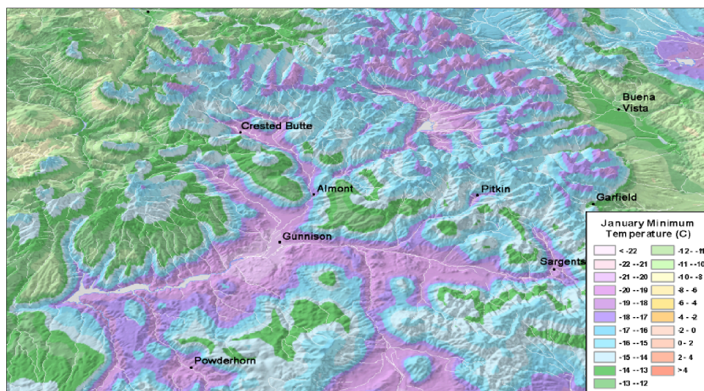
PRISM January 1971–2000 mean minimum temperature in the Gunnison, Colorado area, showing complex relationships between elevation and temperature due to cold air pooling.
