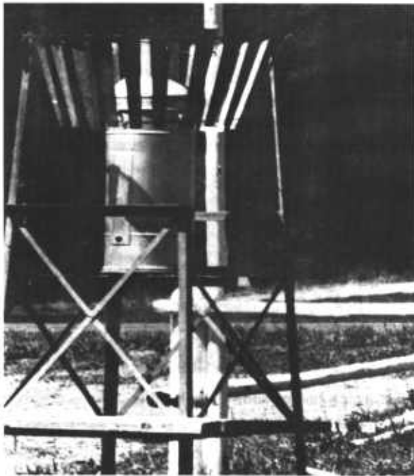
Figure 8.15. — Recording rain gage mounted on tower for snow measurement.
