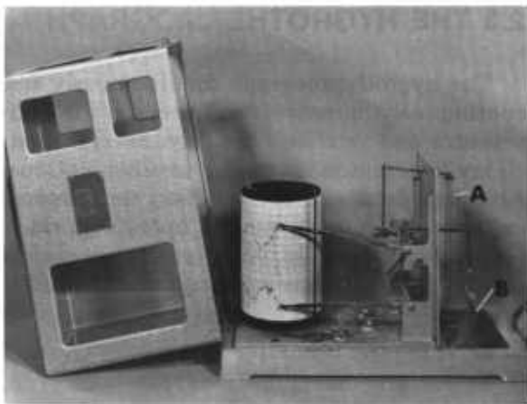
Figure 2.8. — Hygrothermograph equipped with (A) banjo spread hair element and (B) Bourdon Tube.
