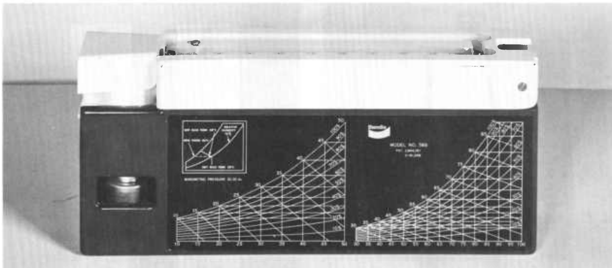
Figure 2.2. — Bendix “Psychron” portable electric fan psychrometer. This instrument allows accurate measurement of RH in the field.
