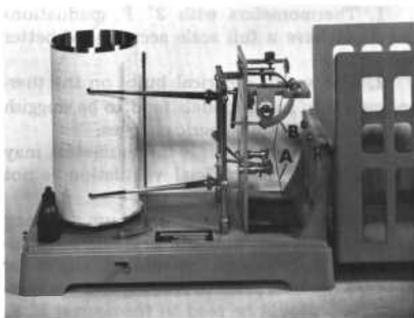
Figure 2.9. — Hygrothermograph equipped with (A) hair bundle element and (B) bimetal strip.
