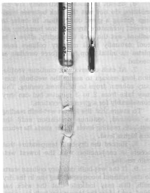
Figure 11.1. — A properly installed wick on wet- and dry-bulb psychrometer.
