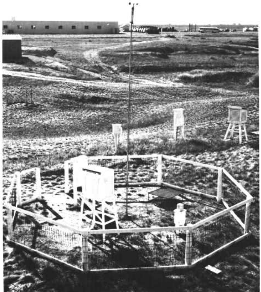
Figure 8.17. — Screen installed over fuel stick at valley station to simulate shade of forest canopy.
