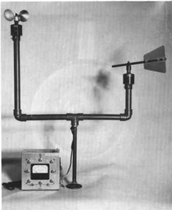
Figure 3.9. — Wind system; anemometer on left, wind vane on right. Remote readout device shows wind-speed (dial) and wind direction (lights).
