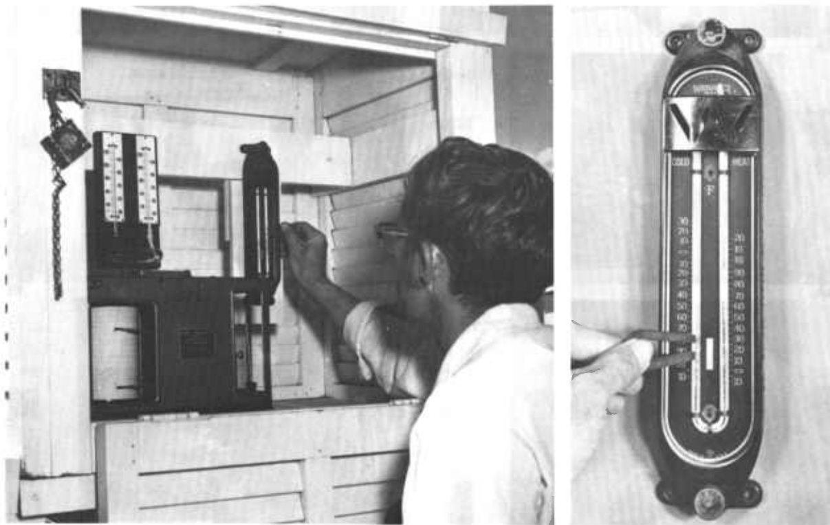
Figure 10.3. — Reading and setting Six's maximum-minimum thermometer.
