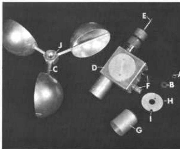
Figure 19.5. — Forester Model 9X150 anemometer (upper) assembled view, (lower) unassembled view: A, Cap nut; B, washer; C, cups; D, housing; E, upper main shaft; F, exterior terminal posts; G, rotor cap; H, balance disc; I, balance weight; J, rotor hub pin.
