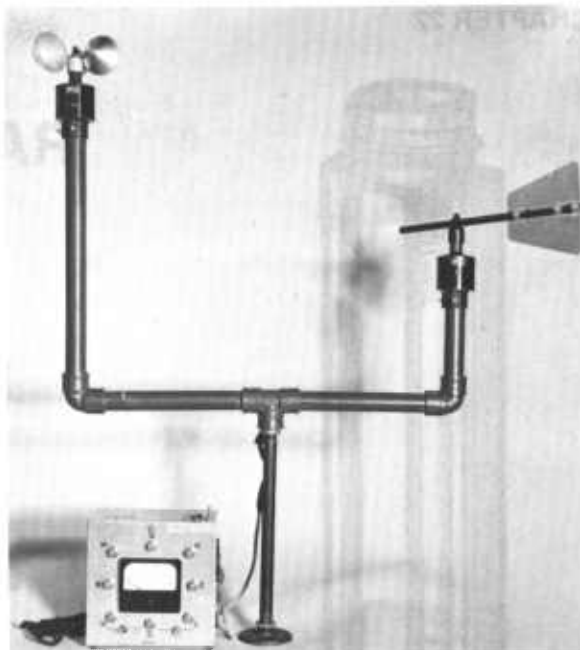
Figure 21.3. — Wind direction system using generator type anemometer and contacting wind vane. Wind direction is indicated by lights; windspeed by arrow on dial.
