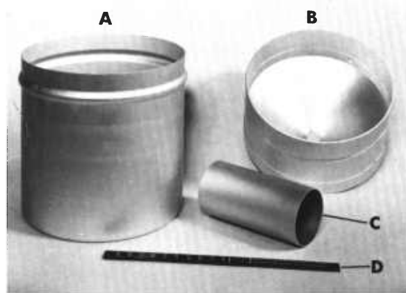
Figure 4.1. — Components of the standard 8-inch rain gage (USDA Forest Service type): A, Overflow cylinder; B, collector; C, measuring tube; D, measuring stick.
