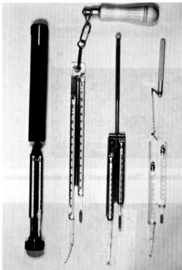
Figure 2.4. — Sling psychrometers. The standard 9½-inch psychrometer (second from left) is often kept as a “spare” at fire-weather stations.
