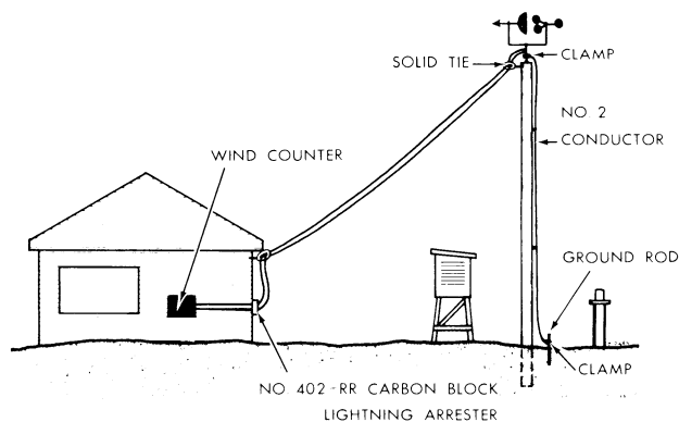
Figure 8.9. — Suggested method for obtaining adequate lightning protection at valley bottom anemometer installations.
