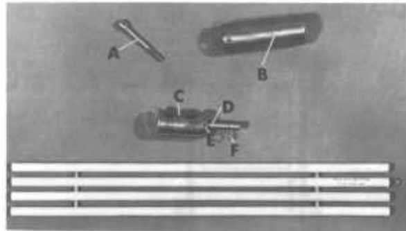
Figure 24.2. — Williams Pocket Firestick Moisture Scale: A, Handle and locking screw; B, cover and 100-gram test weight; C, balance weight; D, balance beam; E, knife edge; F, hook.
