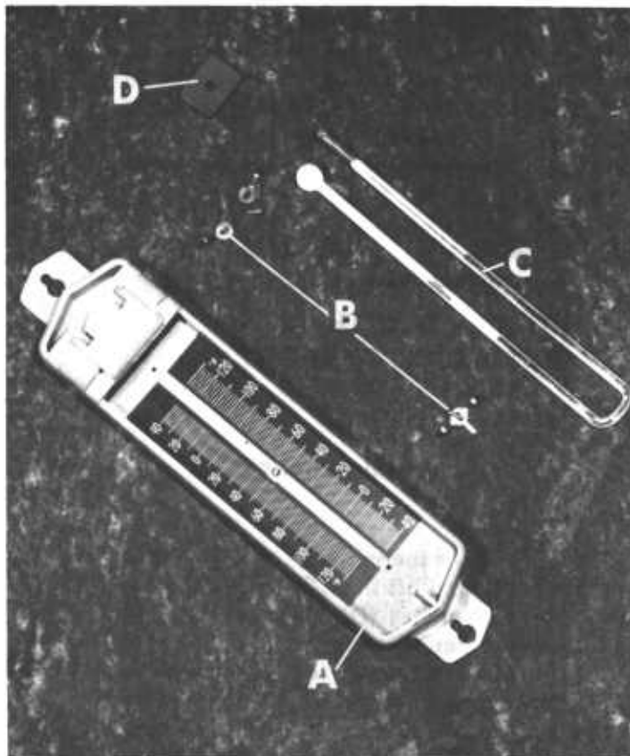
Figure 16.4.— Combined maximum-minimum thermometer; Left, Assembled; right: A, mounting plate; B, thermometer retaining screws and strip; C, thermometer tube; D, magnet.
