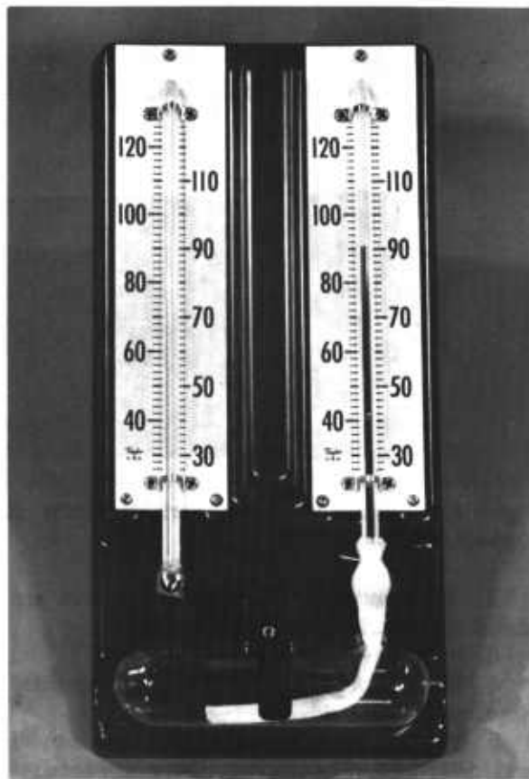
Figure 2.5. — Wet- and dry-bulb hygrometer. The glass reservoir on the bottom must be kept full of water.
