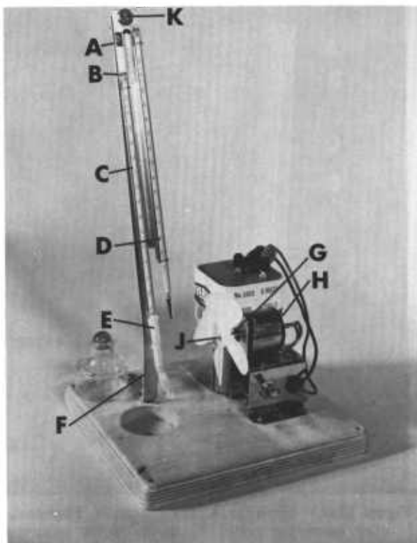
Figure 17.2. — Forester 9X060 electric fan psychrometer (left) and Forest Service electric fan psychrometer (right): A, Thermometer mounting plate; B, thermometer retaining screws and clip; C, wet-bulb thermometer; D, dry-bulb thermometer; E, wet-bulb wick; F, support bracket; G, fan and shaft; H, motor; I, thrust plate; J, fan bushing; K, spacer screw.
