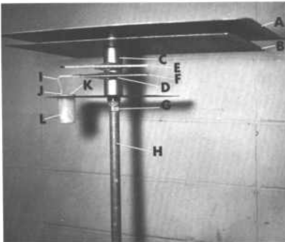
Figure 17.5. — Mortarboard psychrometer: A, Upper radiation shield; B, lower radiation shield; C, spacer; D, thermometer clip; E, dry-bulb thermometer; F, wet-bulb thermometer; G, connectors and couplings; H, support; I, wet-bulb wick; J, plastic tubing; K, water cup cap; L, water cup.
