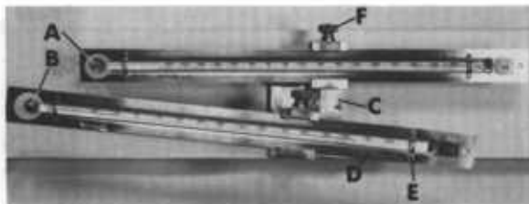
Figure 16.2. — Standard maximum-minimum thermometer mounted in Townsend Support: A, Minimum thermometer; B, maximum thermometer; C, Townsend Support; D, thermometer mounting plate; E, thermometer retaining strip and screws; F, Townsend Support thumbscrew.
