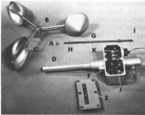
Figure 19.9. — Belfort totalizing anemometer: A, Cap nut; B, hub screw; C, cups; D, housing; E, back cover plate; F, spindle retaining screw; G, spindle; H, upper ball bearings; I, worm gear; J, worm wheel with pins; K, terminal block assembly; L, thumbscrew.
