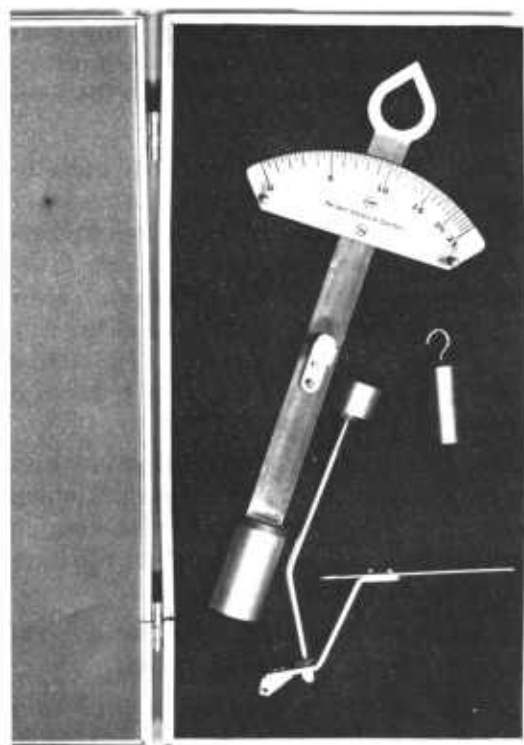
Figure 5.3. — Portable fuel moisture scale.
