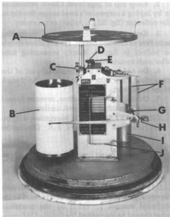
Figure 22.3. — Weighing rain gage — weighing and recording assembly: A, Weighing platform; B, chart drive assembly; C, stop screw; D, spring adjusting screw; E, thumb nut (red); F, linkage assembly; G, magnification bar (first traverse); H, magnification bar (second traverse); I, dash pot; J, pen lifter.
