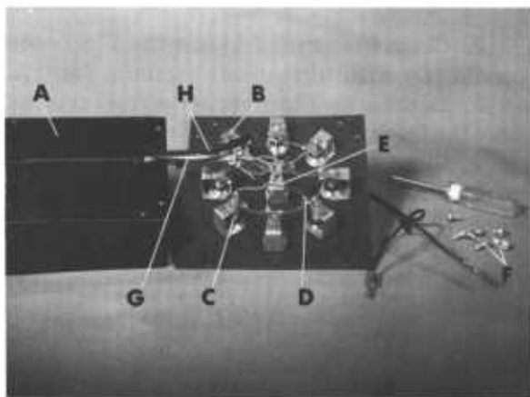
Figure 21.2. — Stewart wind direction system — the wind indicator dial: A , Cabinet; B , indicator panel; C , land socket; D , lamp socket terminal; E , anemometer flasher unit; F , front panel screws; G , multiple conductor cable; H , battery cable.
