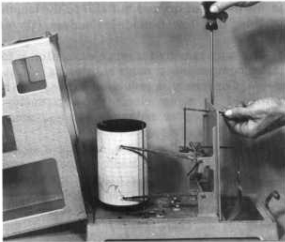
Figure 18.5. — Adjusting the magnification bar on a Belfort hygrothermograph.
