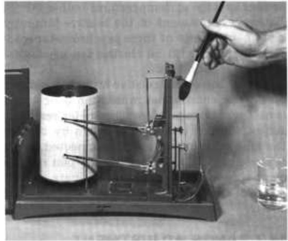
Figure 18.6. — After saturating hair element with a soft camel's hair brush, the humidity pen should indicate between 91 and 95 percent relative humidity.
