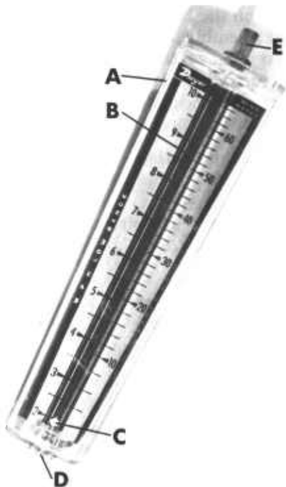
Figure 19.12. — Dwyer hand-held wind meter: A , Outer shell; B , inner tube; C , indicator ball; D , bottom plug; E , top stem.
