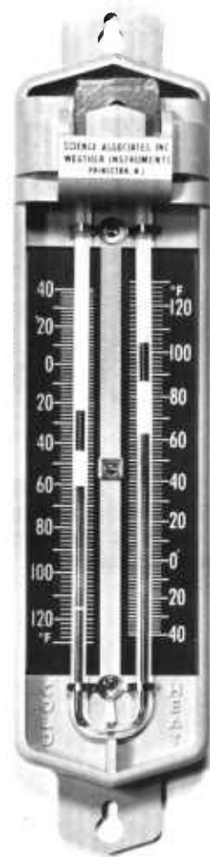
Figure 1.3.—Six's type maximum-minimum thermometer. Maximum temperature is read on the right, minimum temperature is read on the left.
