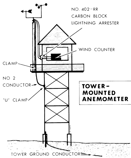
Figure 8.8. — Suggested method for obtaining adequate lightning protection at lookout anemometer installations: Left , Anemometer pole on tower; right , anemometer pole on ground.
