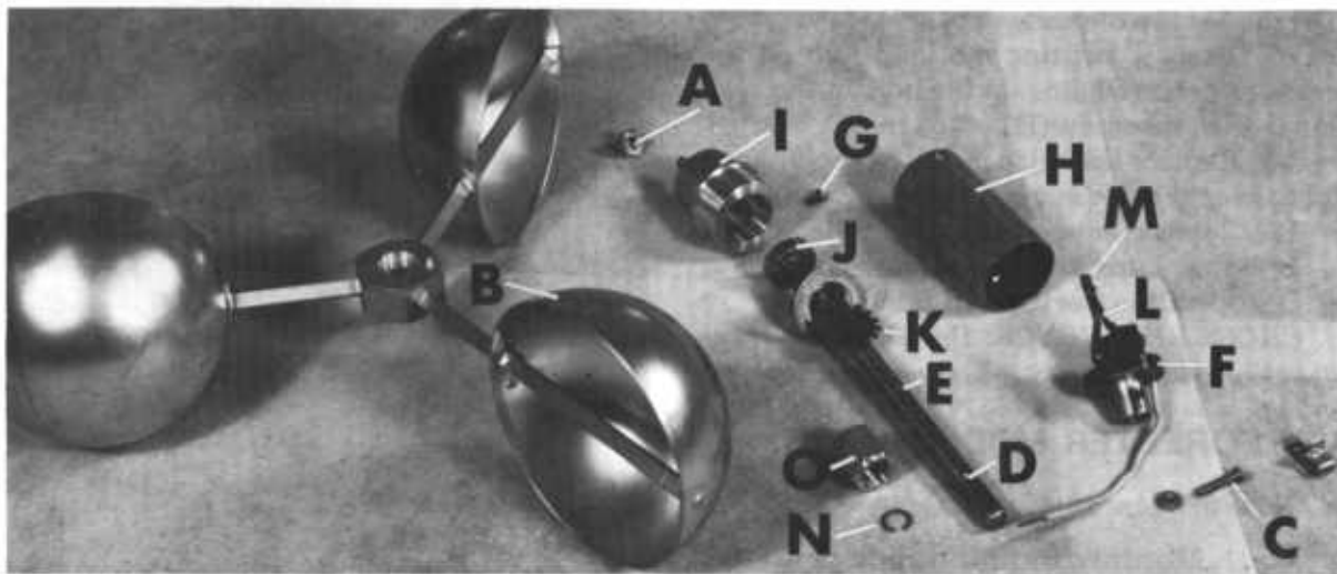
Figure 19.6. — Chisholm Model 2B3C anemometer: A, Cap nut; B, cups; C, electrical unit retaining bolt; D, main shaft; E, electrical unit mounting point; F, electrical unit; G, cylinder retaining screw; H, revolving cylinder; I, cylinder head; J, roller bearings; K, sprocket gear; L, contact fingers; M, contact points; N, mounting nut lockring; O, mounting nut.
