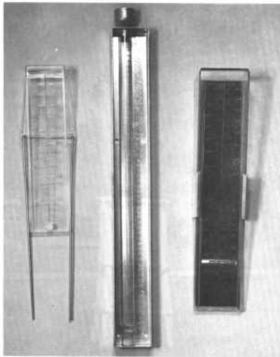
Figure 4.4. — Several types of direct reading small orifice rain gages.
