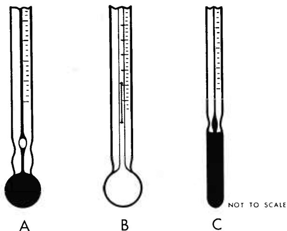
Figure 1.1. — Liquid-in-glass thermometers: A, Mercury-filled maximum thermometer; B, alcohol-filled minimum thermometer; C, standard dry-bulb mercury thermometer.
