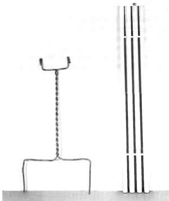
Figure 5.1. — One-half-inch ponderosa pine fuel moisture indicator sticks and wire mounting rack (two required per installation).
