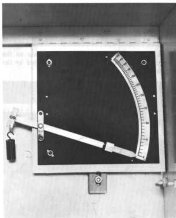
Figure 15.1. — Use a 100-gram test weight to check the calibration of the Appalachian scale.
