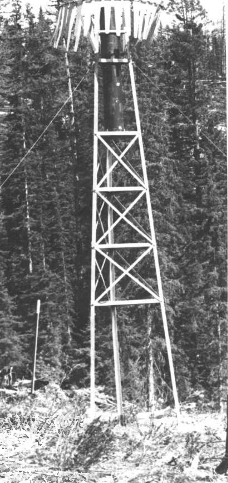
Figure 4.11. — Alter type rain gage shield mounted around a precipitation storage gage.
