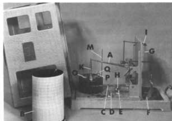
Figure 18.2. — Belfort hygrothermograph. This clock is mounted to the base in this instrument. Components are: A, Temperature pen arm; B, chart and chart drum; C, relative humidity pen arm; D, pen arm shifting rod lever; E, temperature pen adjustment knob; F, Bourdon tube (temperature sensor); G, banjo spread hair element (relative humidity sensor); H, relative humidity pen adjustment knob; I, magnification bar; K, arbor or spindle; M, pen arm shifting rod; O, pinion shaft; P, pinion gear; Q, clock winding key.
