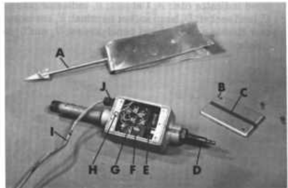
Figure 21.1. — Stewart wind direction system — the electric wind vane component: A, Arrow; B, front cover; C, orientation scribe mark; D, spindle; E, contact roller; F, terminal block binding post; G, anemometer wire binding post; H, ground connection screw; I, multiple conductor cable; J, nut and compression sleeve.
