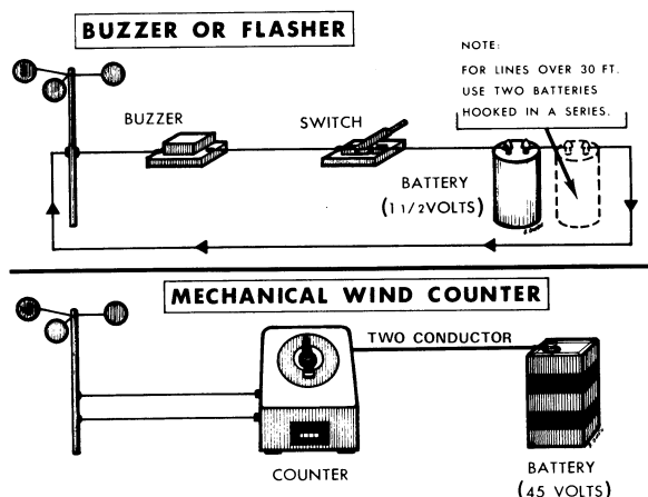
Figure 20.1. — Wiring diagrams: Upper, Buzzer or flasher; lower, mechanical wind counter.
