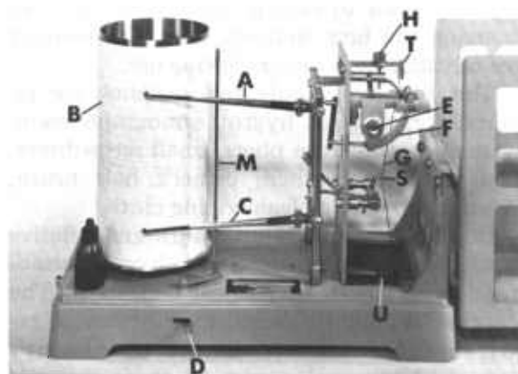
Figure 18.3. — Weather Measure hygrothermograph. This hygrothermograph has a battery-operated clock in the chart drum. Components are: A, Temperature pen arm; B, chart and chart drum; C, relative humidity pen arm; D, pen arm shifting rod lever; E, temperature pen adjustment knob; F, bimetal strip (temperature sensor); G, hair bundle (relative humidity sensor); H, relative humidity pen adjustment knob; M, pen arm shifting rod; S, hooked magnification lever; T, upper hair jaw; U, lower hair jaw.
