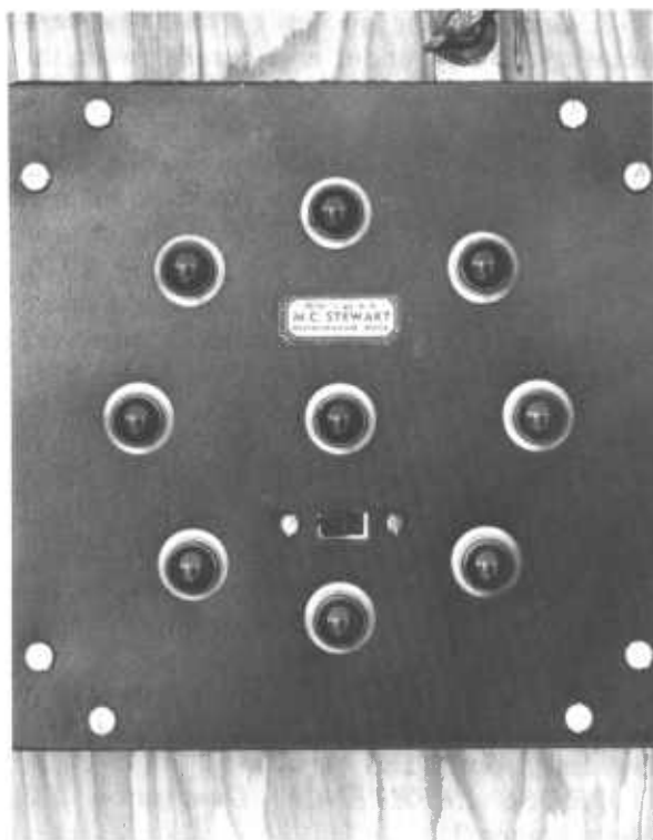
Figure 8.12. — Wind direction indicator. Lighted lamps indicate wind direction.
