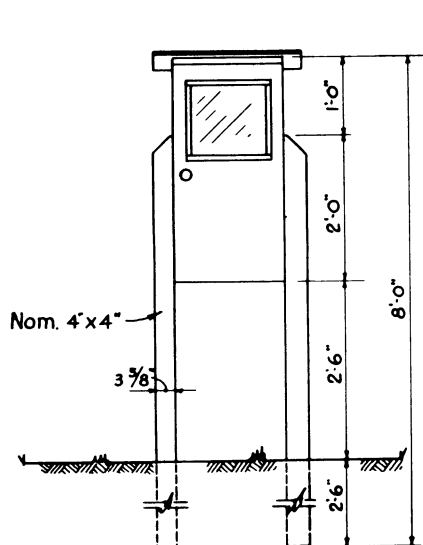
SHELTER MOUNTING DETAIL
