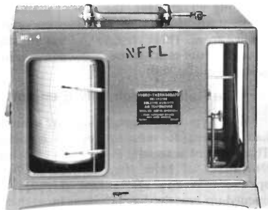
Figure 2.7. — The hygrothermograph. The upper pen records temperature; the lower pen records relative humidity.
