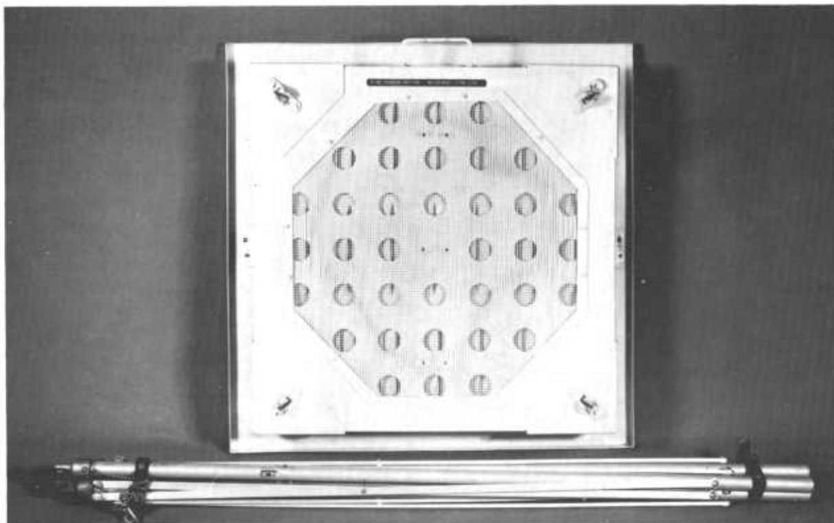
Figure 1.6. — Portable aluminum instrument shelter — knocked down for easy transport to the field.
