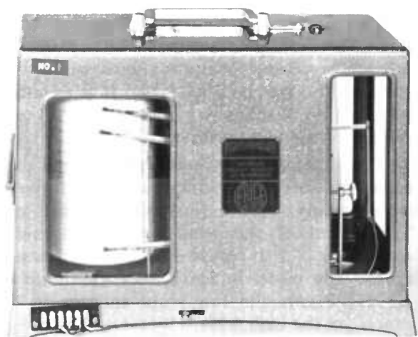
Figure 3.6. — A hygrothermoaerograph (HTAG). Uppermost pen arm has been installed to record wind movement.
