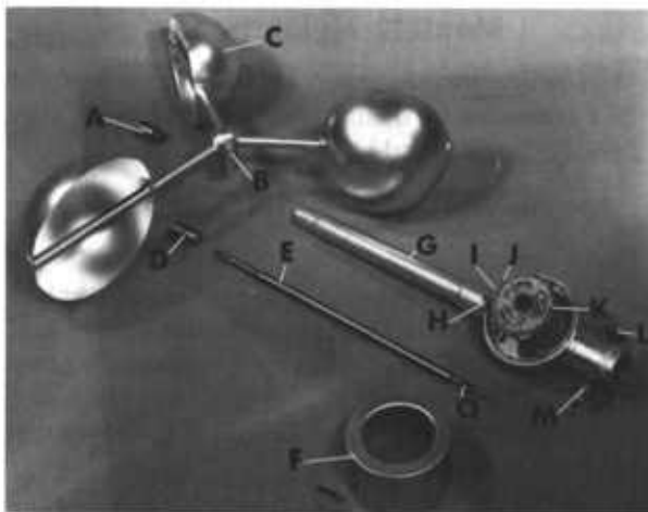
Figure 19.10. — Friez dial type anemometer: A, Oil cup-cap nut; B, rotor hub set screw; C, cups; D, top bushing; E, spindle with worm; F, dial cover plate; G, housing; H, gears; I, 1/60-mile contact; J, contact adjustment screw; K, 1-mile contact; L, thumbscrew clamp; M, grounded terminal; N, 1/60-mile terminal; O, 1-mile terminal; P, oil point plug; Q, outer dial wheel; R, inner dial wheel; S, 1-mile contact pin; T, dial screw; U, location of 10-mile bar.
