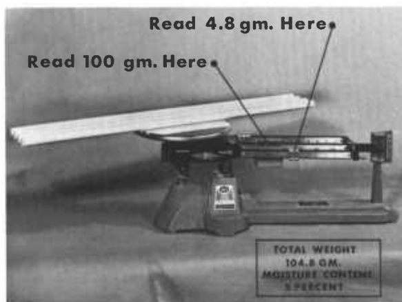
Figure 15.9. — Weighing fuel stick with triple beam balance. This stick weighs 104.8 grams thus indicating a moisture content of 5 percent as indicated on first scale bar.
