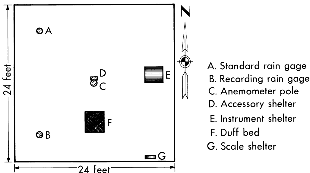
Figure 7.1. — Ground plan for a standard fire-weather station.
