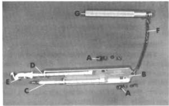
Figure 17.6. — Sling psychrometers: A, Thermometer retaining clip; B, mounting plate; C, dry-bulb thermometer; D, wet-bulb thermometer; E, wet-bulb wick; F, sling chain; G, sling handle.
