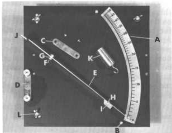
Figure 24.1. — The Appalachian scale; A, Backplate with calibrated scale; B, beam stop plug; C, front pivot plate; D, rear pivot plate; E, beam; F, beam pivot shaft; G, beam pivot shaft spacer; H, sliding weight setscrew; I, sliding weight; J, beam link or hook; K, 100-gram test weight; L, mounting bracket wing nut.
