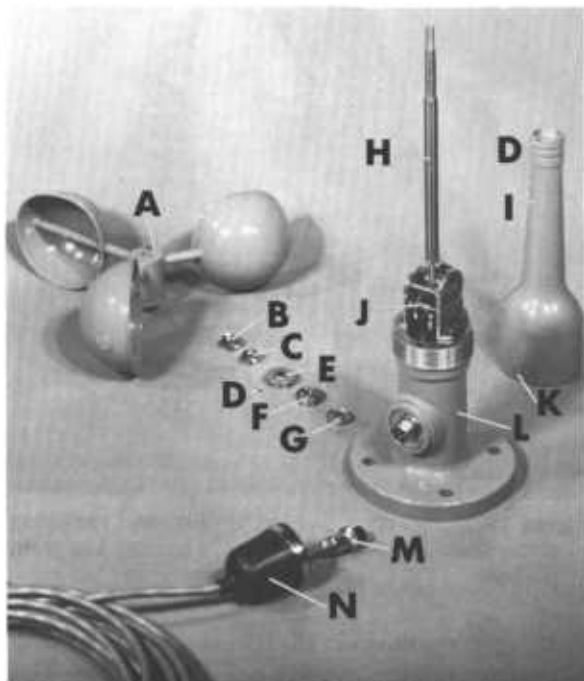
Figure 19.11. — Weather Measure W164 contact anemometer: A, Cups; B, cap lock nut; C, cap nut; D, top lock screw; E, bearing oil seal; F, top bearing; G, bearing oil seal; H, drive shaft with worms; I, top housing; J, drive gear; K, top housing lock pin; L, bottom housing; M, cannon plug; N, weather boat.
