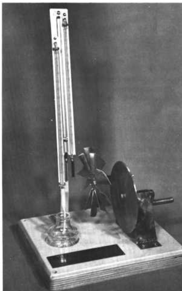
Figure 2.3. — Hand fan psychrometer, USDA Forest Service type.
