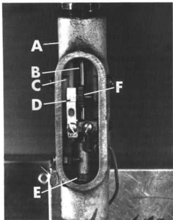
Figure 19.7. — Stewart aluminum cup anemometer: A, Housing; B, spindle; C, bearing block; D, contact leaf spring; E, lower thrust bearing; F, pinion gear.
