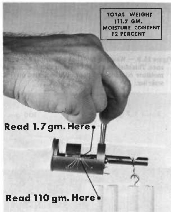
Figure 15.7. — Weighing fuel moisture stick on Williams pocket scale. This stick weighs 111.7 grams so moisture content is 12 percent as indicated on scale.
