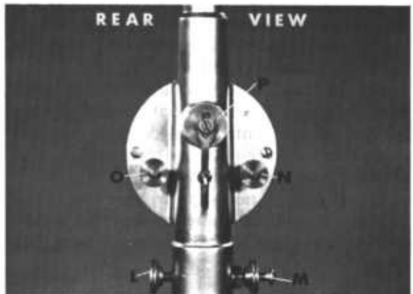
Figure 19.10. — Friez dial type anemometer: A, Oil cup-cap nut; B, rotor hub set screw; C, cups; D, top bushing; E, spindle with worm; F, dial cover plate; G, housing; H, gears; I, 1/60-mile contact; J, contact adjustment screw; K, 1-mile contact; L, thumbscrew clamp; M, grounded terminal; N, 1/60-mile terminal; O, 1-mile terminal; P, oil point plug; Q, outer dial wheel; R, inner dial wheel; S, 1-mile contact pin; T, dial screw; U, location of 10-mile bar.
