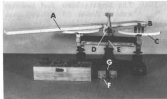
Figure 24.5. — Harvard balance: A, One-half-inch fuel sticks; B, 100-gram weight; C, pan; D, knurled adjusting knob; E, main bearing; F, main bearing cover plate; G, lock.
