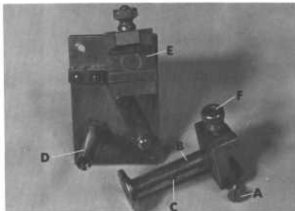
Figure 16.3. — Unassembled Townsend Support: A, Spinner clamp retaining screw; B, spinning clamp; C, oil hole; D, spinner shaft; E, upper clamp; F, thumbscrew.
