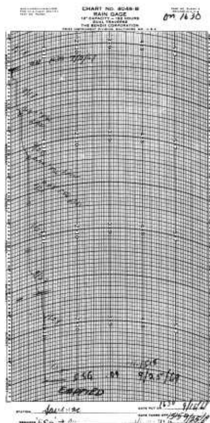
Figure 4.7. — Weighing rain gage chart record. The first 6 inches of rain is recorded on upper traverse of pen.
