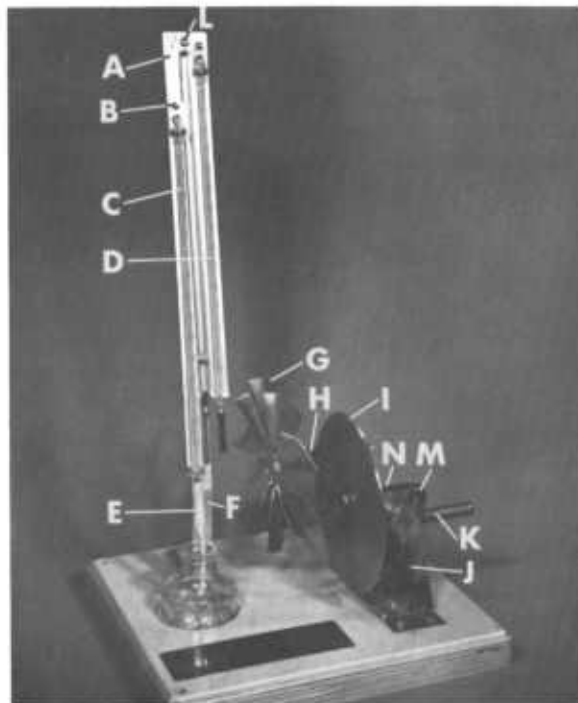
Figure 17.3. — Hand fan psychrometer: A, Thermometer mounting plate; B, thermometer retaining screw and clip; C, wet-bulb thermometer; D, dry-bulb thermometer; E, wet-bulb wick; F, support bracket; G, fan and shaft; H, fan pulley; I, drive wheel; J, fan pedestal; K, crank; L, spacer screw; M, crankshaft; N, oil hole.
