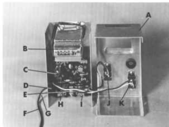
Figure 20.4. — Stewart electronic odometer: A, Front cover; B, mechanical counter; C, test lamp; D, rubber grommet; E, fuse; F, negative battery wire; G, positive battery wire; H, anemometer ground wire (positive) spring clip; I, anemometer wire negative spring clip; J, counter “off-on” switch; K, test lamp “on” switch.
