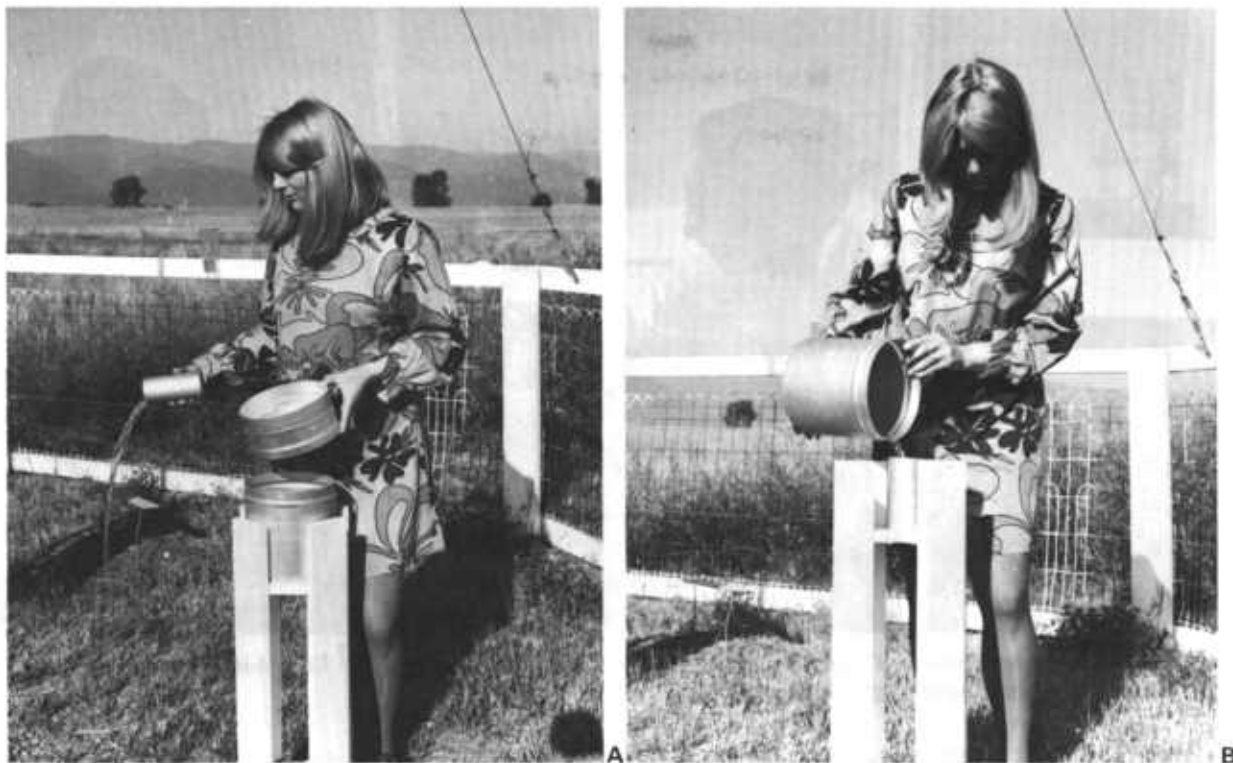
Figure 14.2. —Procedure when measuring tube overflows: A, Dump full tube and record 0.50 inch; B, pour excess into tube and measure.
