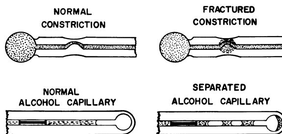
Figure 16.1 — Thermometer defects: Top , Normal and fractured constrictions in maximum thermometers; bottom , normal and separated alcohol capillaries in minimum thermometers.
