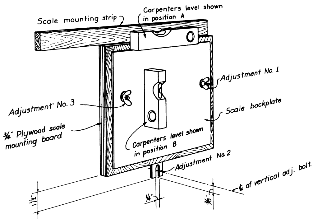
PERSPECTIVE VIEW SCALE LEVELING DETAIL
