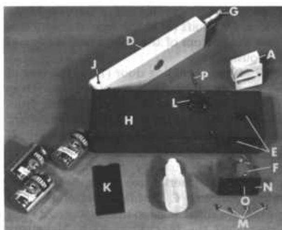
Figure 17.4. — Portable electric fan psychrometers: A, Air intake; B, dry-bulb thermometer; C, retaining strip; D, thermometer holder; E, air intake cylinder; F, fan and motor; G, wet-bulb thermometer and wick; H, psychrometer housing; I, retaining screw; J, thermometer holder shaft; K, sliding door; L, switch; M, motor mounting plate; N, fan shaft; O, fan shaft; P, housing screws.
