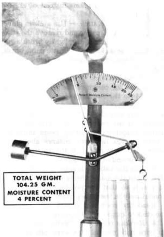
Figure 15.5. — Weighing fuel moisture stick on Chisholm portable scale. This stick weighs 104.25 grams so its moisture content is 4 percent as indicated by the pointer.
