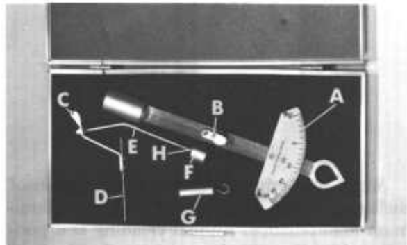
Figure 24.3. — Forester 9X120 portable fuel moisture scale, Chisholm model: A, Scale; B, scale beam support bracket; C, fuel stick suspension loop; D, pointer; E, scale beam shaft; F, scale beam weight; G, 100-gram test weight; H, scale beam weight adjustment nut.
