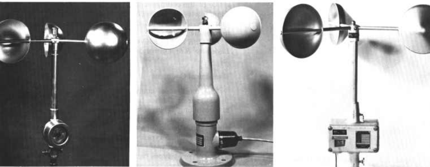
Figure 3.5. — Totalizing-type anemometers equipped with both 1/60-mile and 1-mile contacts: Left , Self-contained dial readout; center , without self-contained readout; right , self-contained counter readout.
