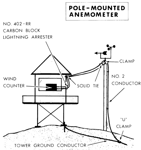
Figure 8.8. — Suggested method for obtaining adequate lightning protection at lookout anemometer installations: Left , Anemometer pole on tower; right , anemometer pole on ground.
