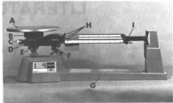
Figure 24.4. — Triple beam balance: A, Platform; B, balance cup; C, knurled adjustment knob; D, friction plate; E, bearing cover; F, bearing cover; G, base; H, poise (sliding weights); I, beam.
