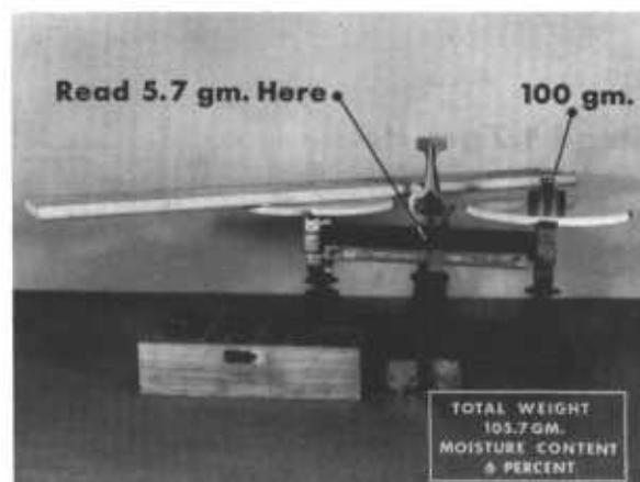
Figure 15.10. — Weighing fuel stick with Harvard balance. This stick weighs 105.7 grams thus indicating a moisture content of 6 percent as indicated on scale.
