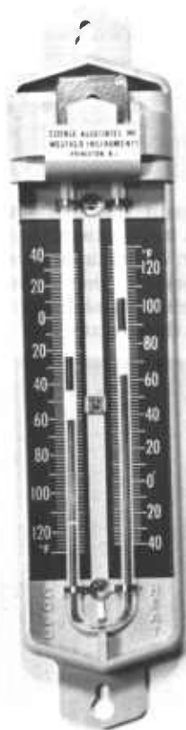
Figure 16.4.— Combined maximum-minimum thermometer; Left, Assembled; right: A, mounting plate; B, thermometer retaining screws and strip; C, thermometer tube; D, magnet.
