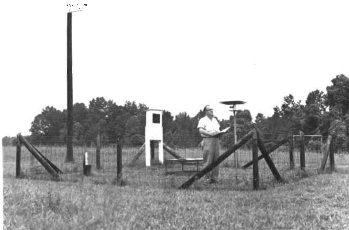
Figure 11.12. — Reading mortarboard psychrometer.
