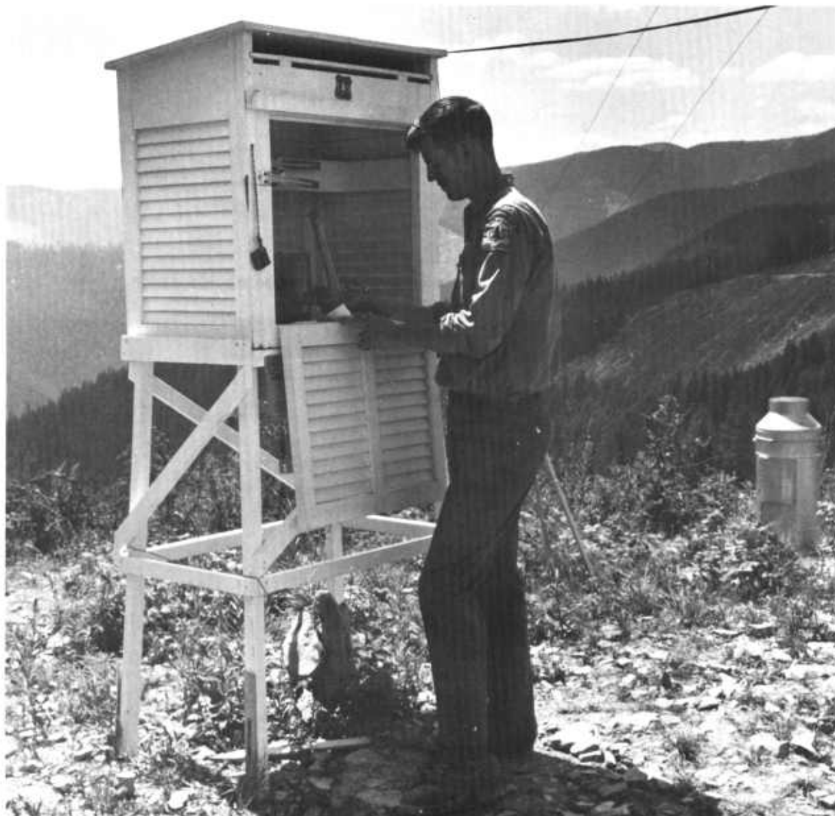
Figure 1.4. — Cotton region type instrument shelter. This standard design is recommended at all fire-weather stations.
