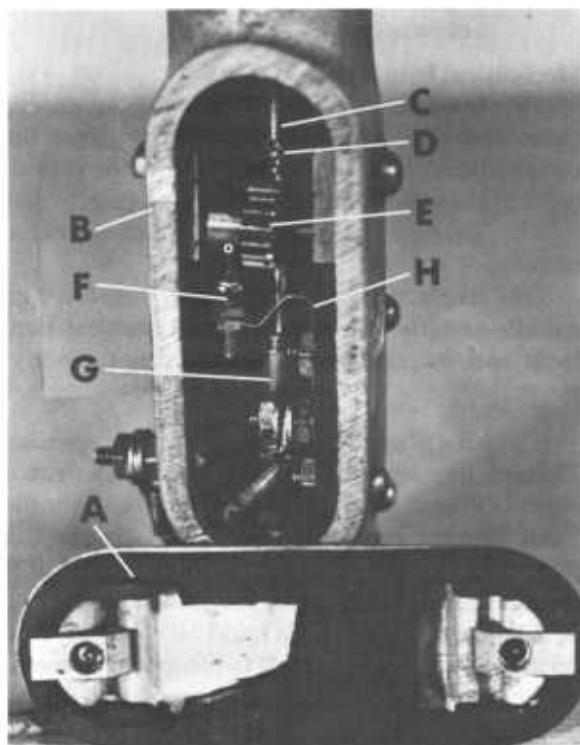
Figure 19.8. — Stewart 4-cup anemometer: A, Cover plate; B, housing; C, shaft; D, worm gear; E, pinion gear; F, contact points; G, lower thrust bearing; H, contact leaf spring.
