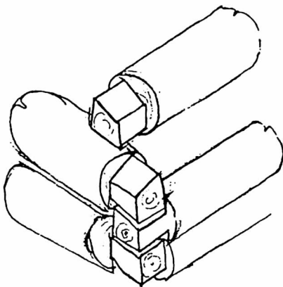
HALF DOVETAIL (Phase II)
