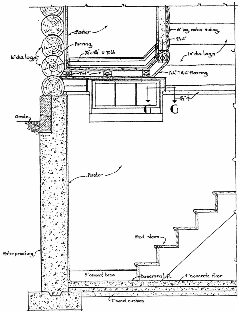
SECTION THRU STAIR Scale \frac{3}{4}" = 1'-0"
