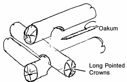
SADDLE (Phase III)
