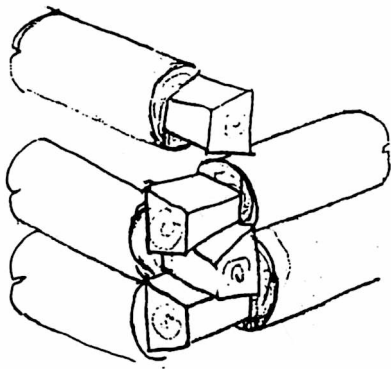
FULL DOVETAIL (Phase I)
