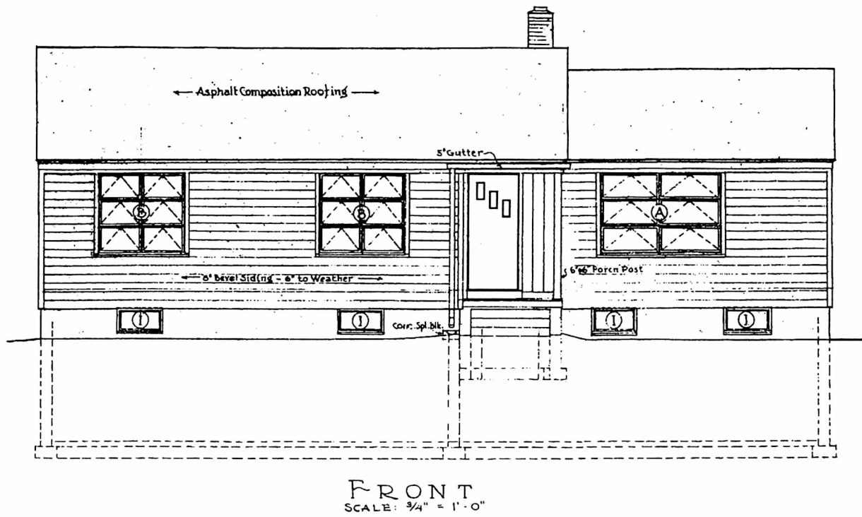
Figure 39. Building Plan, Standard Ranger's Dwelling. Three Bedroom Dwelling plan.
