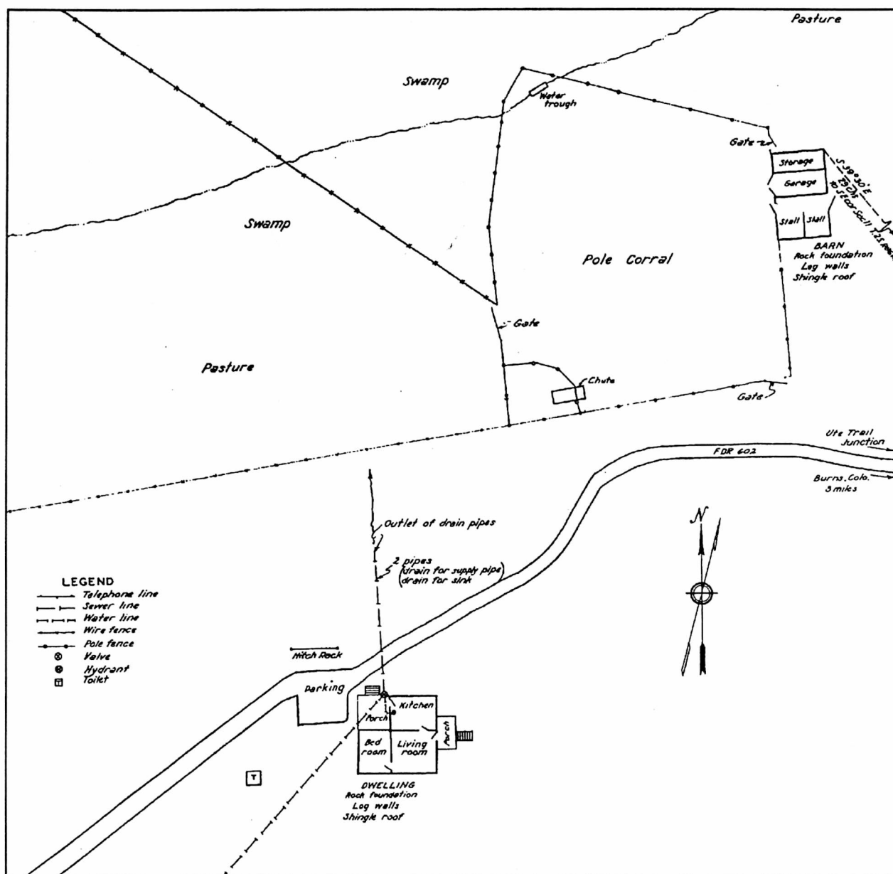
Figure 14. Site Plan, Derby Ranger Station.
