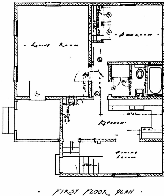
Figure 10. Building Plan and Elevation, Plan # 3, Ranger's Dwelling. Glade Ranger Station Dwelling.
