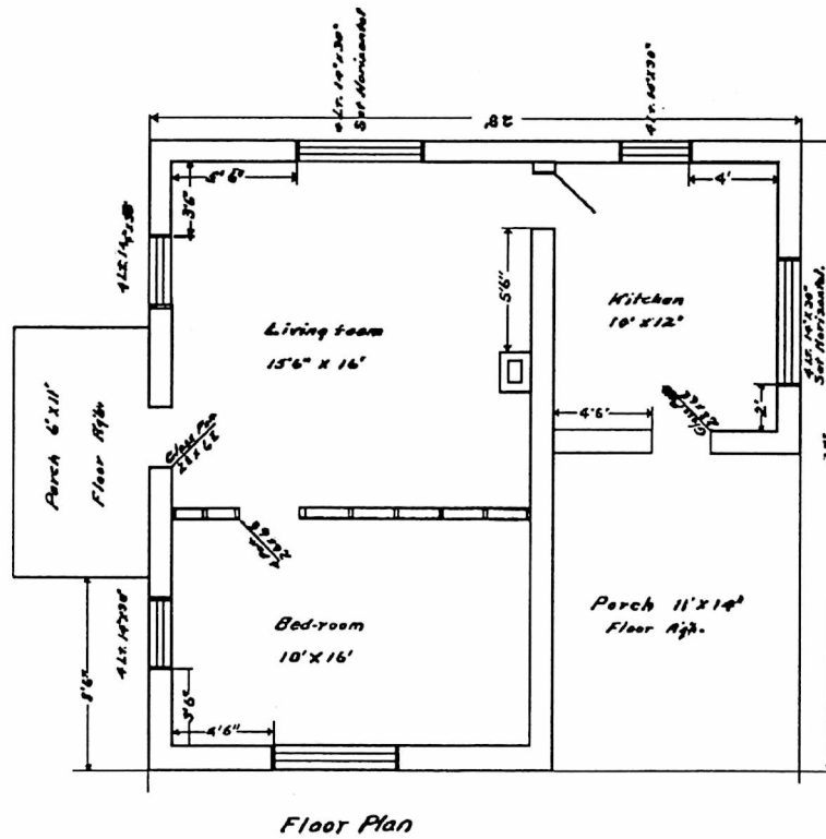
Figure 12. Building Plan and Elevation, Derby Ranger Station Dwelling.
