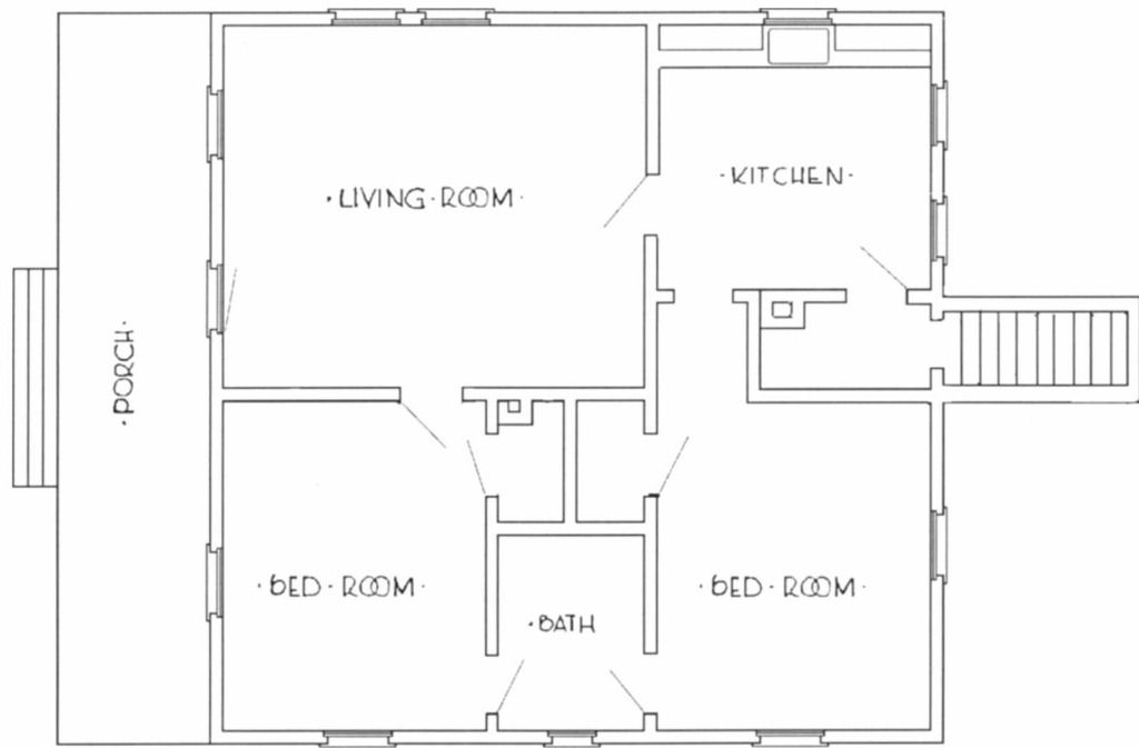
Figure 18. Building Plan, Pyramid Ranger Station Dwelling.
