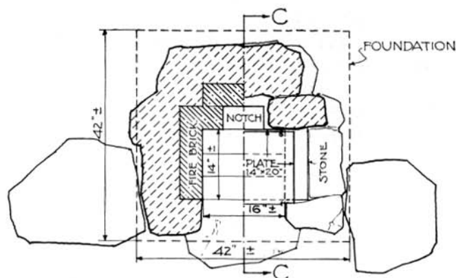
1/2 PLAN "A" 1/2 PLAN "B" FIG 5
