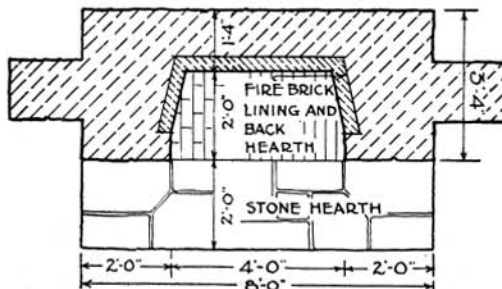
PLAN - FIG.4
