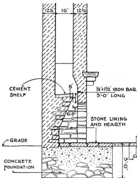
SECTION-FIG. 2
