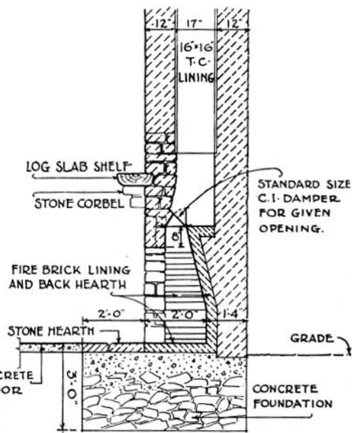
SECTION-FIG. 3
