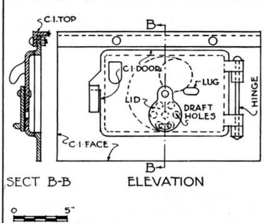
FIG. 4 CAST IRON STOVE DETAILS
