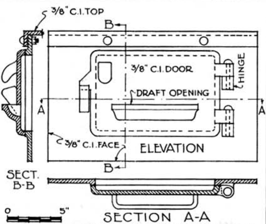
FIG. 3 CAST IRON STOVE DETAILS
