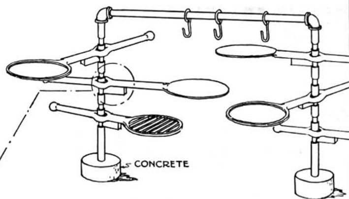
FIG. 1 COOKING STANDARD FOR CAMPFIRE USE
