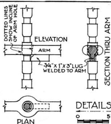
FIG. 1 COOKING STANDARD FOR CAMPFIRE USE
