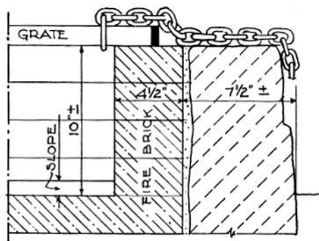
FIRE BOX DETAIL, SECT. 4 1/2" SIDE LINING, CHAINED GRATE.
