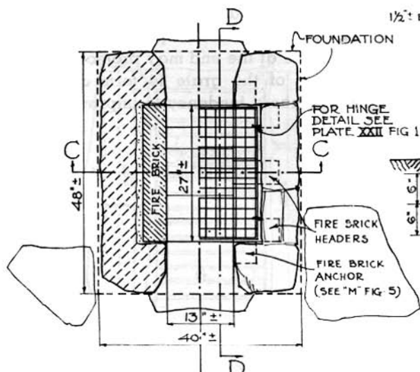
1/2 PLAN "A" 1/2 PLAN "B" FIG. 4
