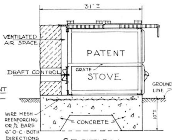
SECTION FIG 4
