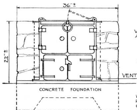
ELEVATION FIG 3
