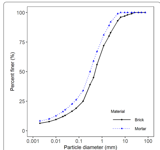
Fig. 2 Block and mortar particle size distributions, methods ASTM D 6913-17 and ASTM C136-14 [44, 45]
