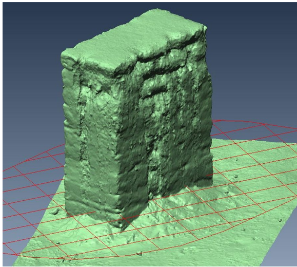
Fig. 5 Example of the three-dimensional mesh of an adobe test wall and exclusion plane
