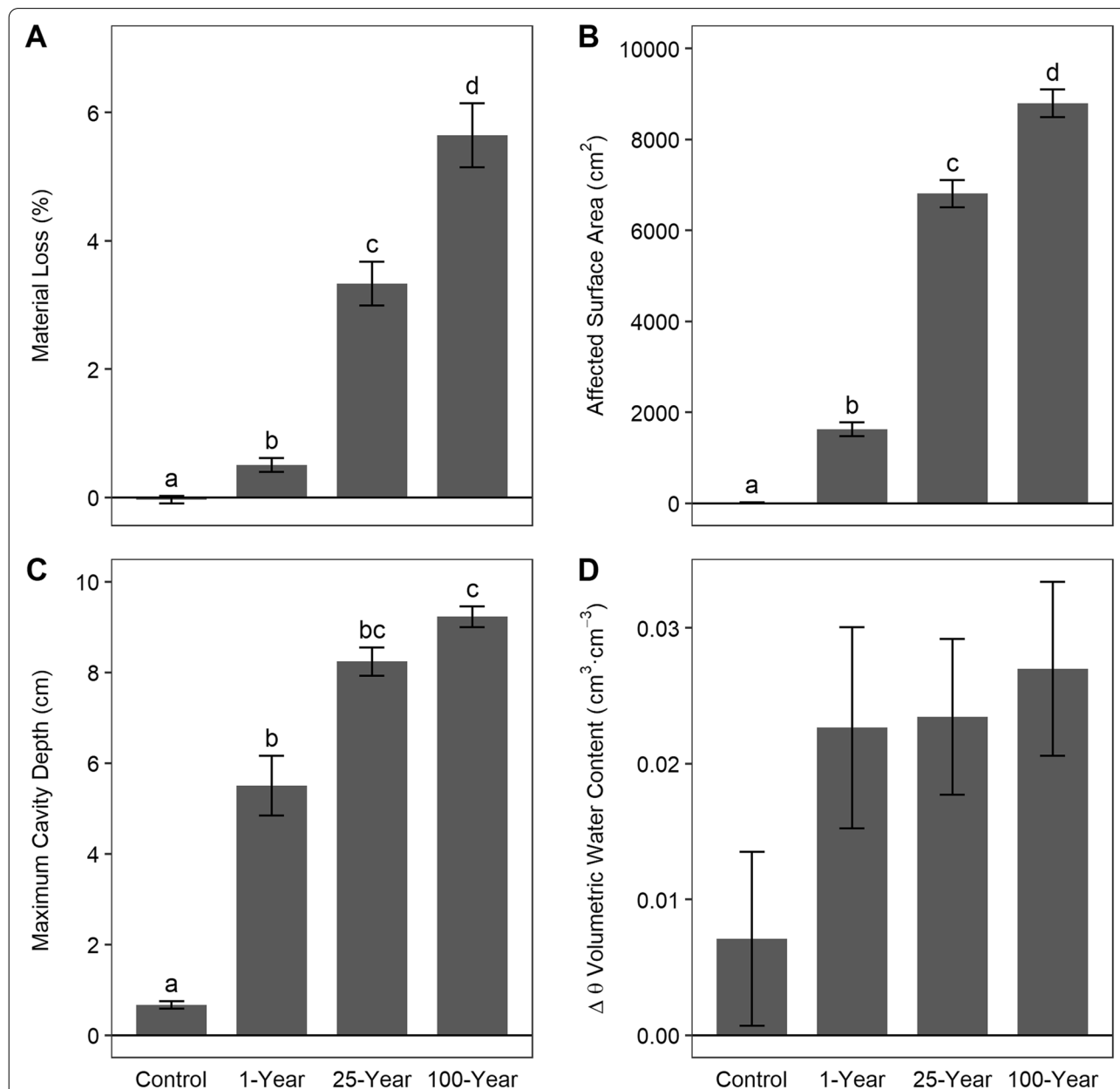
Fig. 6 Estimated marginal mean ( \pm SE) for erosion and moisture metrics by high intensity rainfall treatments. Lowercase letters across treatments within a metric (A–C) indicate statistically different groups based on post-hoc pairwise comparisons, Dunnnett t3 method ( p \leq 0.05 ) for material loss, affected surface area and cavity depth; Tukey method ( p \leq 0.05 ) for net change of volumetric water content
