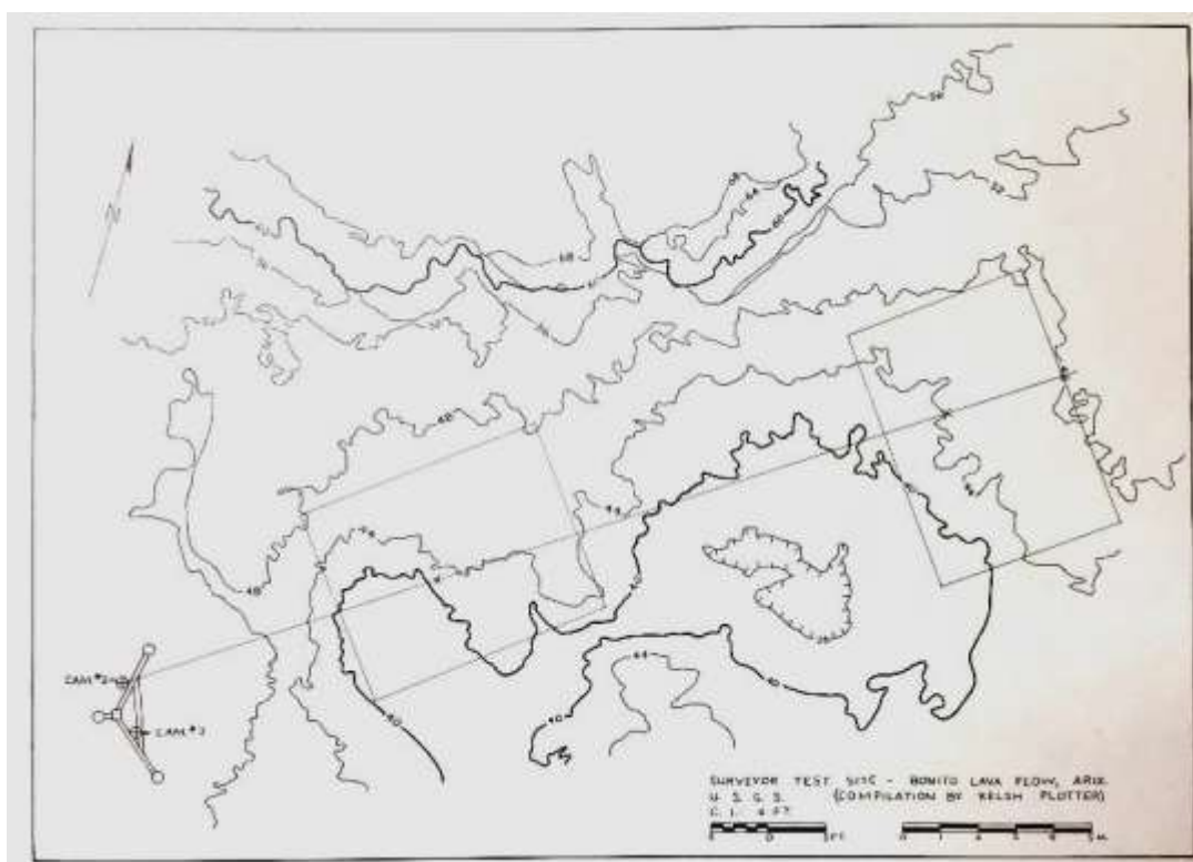
Fig. 68. Map of the Surveyor camera test site on the Bonito Lava Flow. (Uncatalogued USGS Image, USGS Astrogeology Regional Planetary Information Facility, USGS Astrogeology Science Center, Flagstaff, Arizona.)
