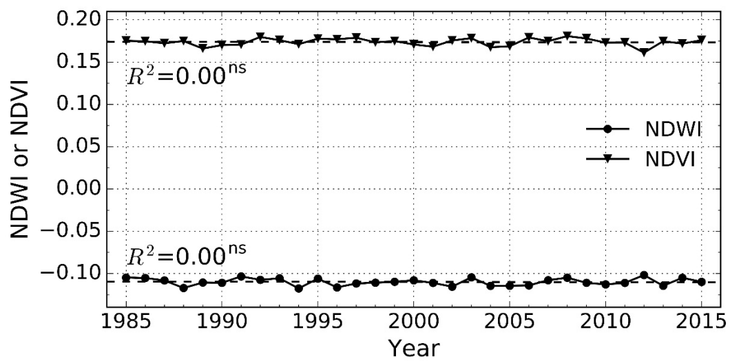
Figure S4. Trends over time of NDWI and NDVI of five randomly selected time-invariant objects (water bodies or bare rock areas).
