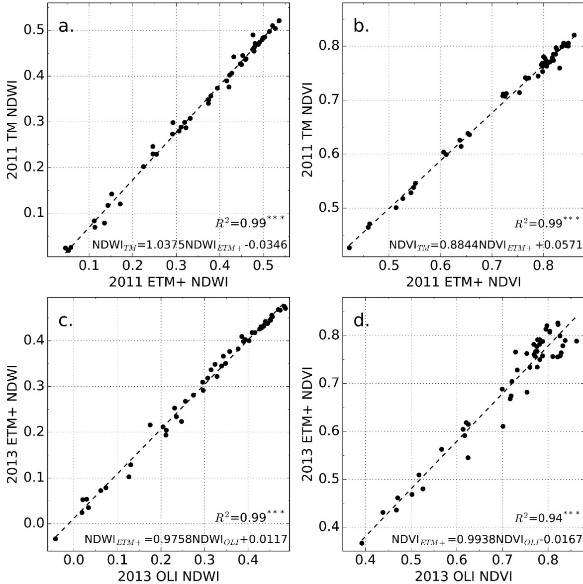
Figure S3. Comparisons of (a) 2011 Landsat 7 ETM+ NDWI and 2011 Landsat 5 TM NDWI, (b) 2011 Landsat 7 ETM+ NDVI and 2011 Landsat 5 TM NDVI, (c) 2013 Landsat 8 OLI NDWI and 2013 Landsat 7 ETM+ NDWI, and (d) 2013 Landsat 8 OLI NDVI and 2013 Landsat 7 ETM+ NDVI at the 50 selected reference sites.
