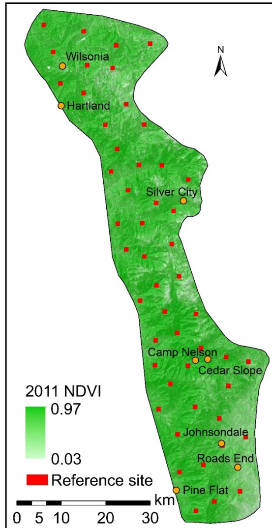
Figure S2. The distribution of the selected 1 km 2 reference sites used for homogenizing the three Landsat sensors (i.e., TM, ETM+, and OLI). The background NDVI is derived from the 2011 Landsat 5 TM data.
