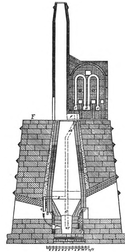
19th Century Furnace of Ashlar with Air Blast Preheat
