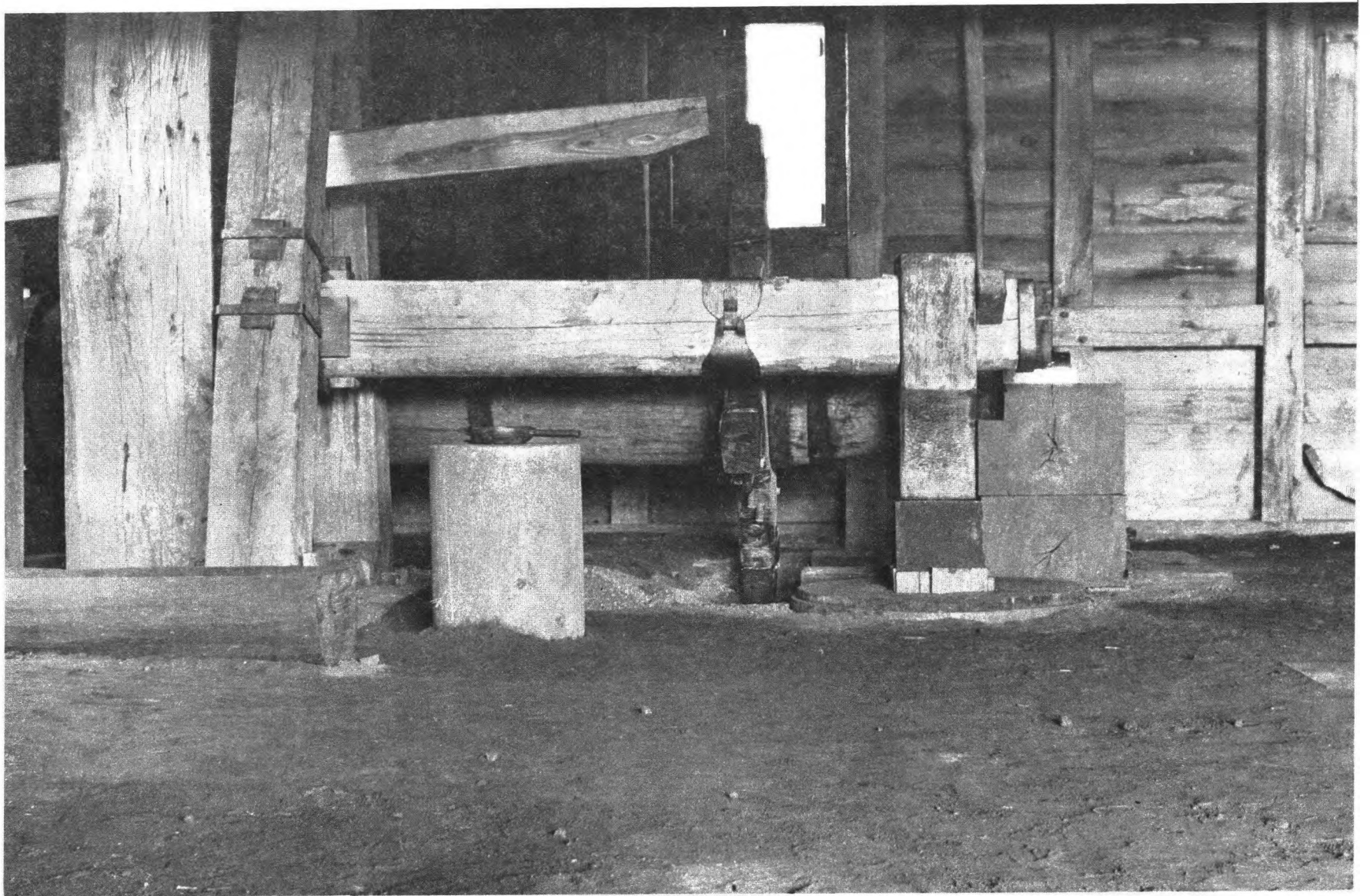
THE FORGE HAMMER
