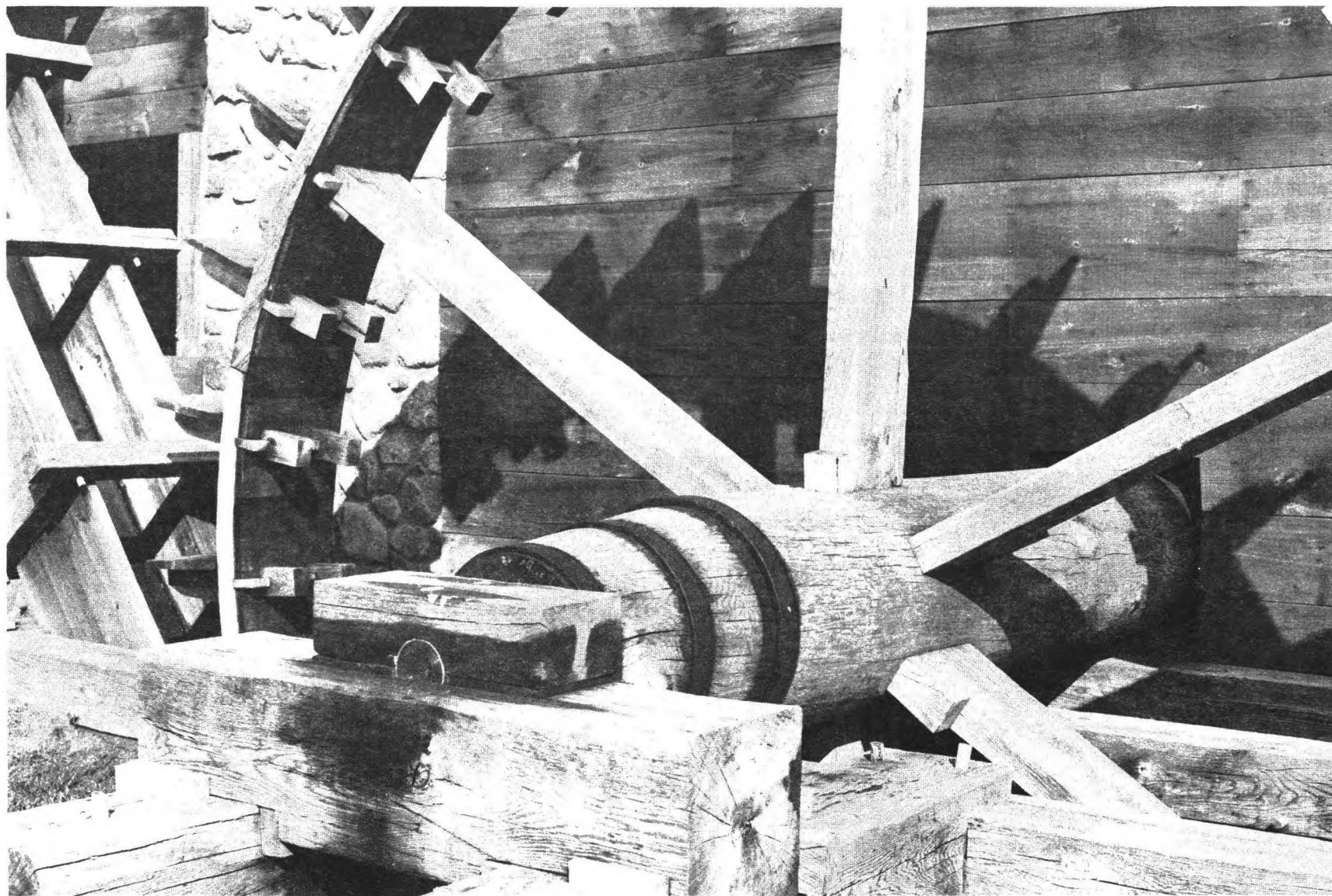
DETAIL OF WATERWHEEL
