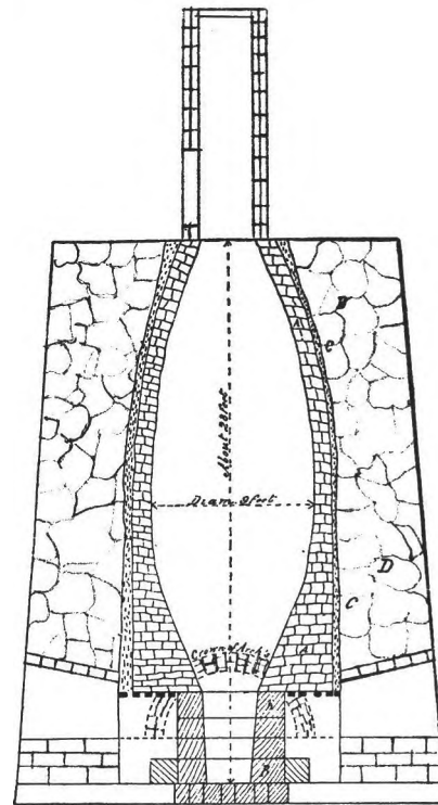
17th Century Furnace of Fieldstone
