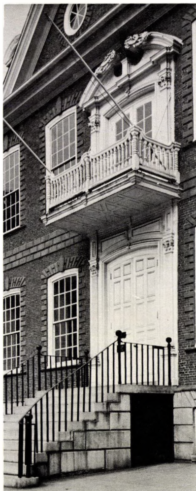
Colony House, Balcony, showing carved pediment and twisted balusters. Meservey photo.
