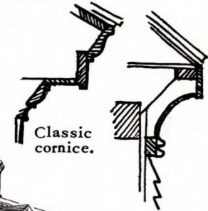
Plaster cove cornice.
