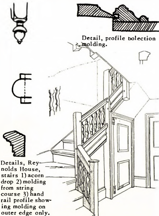
Stairway, about 1720, showing flat balusters sawn to S shape. 3 run plan, closed string course.
