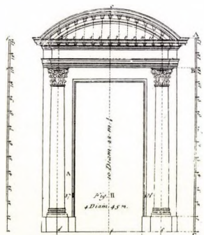
Model for Russell House door from Battey Langley.
