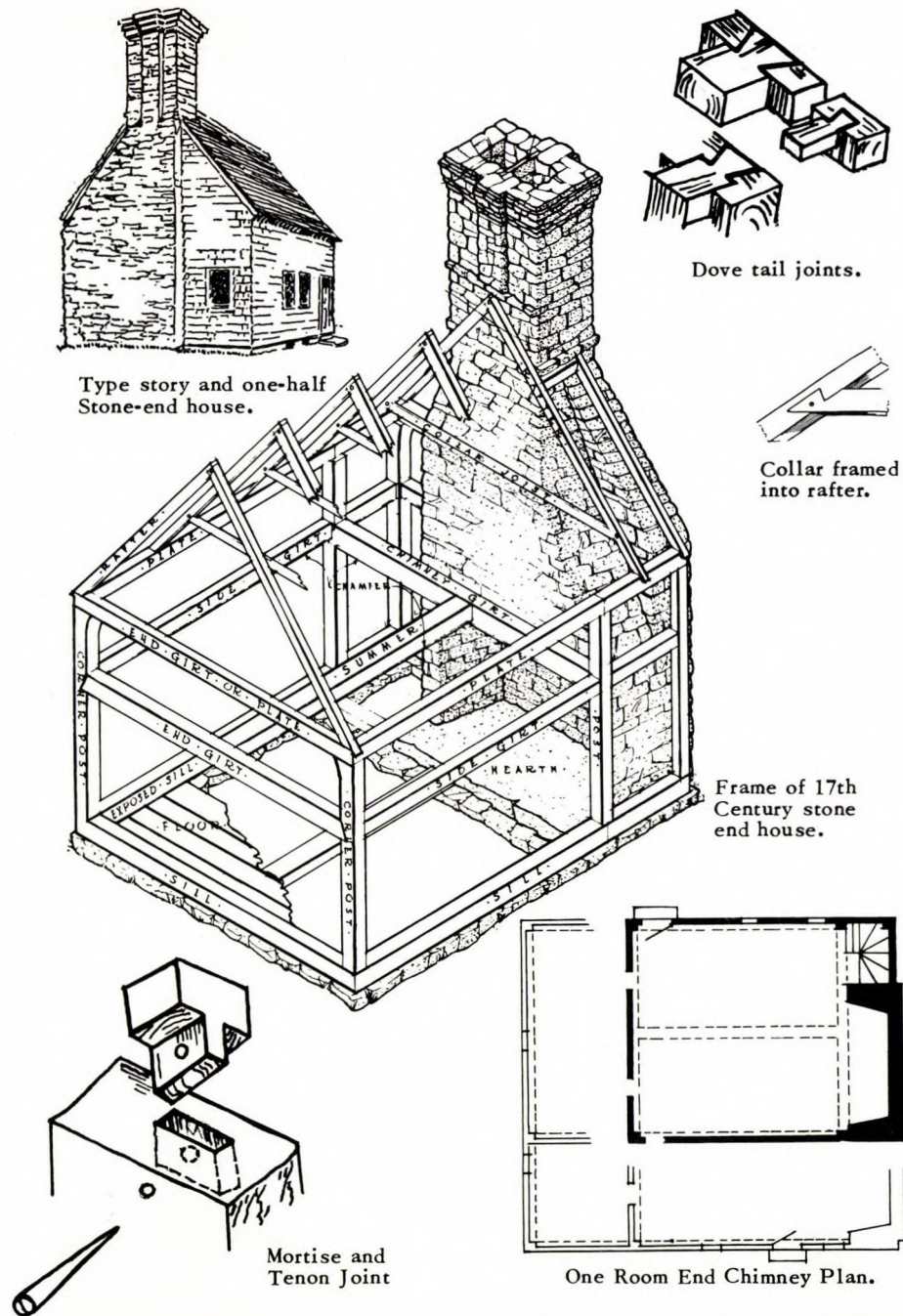
Seventeenth Century one and a half story end chimney house frame, typical one room end chimney plan, and framing details. Studs were not often used in Northern Rhode Island houses. Wide Vertical Boards, nailed to sills, girts and plates formed the walls. Hand split, feathered and ship lapped clapboards or hand split shingles were nailed to these boards.
