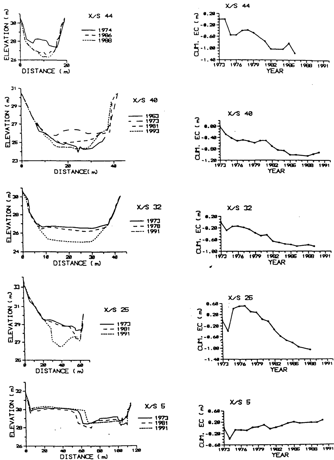
Figure 4 Graph showing selected channel cross-section surveys, Redwood Creek
