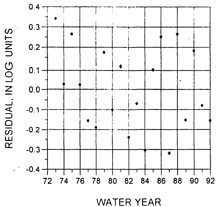
Figure 6 Graph showing suspended-sediment residuals for Redwood Creek at Orick, 1971-92 (A) and Redwood Creek at O'Kane, 1973-92.
