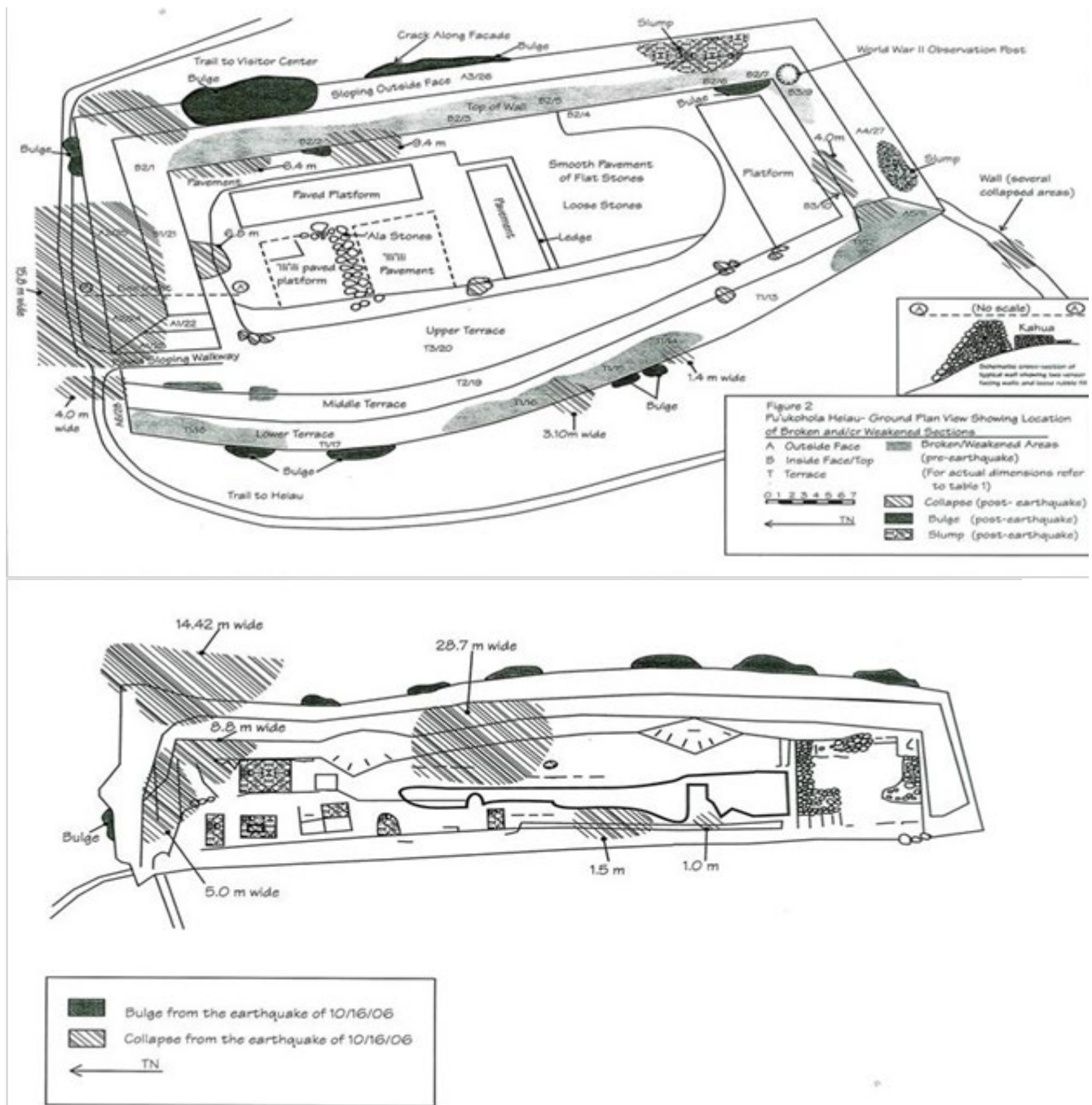
Figure 38. Plan maps of Pu'ukohola Heiau (top) and Mailekini Heiau (bottom) showing areas damaged by the 2006 earthquakes. Maps courtesy of NPS.
