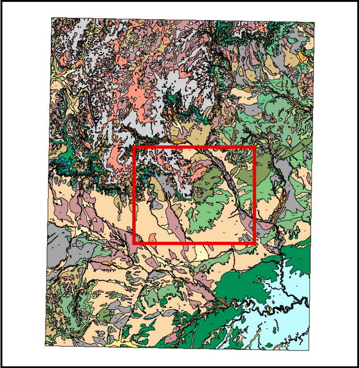
Full Extent of Digital Geologic Data, Area of Detail in Red
