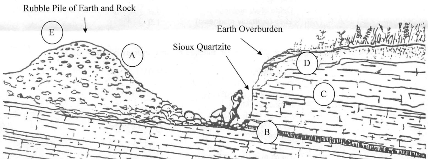
Pencil sketch showing geologic cross section of quarry, pipestone is the dark stratum near the bottom of the quarry
