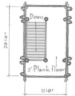
TOP PLAN
