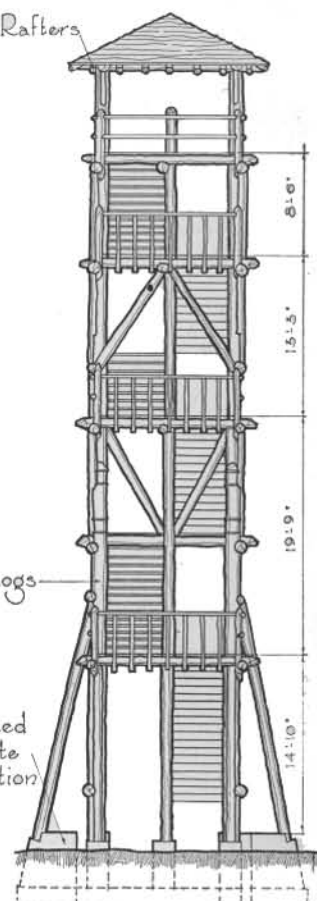
SIDE ELEVATION - FRONT ELEVATION - SIDE ELEVATION - REAR ELEVATION
