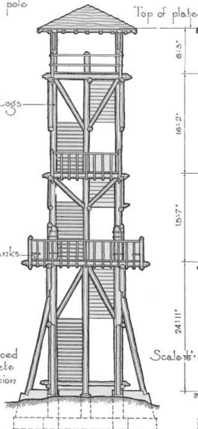
SIDE ELEVATION - FRONT ELEVATION - SIDE ELEVATION - REAR ELEVATION
