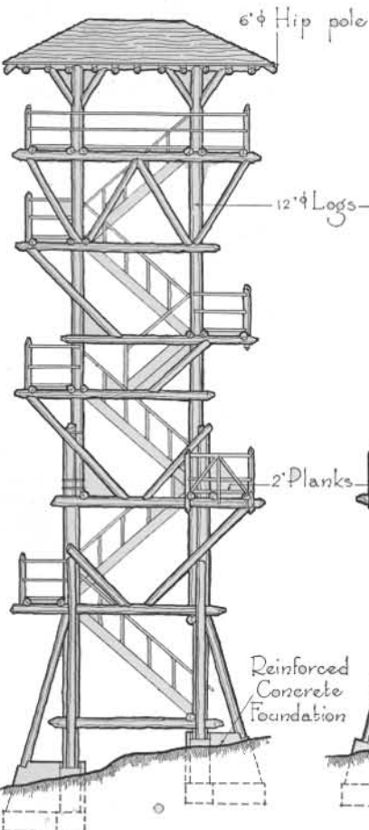
SIDE ELEVATION - FRONT ELEVATION - SIDE ELEVATION - REAR ELEVATION
