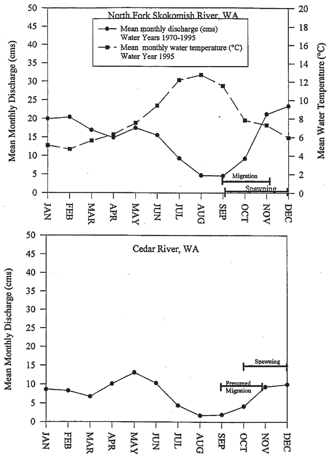
Figure 27. Comparison of mean monthly discharge (cms) in N. Fk. Skokomish River (WY 1970-1995; circle) and Cedar River (WY 1945-1992) WA in relation to bull trout migration and spawning. N. Fk. Skokomish River temperature (WY1995; square) denoted. Data from unpublished USGS files.
