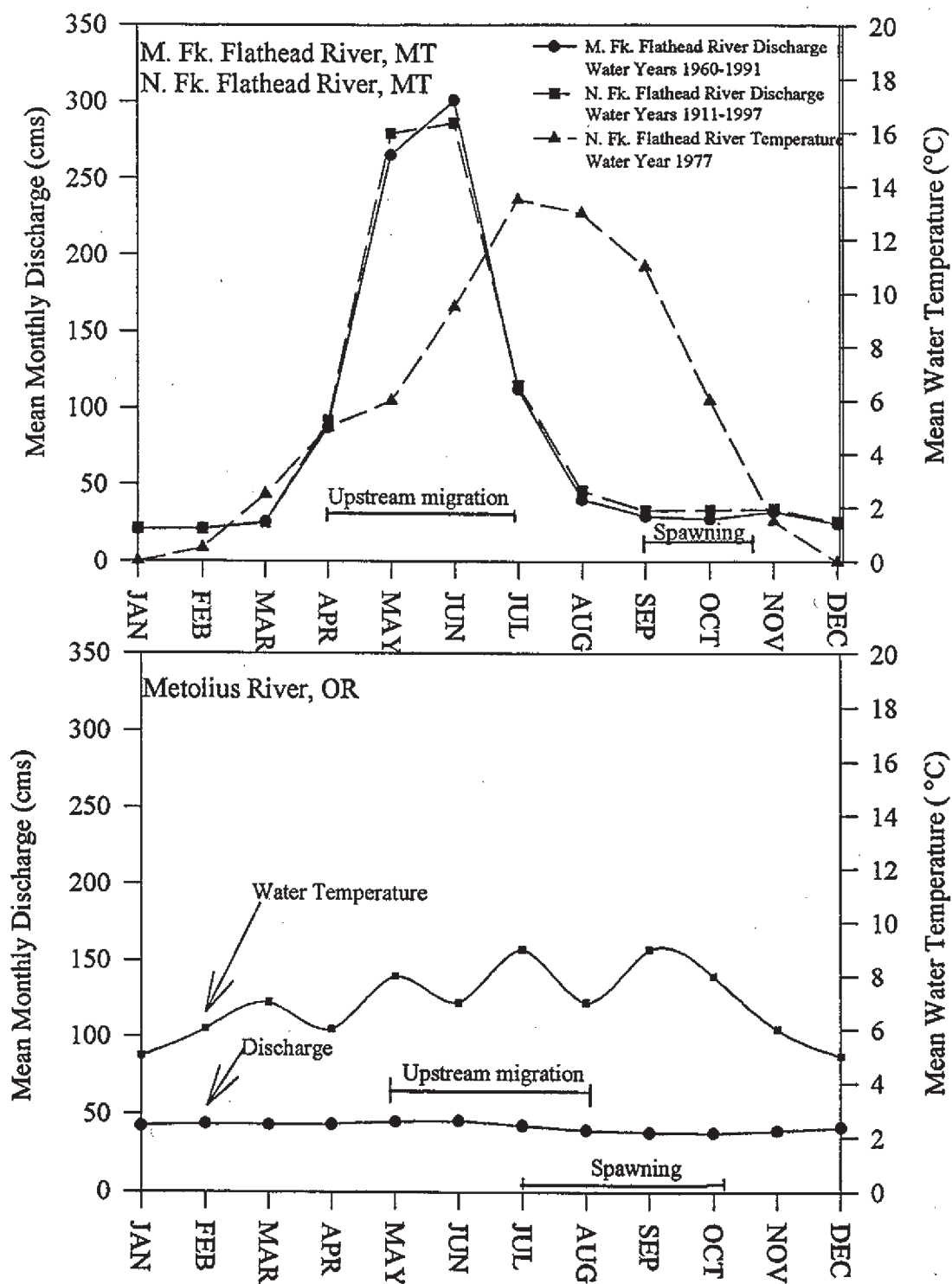
Figure 25. Mean monthly discharges (cms) and water temperature (°C) in M. Fk. (WY 1960-1991) and N. Fk. (WY 1911-1997) Flathead Rivers, MT and Metolius River (WY 1913-1995), OR in relation to bull trout migration and spawning. Metolius River temperature (Scott Lewis, personal communication, Portland General Electric).
