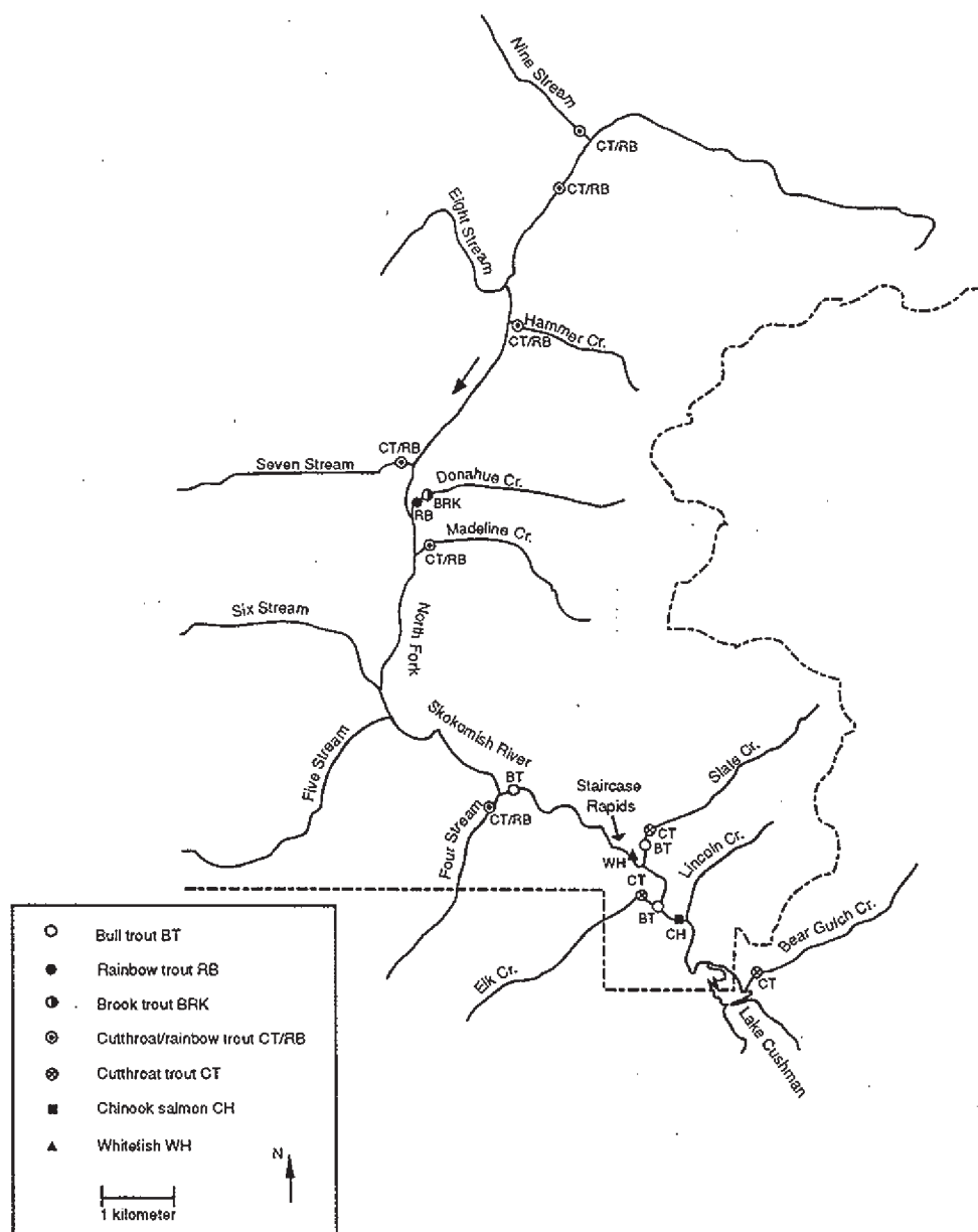
Figure 6. Uppermost distributions of salmonids in North Fork Skokomish River Basin as determined by day snorkel surveys and electrofishing.
