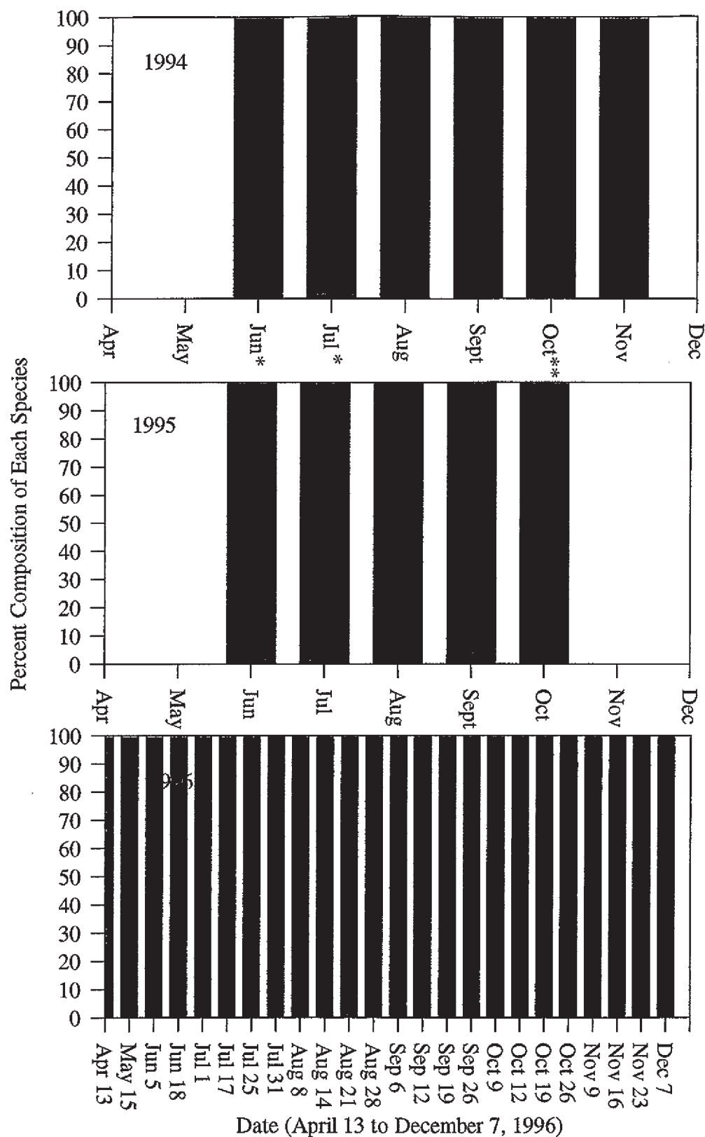
Figure 23. Percent composition of adult bull trout (black), adult whitefish (green), and cutthroat/rainbow trout (red) in the N. Fk. Skokomish River sections 2 to 5 from 1994 to 1996.*river sections 2-4**WDFW 2-6. Based on counts from day snorkel surveys.
