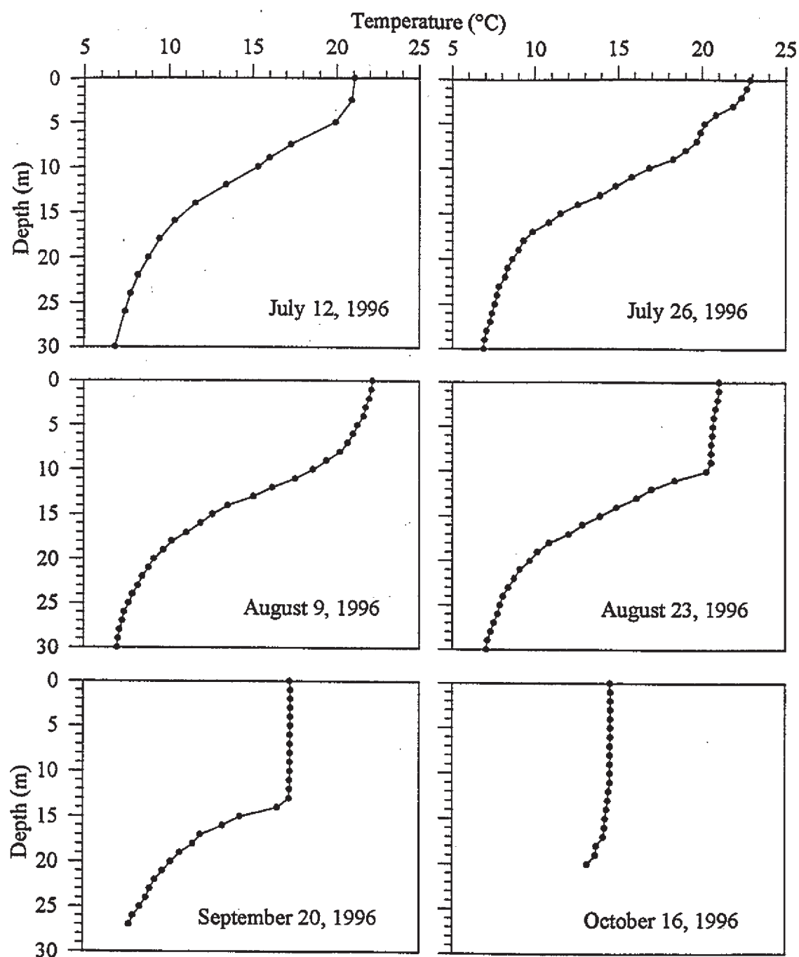
Figure 21. Mean water temperature (°C) as a function of depth (m) in Lake Cushman from July 12 to October 16, 1996. Values averaged for limnological stations one and two.
