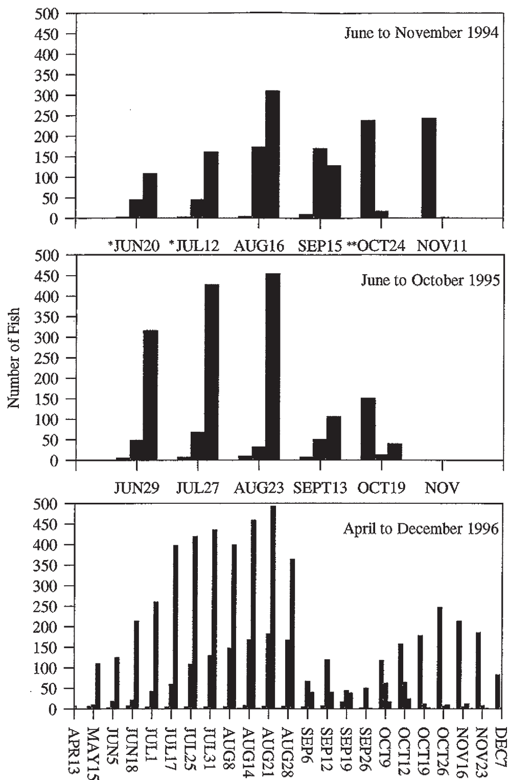
Figure 22. Temporal shifts in abundances of adult bull trout (black), adult whitefish (green), and cutthroat/rainbow trout (red) in N. Fk. Skokomish River sections 2-5 from 1994 to 1996. Based on day snorkel counts of each species. *river sections 2-4 **WDFW sections 2-6.
