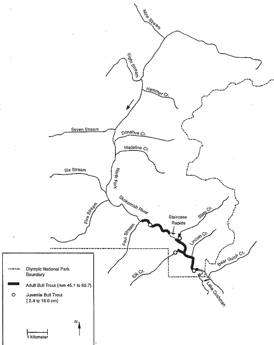
Figure 5. Distribution of adult (—) and juvenile (○) bull trout in the North Fork Skokomish River Basin, Olympic National Park in 1996.
