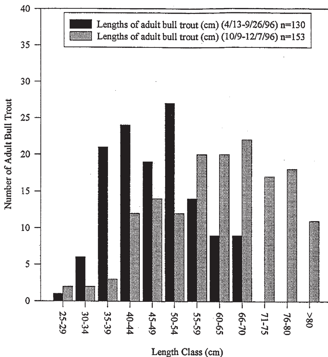
Figure 10. Length distributions (cm) of early (4/13/96-9/26/96; n=130) and late (10/9/96-12/7/96; n=153) migrating adult bull trout. Based on length estimates from total number of observations during day snorkel surveys in North Fork Skokomish River.
