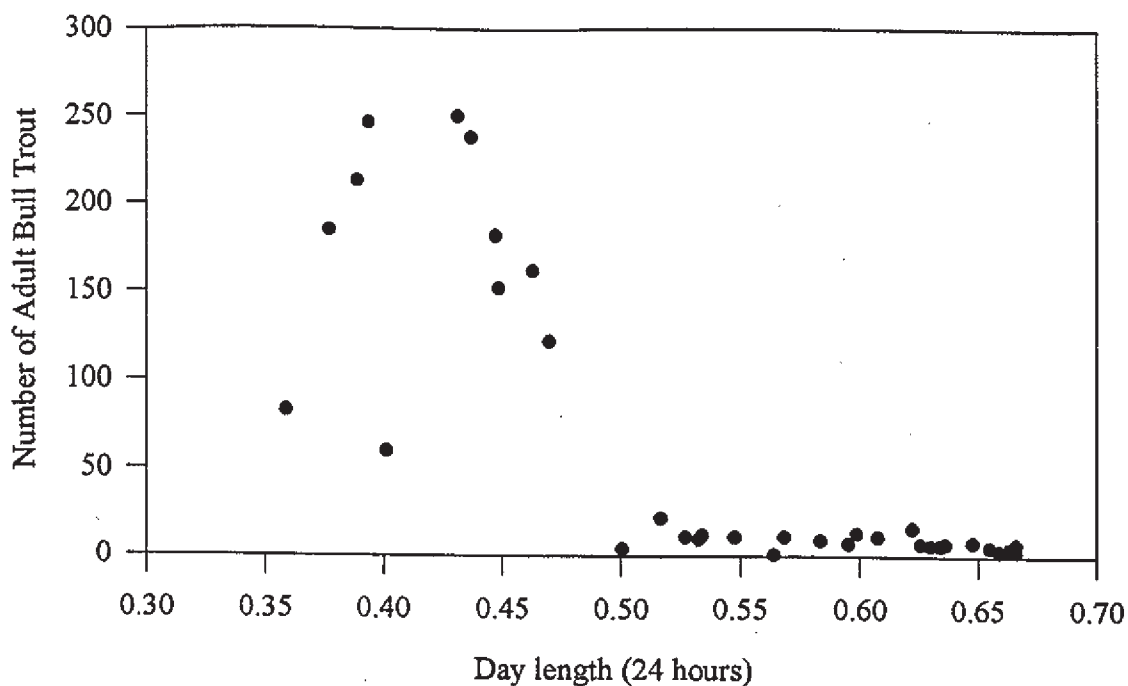
Figure 13. Relationship between number of adult bull trout and day length in the North Fork Skokomish River ( 47^{\circ} 30' N ). Based on number of adult bull trout observed during snorkel counts from 1994 to 1996.
