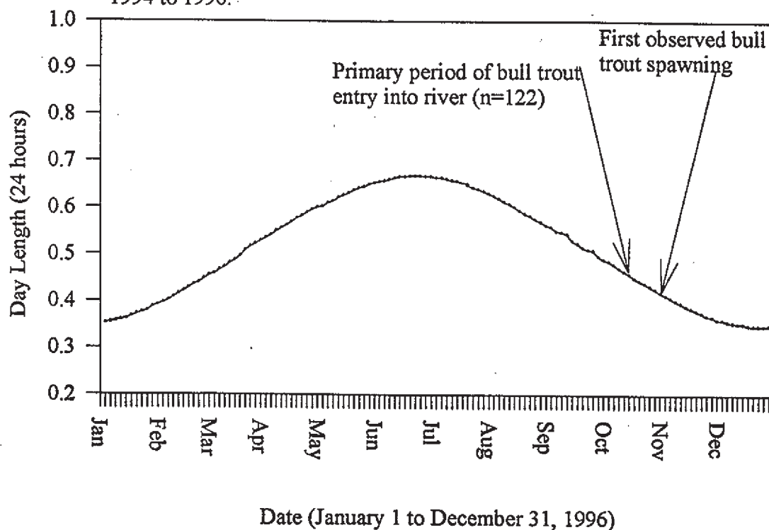
Figure 14. Day length at 47^{\circ} 30' N latitude (North Fork Skokomish River) from January 1 to December 31, 1996. Timing of bull trout migration and first observed spawning denoted.
