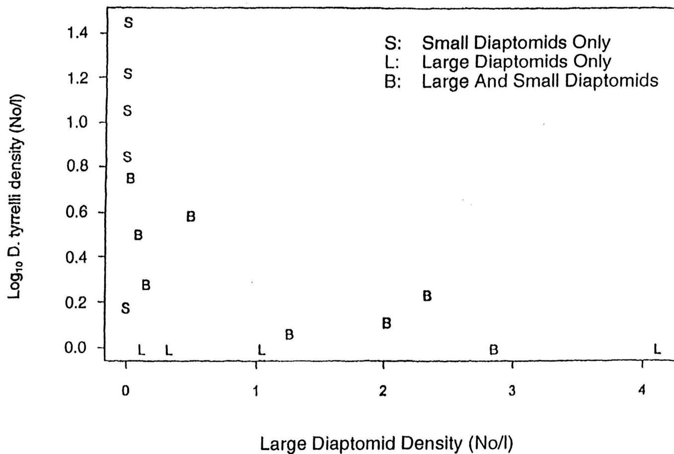
Figure 4.3. Relationship between Diaptomus tyrrelli density and density of large diaptomids ( D. kenai and D. arcticus ) for lakes with \text{TKN} \geq 0.05 \text{ mg l}^{-1} and \text{TP} \geq 0.007 \text{ mg l}^{-1} .
