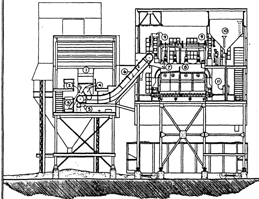
SECTION B-B THROUGH MAIN SCREENING ROOM AND COAL WASHING ROOM (LOOKING EAST)
