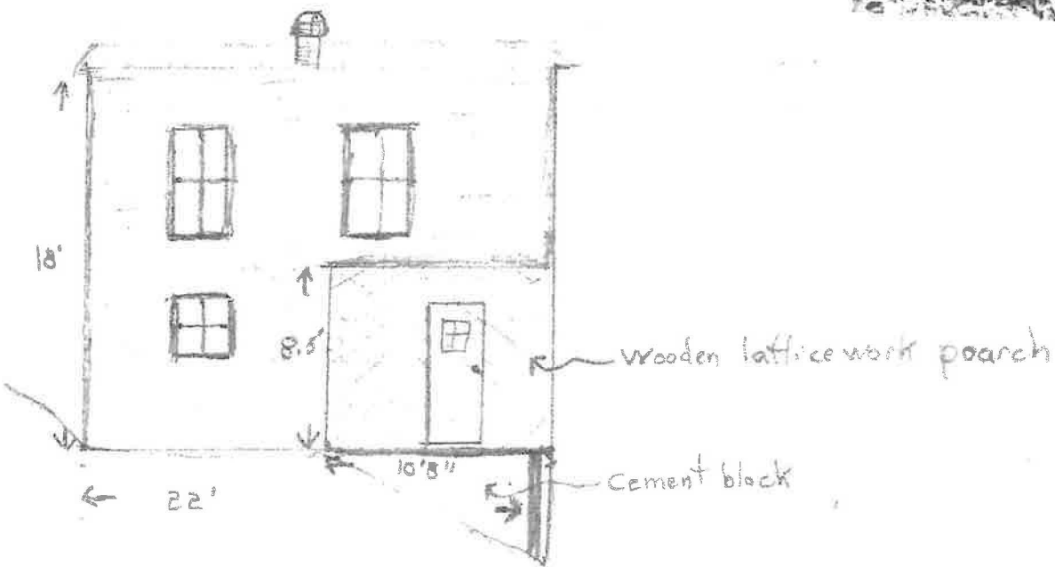
Scale \frac{1}{8}" = 1' Pugh House W. Facade, Thurmond, WV, Summer 1989
