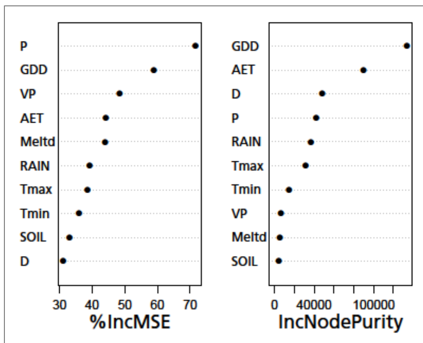
Figure 22. Variable importance in the random-forest model of climate drivers of the start of growing season. Percent increase in mean square error (%IncMSE) is a measure of model performance with each variable. Increase in node purity (IncNodePurity) is the difference in residual sum of squares in regression with or without each variable.
