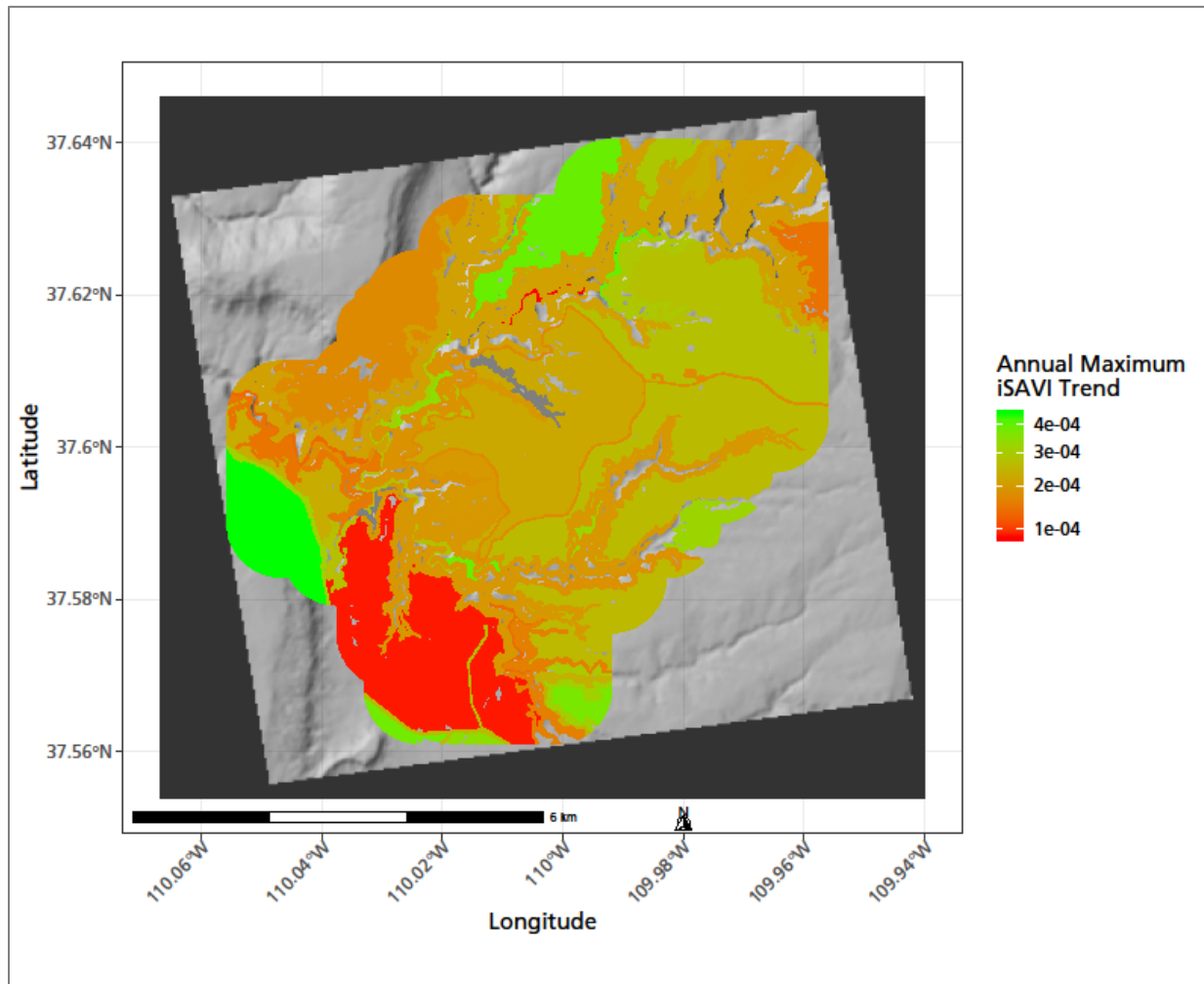
Figure 27. Spatial pattern of trends in maximum annual iSAVI. Trend is average change in iSAVI per year for the period 2000–2019.
