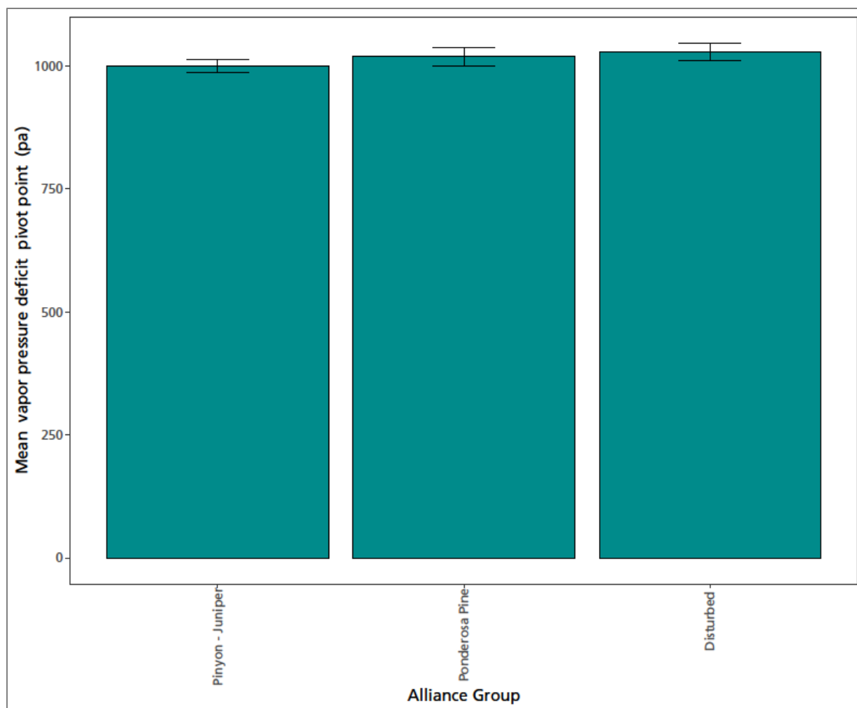
Figure 46. Pivot points for polygons in Natural Bridges National Monument where vapor pressure deficit was significantly related to interannual variation in production (p-value < 0.05). Climate data summarized by water year.
