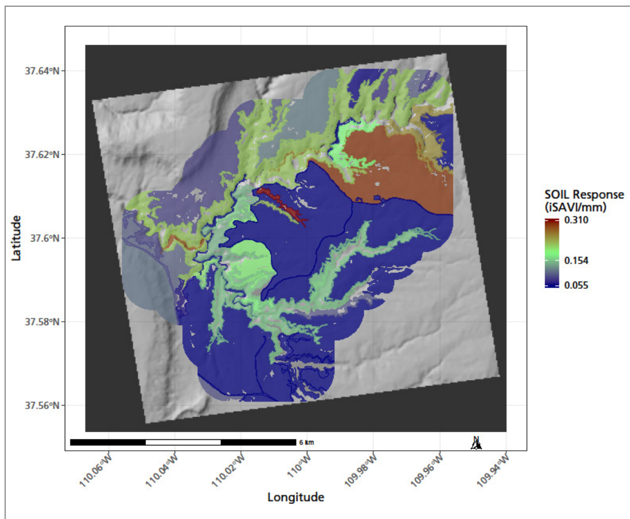
Figure 51. Sensitivity of growing season vegetation production to soil moisture, where the relationship was significant ( p -value < 0.05 ). Climate data summarized by water year.
