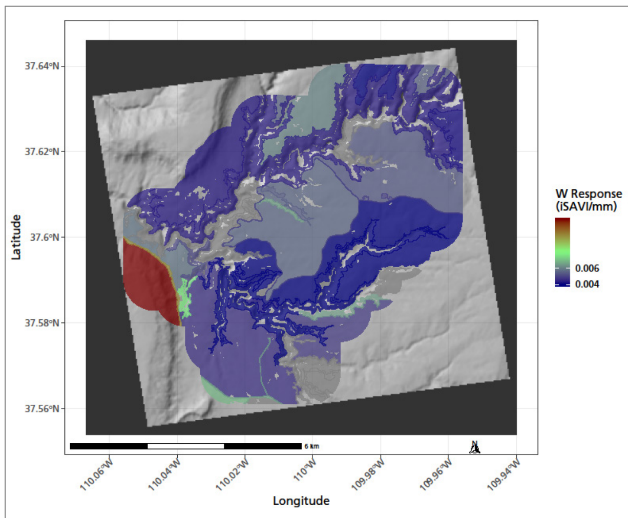
Figure 61. Sensitivity of growing season vegetation production to rain plus snowmelt where the relationship was significant ( p -value < 0.05). Climate data summarized by water year.
