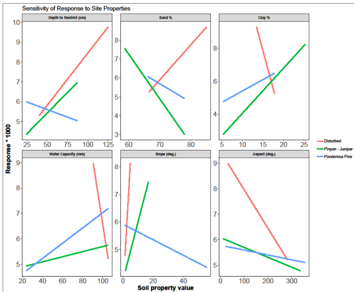
Figure 65. Variation in responses to precipitation as related to soil and site characteristics. Steeper slopes indicate greater sensitivity of responses to site properties. These site properties are important modifiers of climate because they control water retention and distribution in the soil profile and, in the case of site slope and aspect, because they affect the heat load on vegetation.
