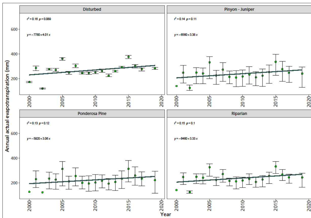
Figure 73. Cumulative annual actual evapotranspiration over time (2000 to 2019) in vegetation alliance groups. The trend over time is shown for the period in gray in the previous figure. Error bars are standard error.
