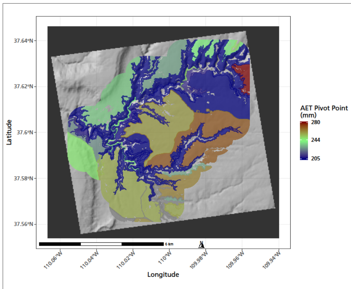
Figure 43. Pivot points for polygons where actual evapotranspiration was significantly related to interannual variation in production ( p -value < 0.05 ). Climate data summarized by water year.
