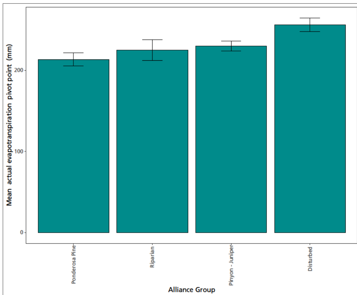
Figure 10. The mean actual evapotranspiration pivot-point values shown here represent critical water needs for the different alliance groups. Standard error bars indicate range in variability of pivot points among polygons of an alliance group if more than one polygon had a statistically significant relationship ( p -value < 0.05) with precipitation. Pivot points identify the critical water need that achieves average production for each alliance group.
