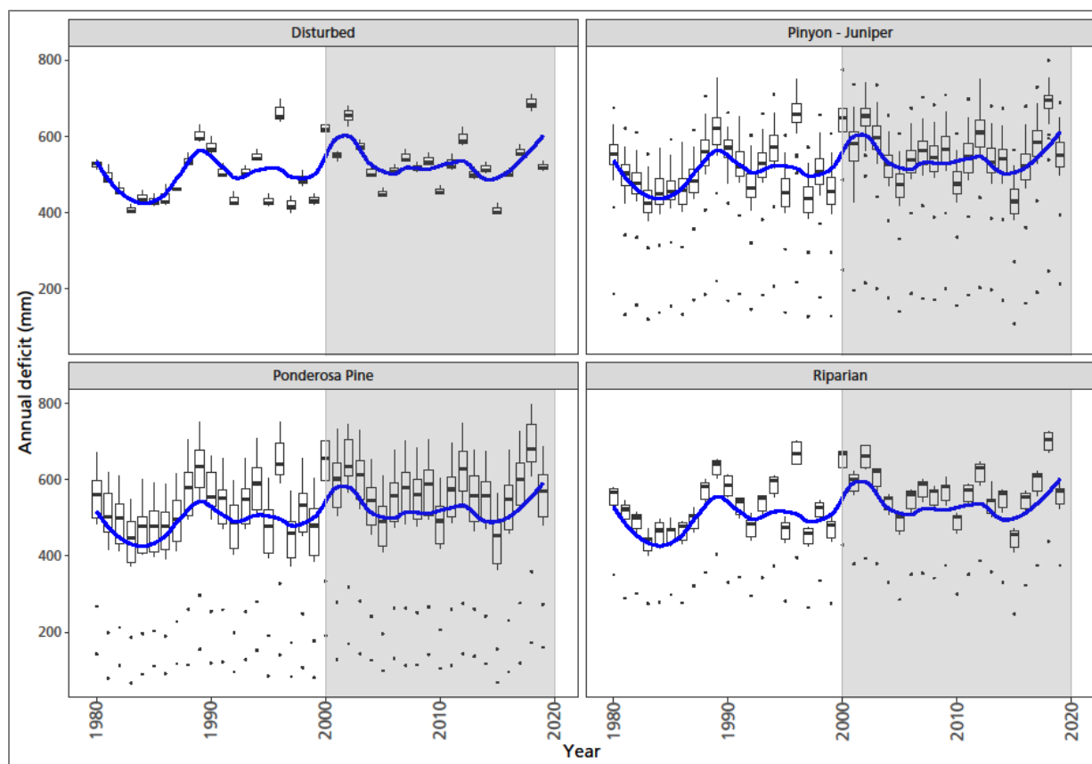
Figure 74. Cumulative annual water deficit over time (1980 to 2019) in vegetation alliance groups. Box plots demonstrate the range of variation within alliance groups by year. The blue line is a loess smooth with a 25 percent span to illustrate multiyear patterns. Gray shaded area includes the period investigated for relationships between production and climate when satellite imagery and climate data were both available.
