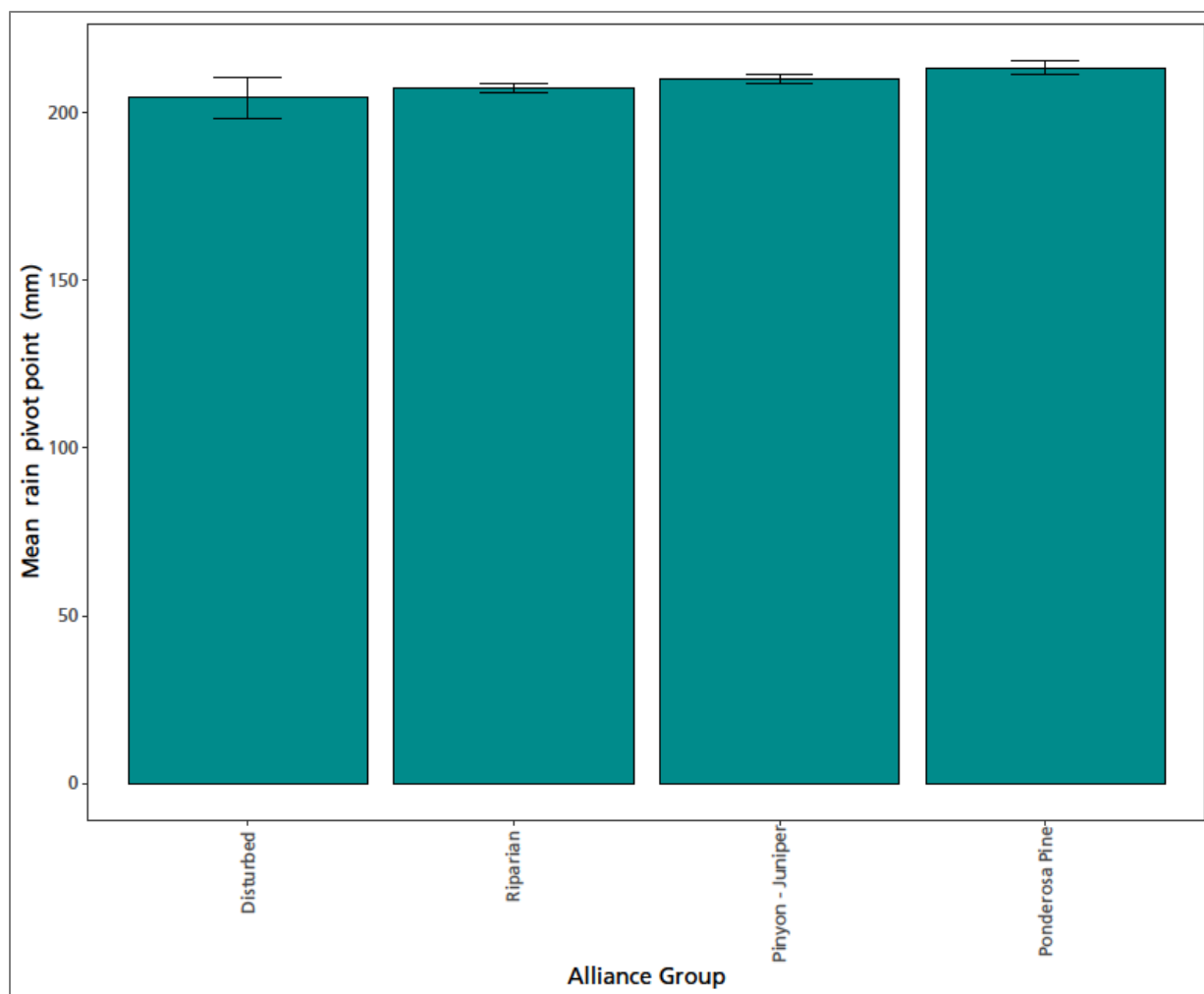
Figure 32. Pivot points for polygons in Natural Bridges National Monument where rain was significantly related to interannual variation in production ( p -value < 0.05 ). Climate data summarized by water year. NPS / DAVID THOMA
