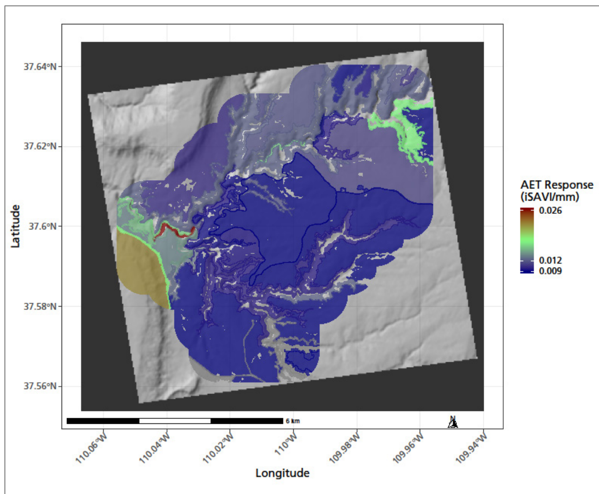
Figure 59. Sensitivity of growing season vegetation production to actual evapotranspiration where the relationship was significant ( p -value < 0.05). Climate data summarized by water year.
