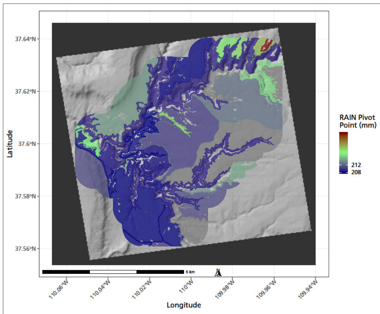
Figure 33. Pivot points for polygons where rain was significantly related to interannual variation in production ( p -value < 0.05). Climate data summarized by water year.
