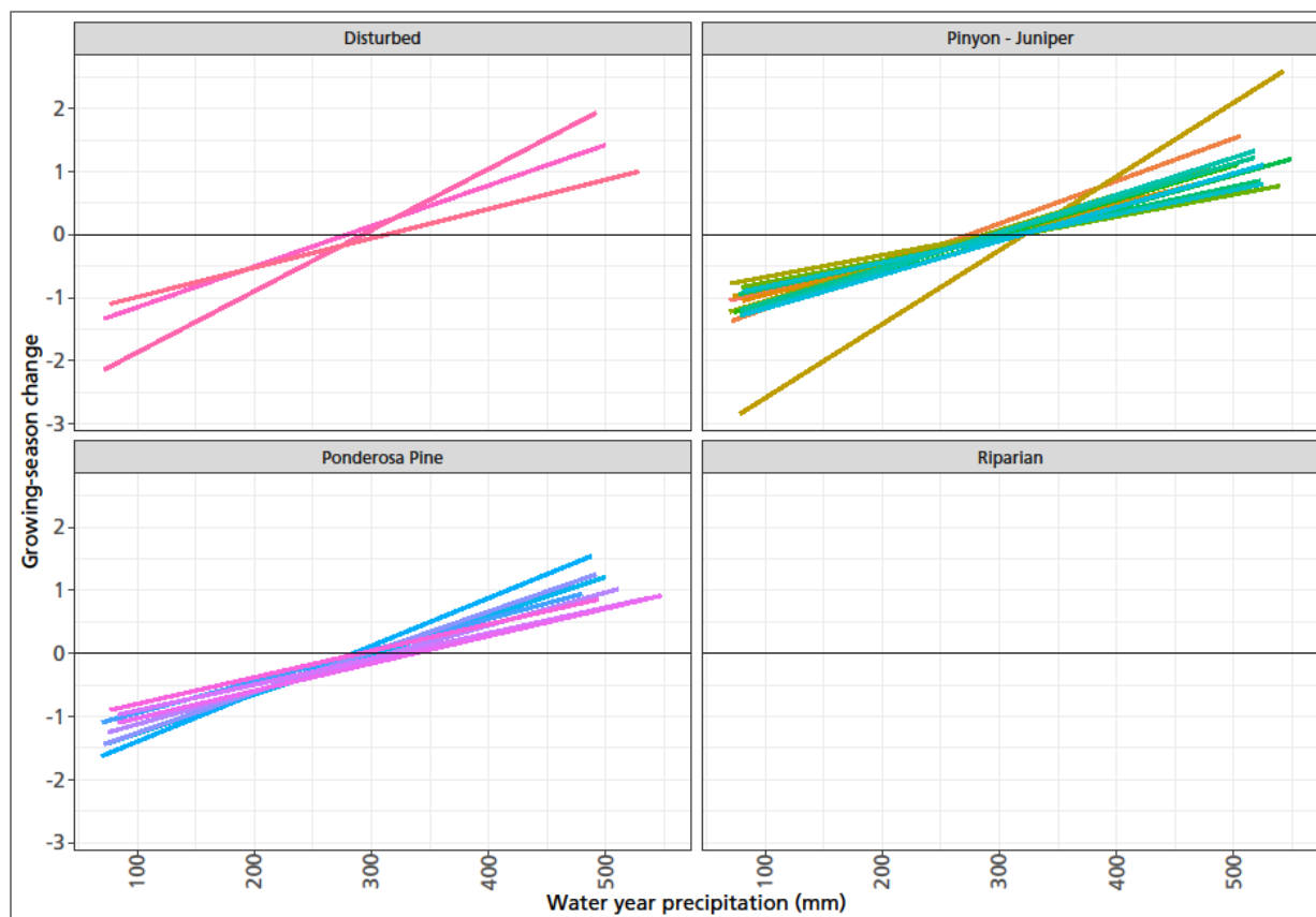
Figure 16. Graphical depiction of the relationship between pivot points and responses in polygons that had a significant relationship ( p -value < 0.05 ) between iSAVI and water-year precipitation (e.g., critical water need vs. rate of growing-season iSAVI change per mm precipitation). Polygon-level pivot points and responses are provided in Table S-2 of NPS (2025). Alliance groups with steeper slopes are considered more responsive to changes in water availability. Alliance groups and alliance polygons within alliance groups that cross the horizontal axis further left are more drought resistant, as they shift to above-average condition with less precipitation. Only significant relationships are shown. Panels without lines represent alliance groups with no significant relationships between iSAVI and climate variables. Colors help differentiate individual polygons within alliance groups.
