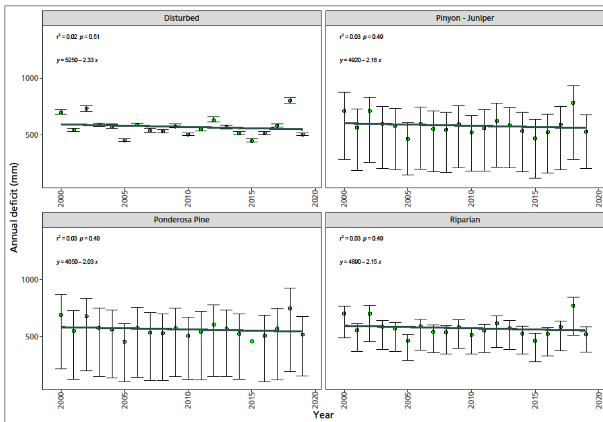
Figure 75. Cumulative annual water deficit over time (2000 to 2019) in vegetation alliance groups. The trend over time is shown for the period in gray in the previous figure. Error bars are standard error.
