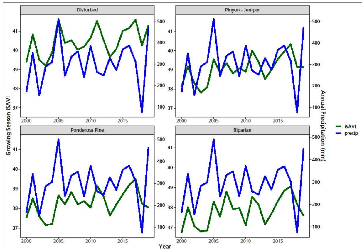
Figure 8. Co-variation in growing-season production, estimated as the iSAVI between March and October, and water-year cumulative precipitation averaged within alliance groups, demonstrating the link between climate and vegetation production in the monument at the annual scale. The time series shown here is intended to illustrate precipitation as a master climate driver of production in semiarid environments. Statistical analyses of the relation of production to precipitation and all other climate variables are the subject of following sections.
