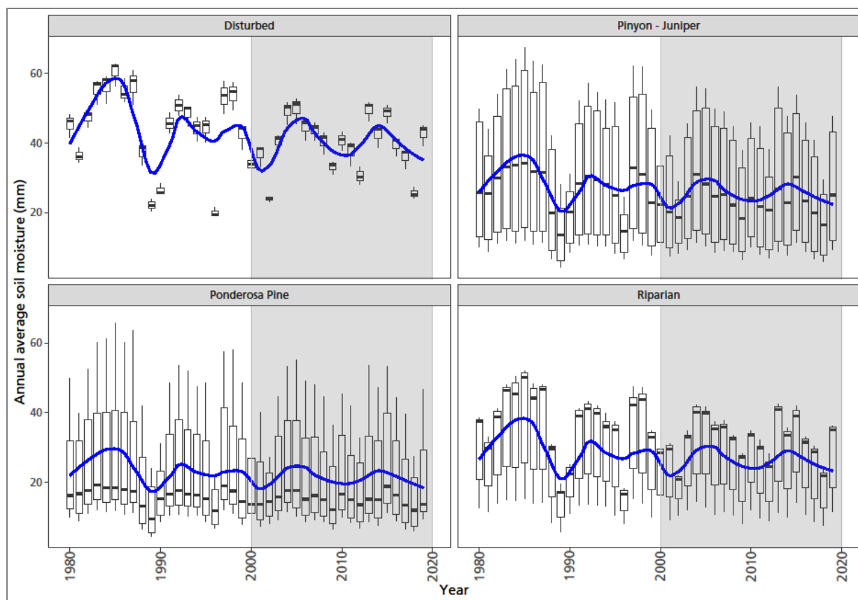
Figure 76. Annual average soil moisture over time (1980 to 2019) in vegetation alliance groups. Box plots demonstrate the range of variation within alliance groups by year. The blue line is a loess smooth with a 25 percent span to illustrate multi-year patterns. Gray shaded area includes the period investigated for relationships between production and climate when satellite imagery and climate data were both available.
