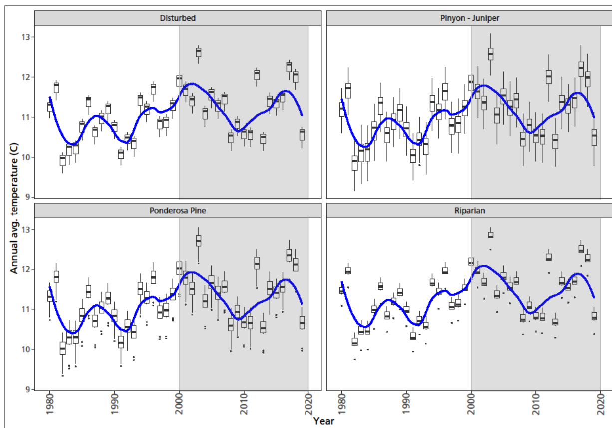
Figure 70. Annual average temperature over time (1980 to 2019) in vegetation alliance groups. Box plots demonstrate the range of variation within alliance groups by year. The blue line is a loess smooth with a 25 percent span to illustrate multiyear patterns. Gray shaded area includes the period investigated for relationships between production and climate when satellite imagery and climate data were both available.
