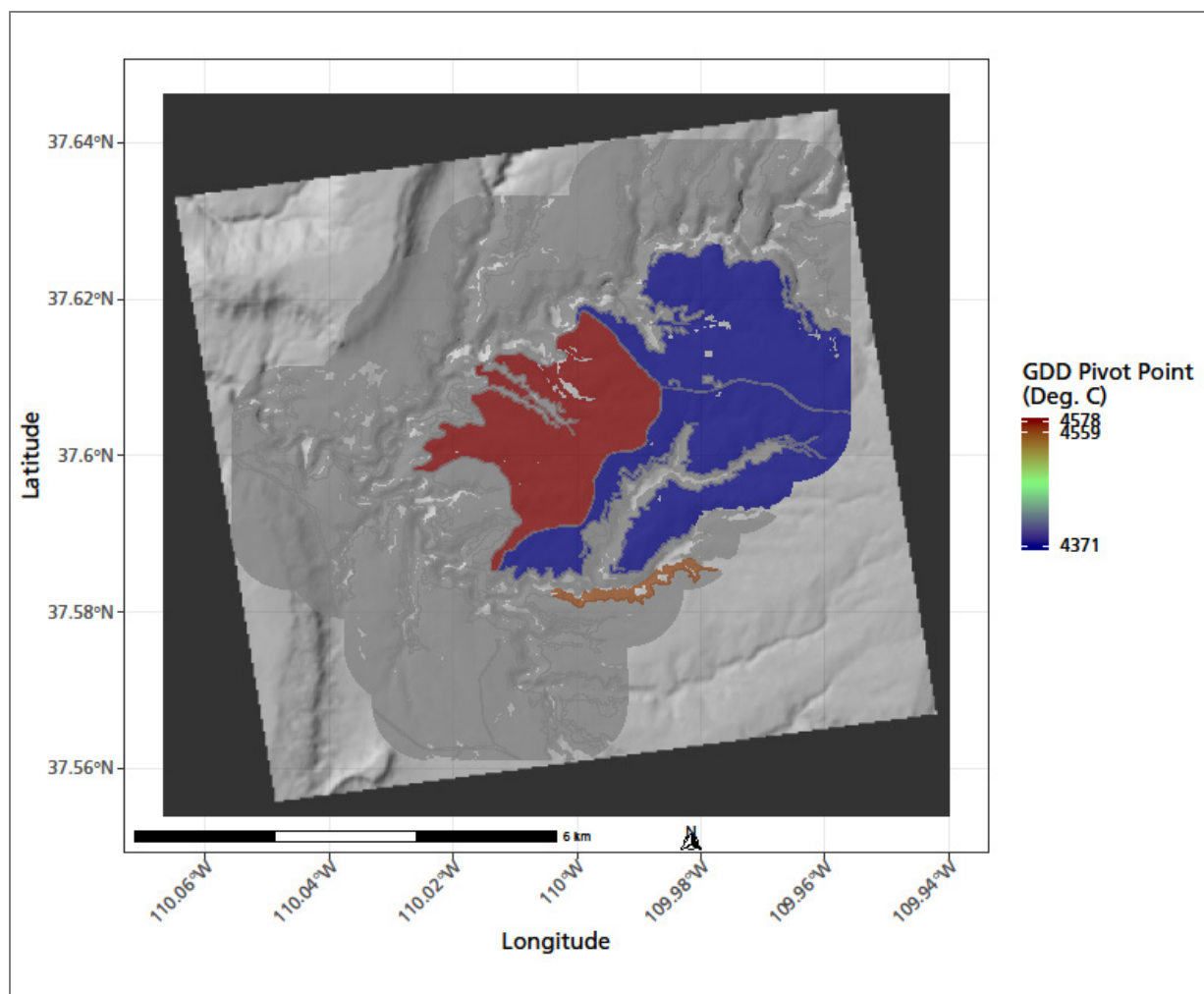
Figure 39. Pivot points for polygons where growing degree days were significantly related to interannual variation in production ( p -value < 0.05). Climate data summarized by water year.
