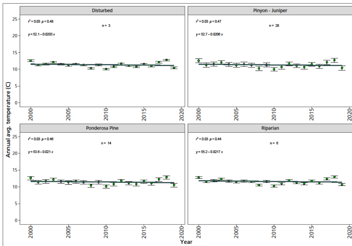
Figure 71. Annual average temperature over time (2000 to 2019) in vegetation alliance groups. The trend over time is shown for the period in gray in the previous figure. Error bars are standard error.
