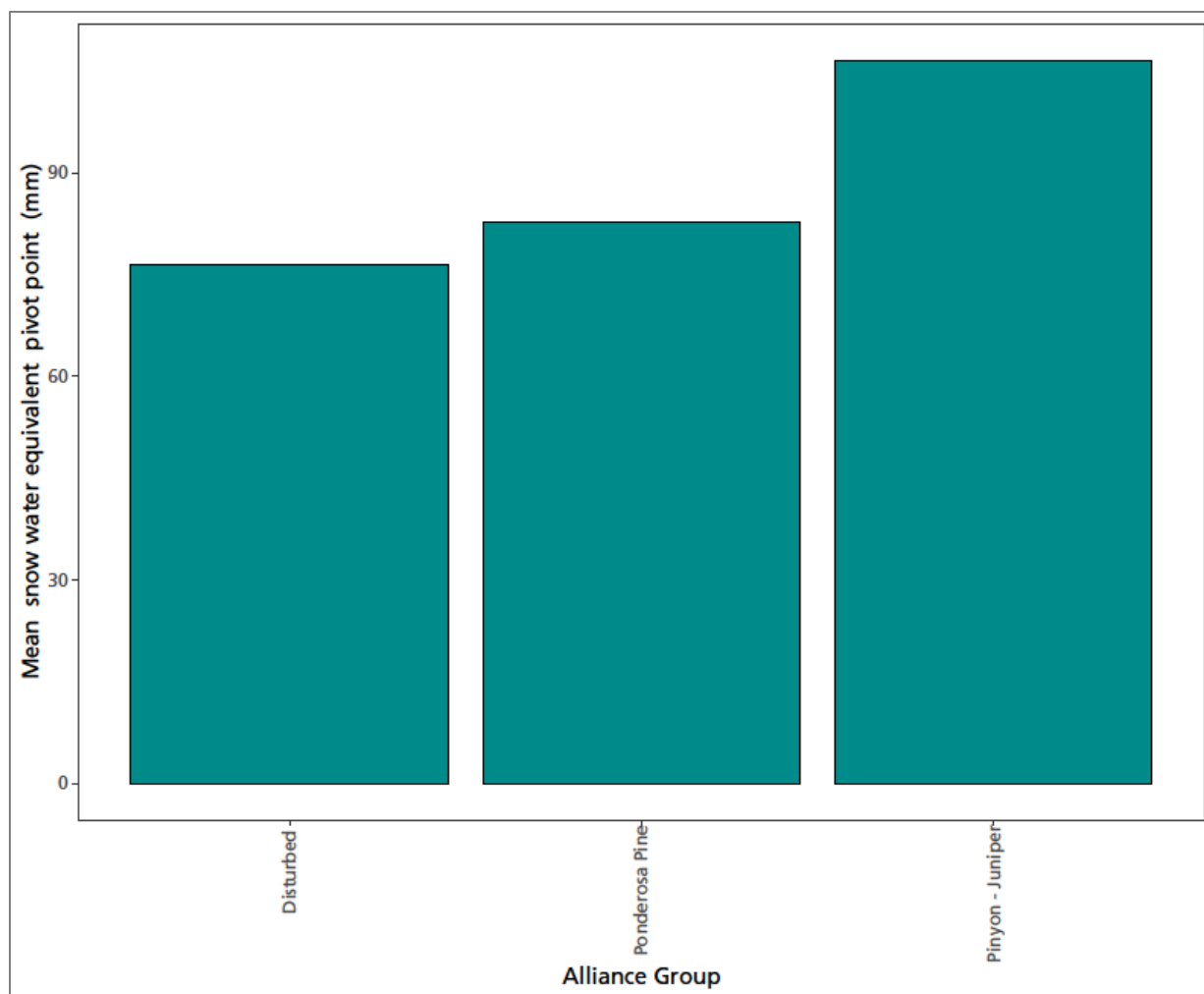
Figure 30. Pivot points for polygons where snow water equivalent was significantly related to interannual variation in production ( p -value < 0.05). Climate data summarized by water year.
