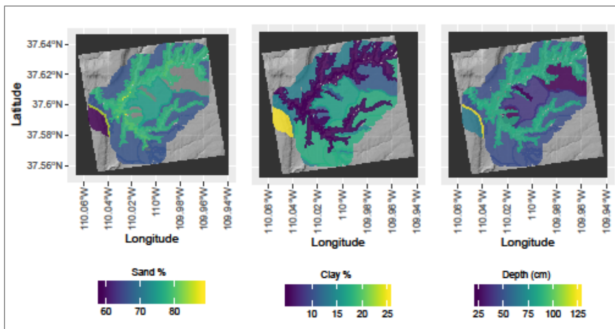
Figure 15. Maps of percentage sand content in top meter of soil, percentage clay content of soil, and depth to restrictive layer in alliance groups. Spatial patterns of soil properties correspond with patterns in vegetation response to climate. Areas of no color fill indicate missing soil properties data or depth is greater than 100 centimeters.
