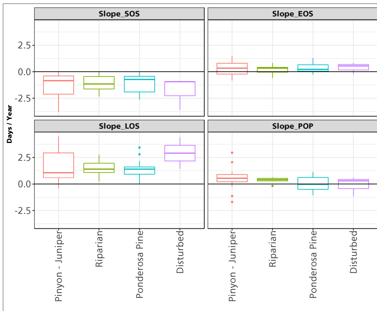
Figure 66. Direction and magnitude of change rate in land surface phenology metrics determined as \pm days per year for the start of season date (Slope SOS), end of season date (Slope EOS), length of season (Slope LOS), and timing of peak SAVI (Slope POP). Slope refers to the slope of linear regression of each phenology metric versus year for the period 2000–2019.
