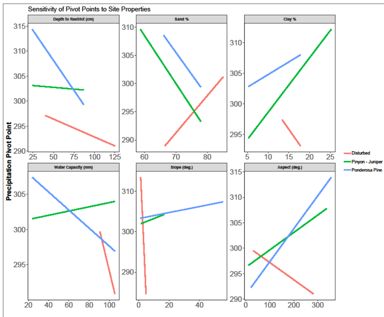
Figure 64. Variation in precipitation pivot points as related to soil and site characteristics in Natural Bridges National Monument. Steeper slopes indicate greater sensitivity of pivot points to site properties. These site properties modify climate effects by influencing soil water retention and availability, and, in the case of slope and aspect, by altering the heat load on vegetation.
