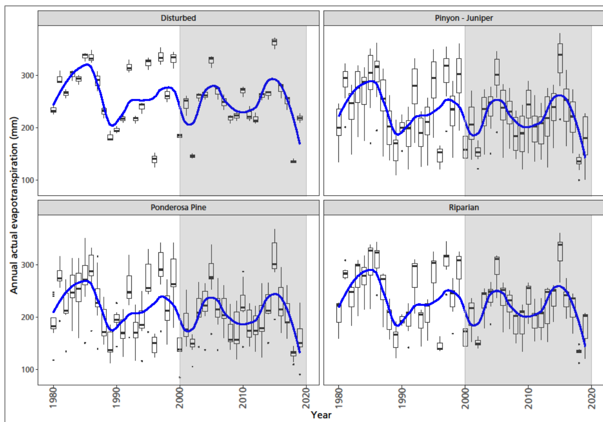
Figure 72. Cumulative annual actual evapotranspiration over time (1980 to 2019) in vegetation alliance groups. Box plots demonstrate the range of variation within alliance groups by year. The blue line is a loess smooth with a 25 percent span to illustrate multiyear patterns. Gray shaded area includes the period investigated for relationships between production and climate when satellite imagery and climate data were both available.
