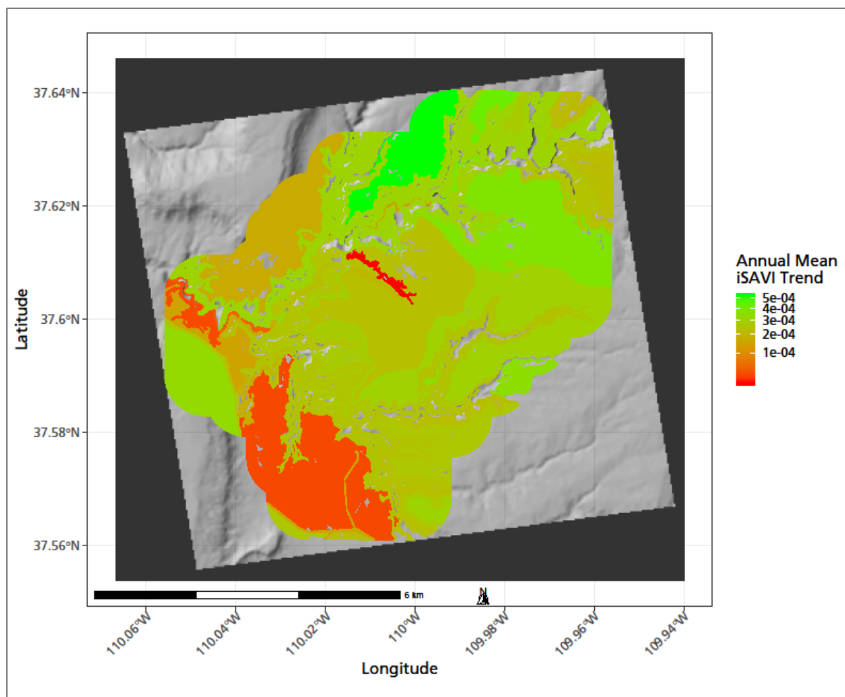
Figure 7. Spatial pattern of trends in mean annual iSAVI. Trend is average change in iSAVI per year for 2000 – 2019. Gray areas are outside the study area, too small to analyze (< 8.3 ha) or did not show a statistically significant trend (p-value < 0.05).
