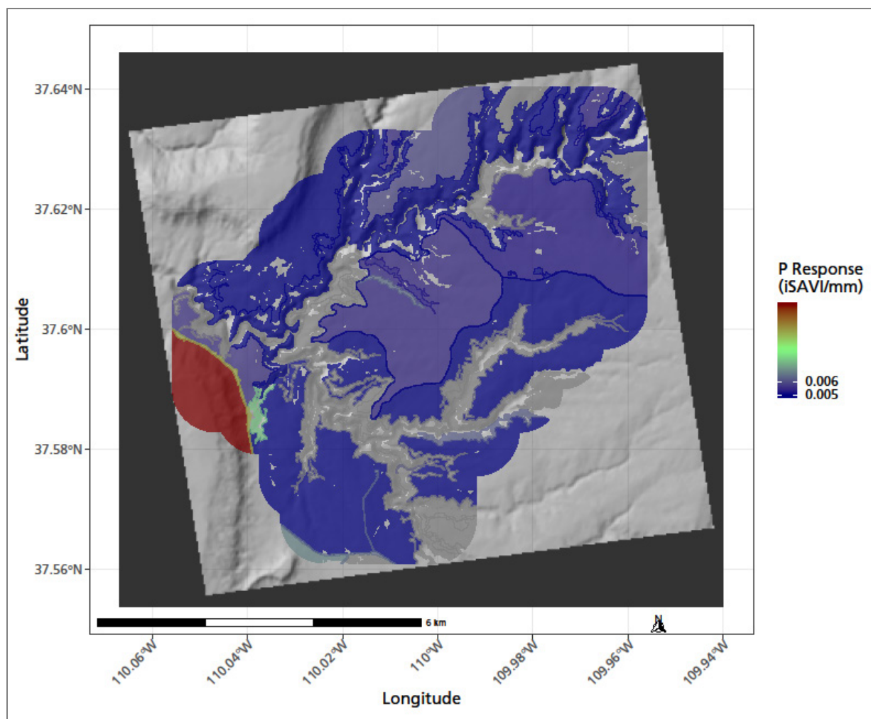
Figure 55. Sensitivity of growing season vegetation production to precipitation where the relationship was significant ( p -value < 0.05). Climate data summarized by water year.
