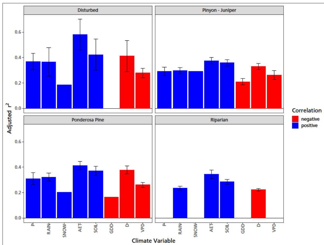
Figure 9. Significant ( p -value < 0.05) relationships between water-year climate variables and first difference of growing-season iSAVI, 2000–2019. Bar height is the mean variation in iSAVI explained by variation in climate or water-balance variable on the x-axis. Error bars are standard error. Blue bar color indicates positive correlation. Red bar color indicates negative correlation. P = precipitation (mm), RAIN = precipitation as rain (mm), SNOW = precipitation as snow (mm of water), AET = actual evapotranspiration (mm), SOIL = average soil moisture (mm), GDD = growing degree days ( ^{\circ}\text{C} ), D = climatic water deficit (mm), VPD = vapor-pressure deficit (Pa).
