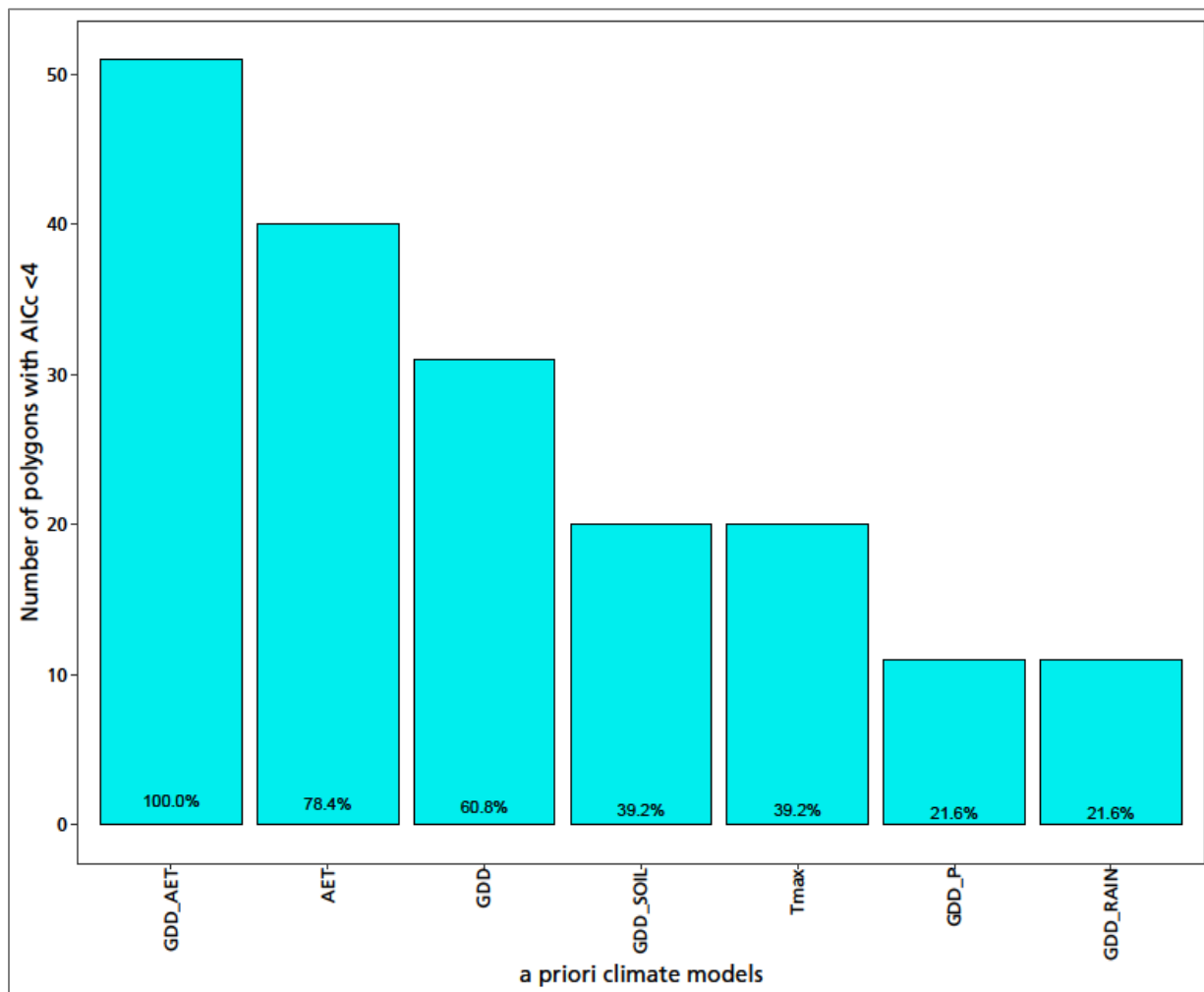
Figure 20. Top models in multi-model comparisons of climate correlates with start of growing season at the whole-monument scale. The x-axis labels refer to a priori climate models as determinants of green-up or start of season. GDD = growing degree days, AET = actual evapotranspiration, SOIL = soil moisture, Tmax = maximum temperature, P = precipitation, RAIN = precipitation as rain.
