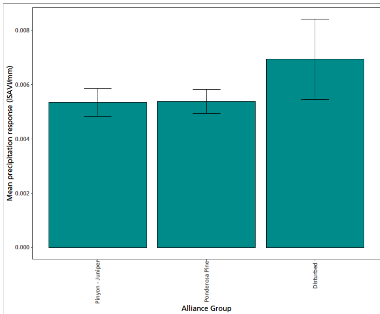
Figure 54. Sensitivity of growing season vegetation production to precipitation in polygons at Natural Bridges National Monument where the relationship was significant ( p -value < 0.05). Climate data summarized by water year.
