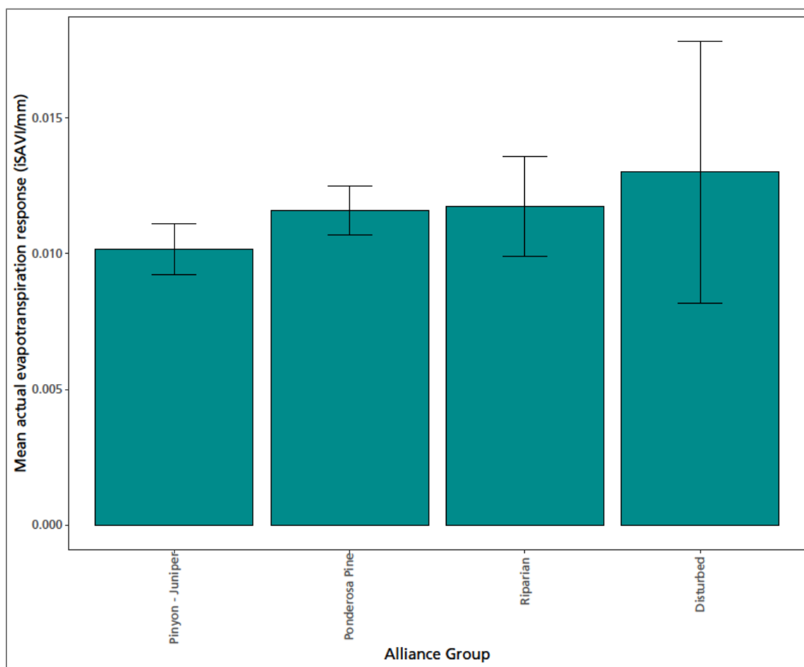
Figure 14. The mean actual evapotranspiration response values shown here represent average vegetation response to climate across different alliance groups. Standard error bars indicate variability in response among polygons within each alliance group. These values identify the typical level of evapotranspiration change ( \Delta SAV/mm) associated with climate drivers across the park's vegetation types..
