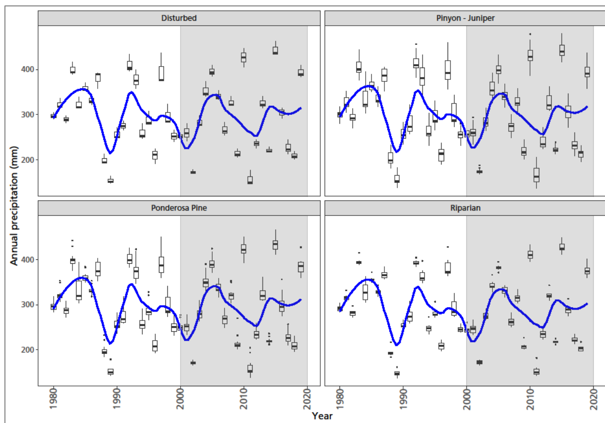
Figure 68. Cumulative annual precipitation over time (1980 to 2019) in vegetation alliance groups. Box plots demonstrate the range of variation within alliance groups by year. The blue line is a loess smooth with a 25 percent span to illustrate multiyear patterns. Gray shaded area includes the period investigated for relationships between production and climate when satellite imagery and climate data were both available.
