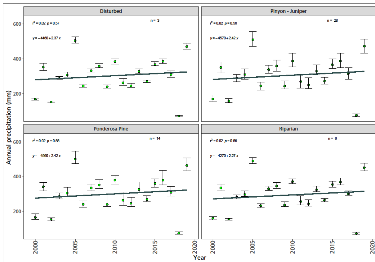
Figure 69. Cumulative annual precipitation over time (2000 to 2019) in vegetation alliance groups. The trend over time is shown for the period in gray in the previous figure. Bars are standard error. Error bars are standard error.
