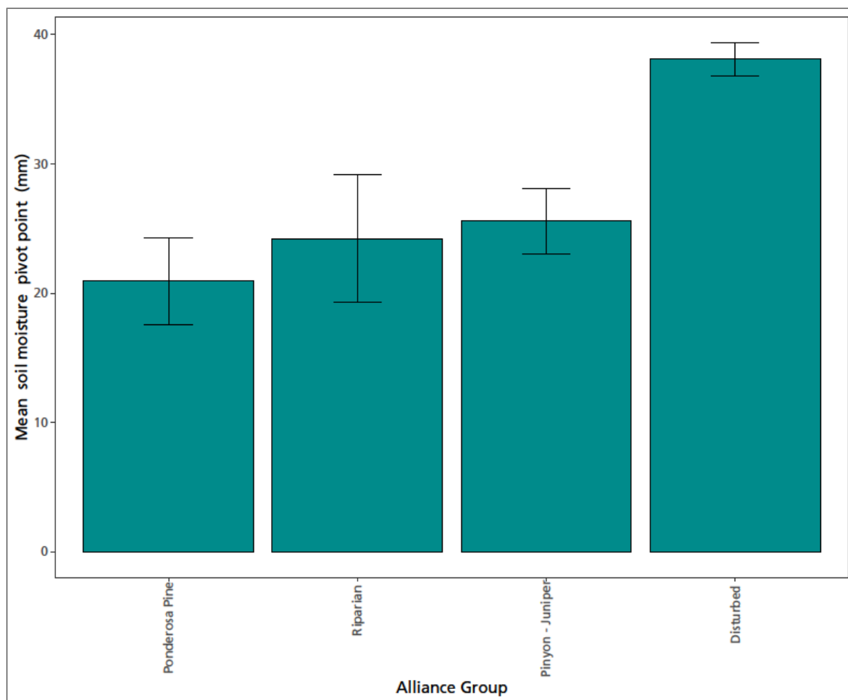
Figure 28. Pivot points for polygons in Natural Bridges National Monument where soil moisture was significantly related to interannual variation in production ( p -value < 0.05). Climate data were summarized by water year.
