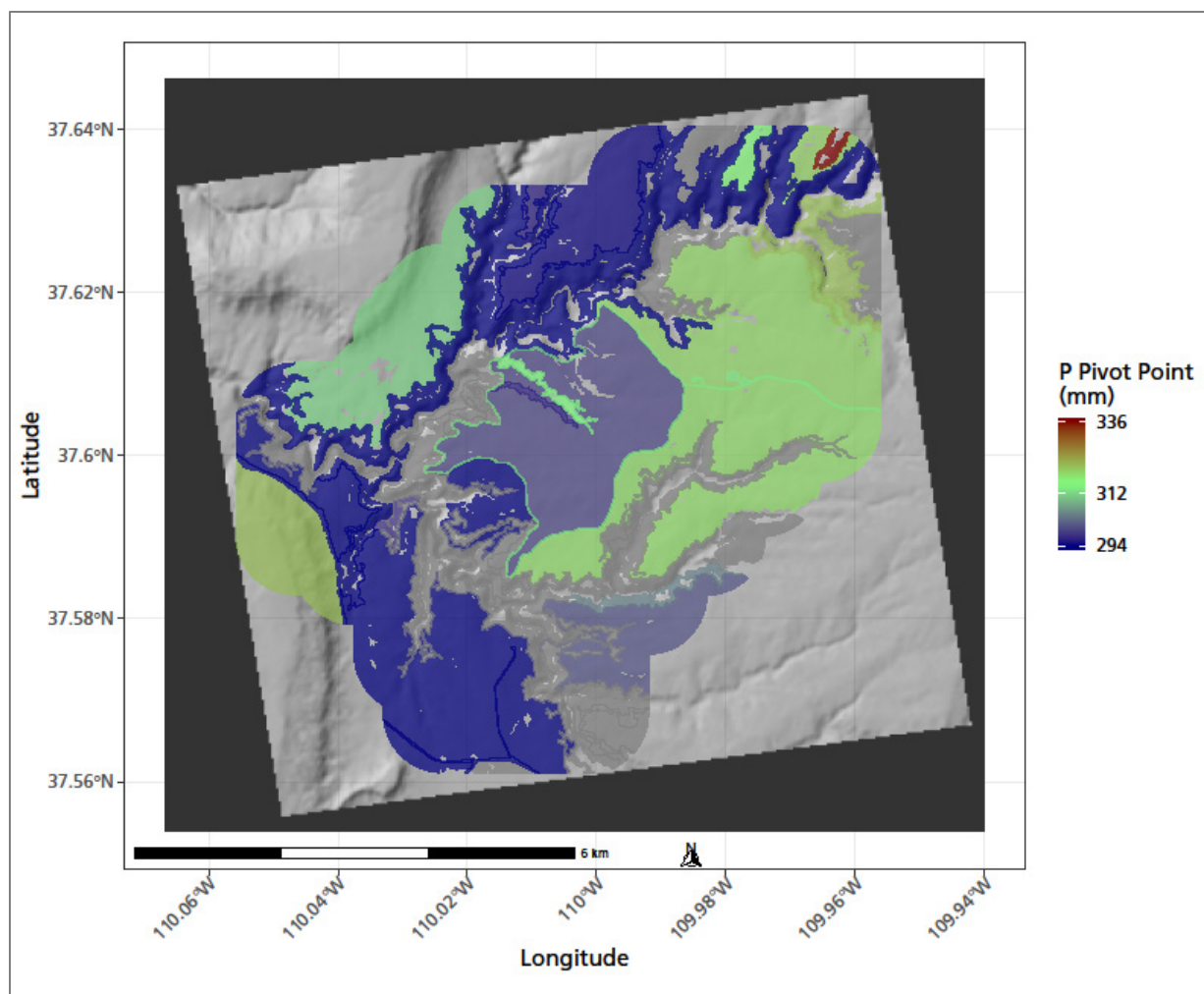
Figure 37. Pivot points for polygons where precipitation was significantly related to interannual variation in production (p-value < 0.05). Climate data summarized by water year.
