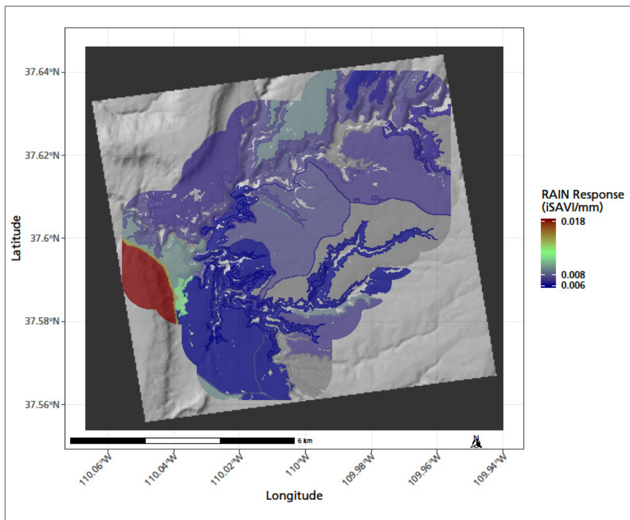
Figure 53. Sensitivity of growing season vegetation production to rain, where the relationship was significant ( p -value < 0.05). Climate data summarized by water year.
