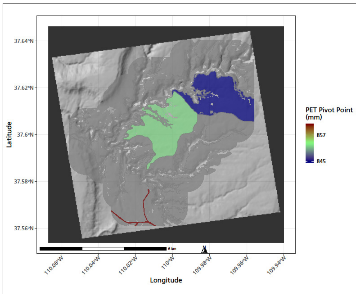
Figure 35. Pivot points for polygons where potential evapotranspiration was significantly related to interannual variation in production (p-value < 0.05). Climate data summarized by water year.
