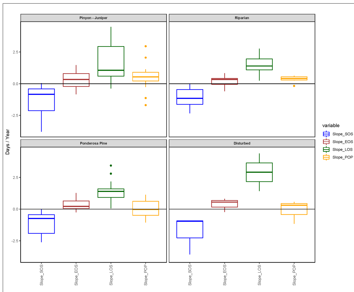
Figure 67. Direction and magnitude of change rate in land surface phenology metrics by alliance group, determined as \pm days per year for start of season date (Slope SOS), end of season date (Slope EOS), length of season (Slope LOS), and timing of peak SAVI (Slope POP). Slope refers to the slope of linear regression of phenology metric versus year for the period 2000–2019.
