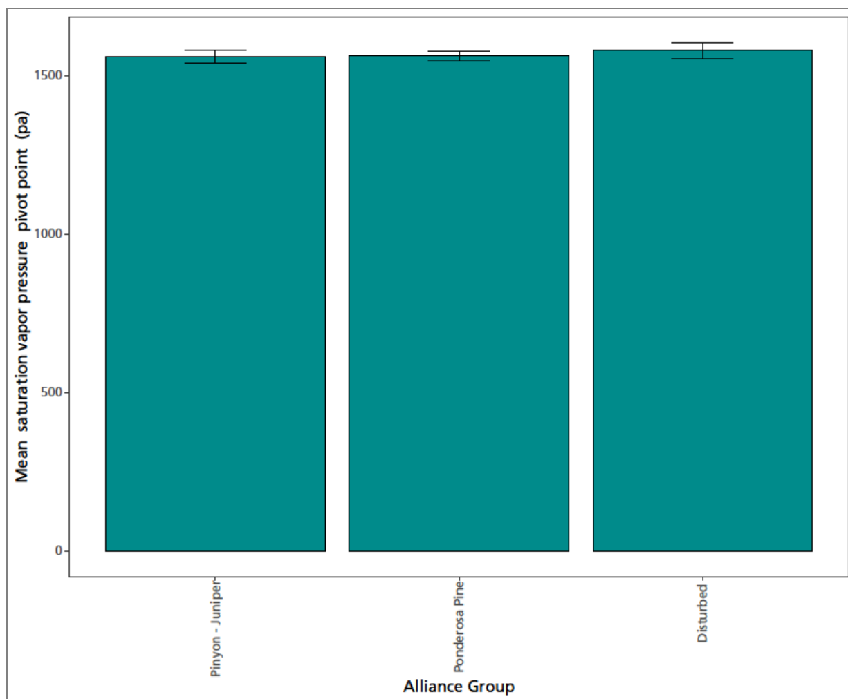
Figure 48. Pivot points for polygons in Natural Bridges National Monument where saturation vapor pressure was significantly related to interannual variation in production (p-value < 0.05). Climate data summarized by water year.
