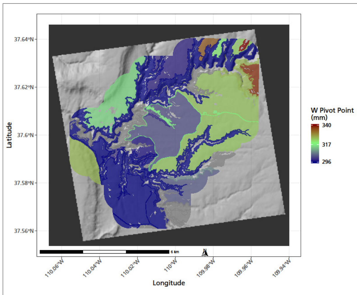
Figure 45. Pivot points for polygons where snow melt plus rain were significantly related to interannual variation in production (p-value < 0.05). Climate data summarized by water year.
