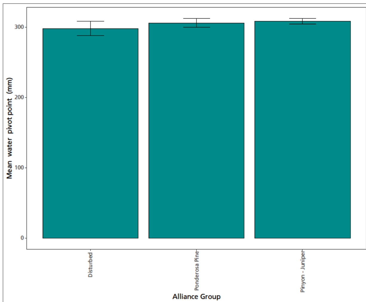
Figure 44. Pivot points for polygons in Natural Bridges National Monument where water was significantly related to interannual variation in production ( p -value < 0.05 ). Climate data summarized by water year. NPS / DAVID THOMA
