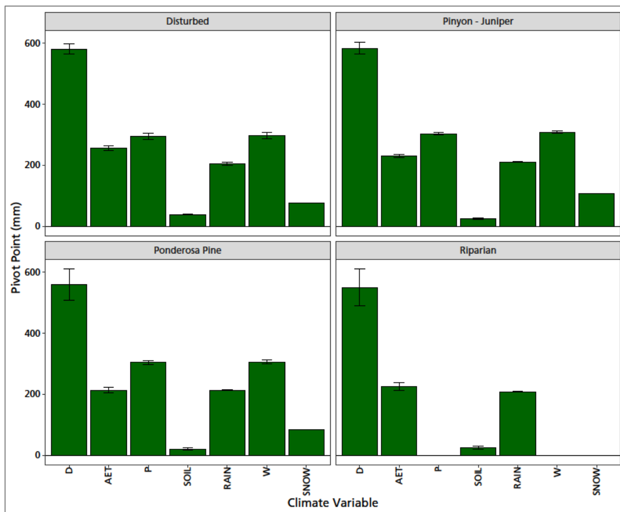
Figure 12. Significant ( p -value < 0.05) water-related pivot points by alliance group. See Tables S-2 and S-4 in NPS (2025) for the pivot point values. The magnitude of each pivot point reflects generally average conditions for polygons in each alliance group. The mean pivot-point values are the critical values where annual production switches from below to above average (relative to previous year) for the different alliance groups. D = climatic water deficit (mm), AET = actual evapotranspiration (mm), P = precipitation (mm), SOIL = average soil moisture (mm), RAIN = precipitation as rain (mm), W = snowmelt plus rain (mm), SNOW = precipitation as snow (mm).
