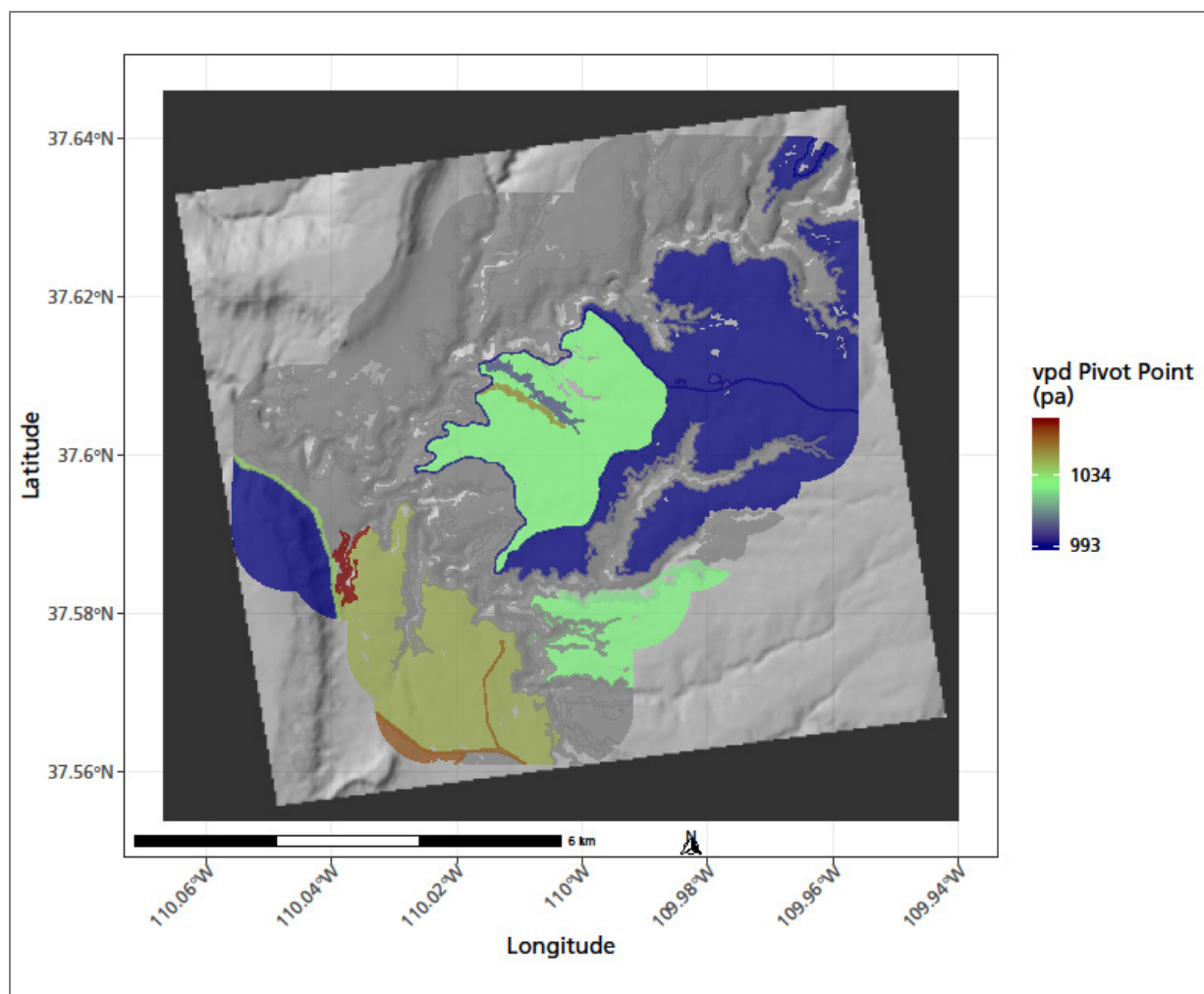
Figure 47. Pivot points for polygons where vapor pressure deficit was significantly related to interannual variation in production (p-value < 0.05). Climate data summarized by water year.
