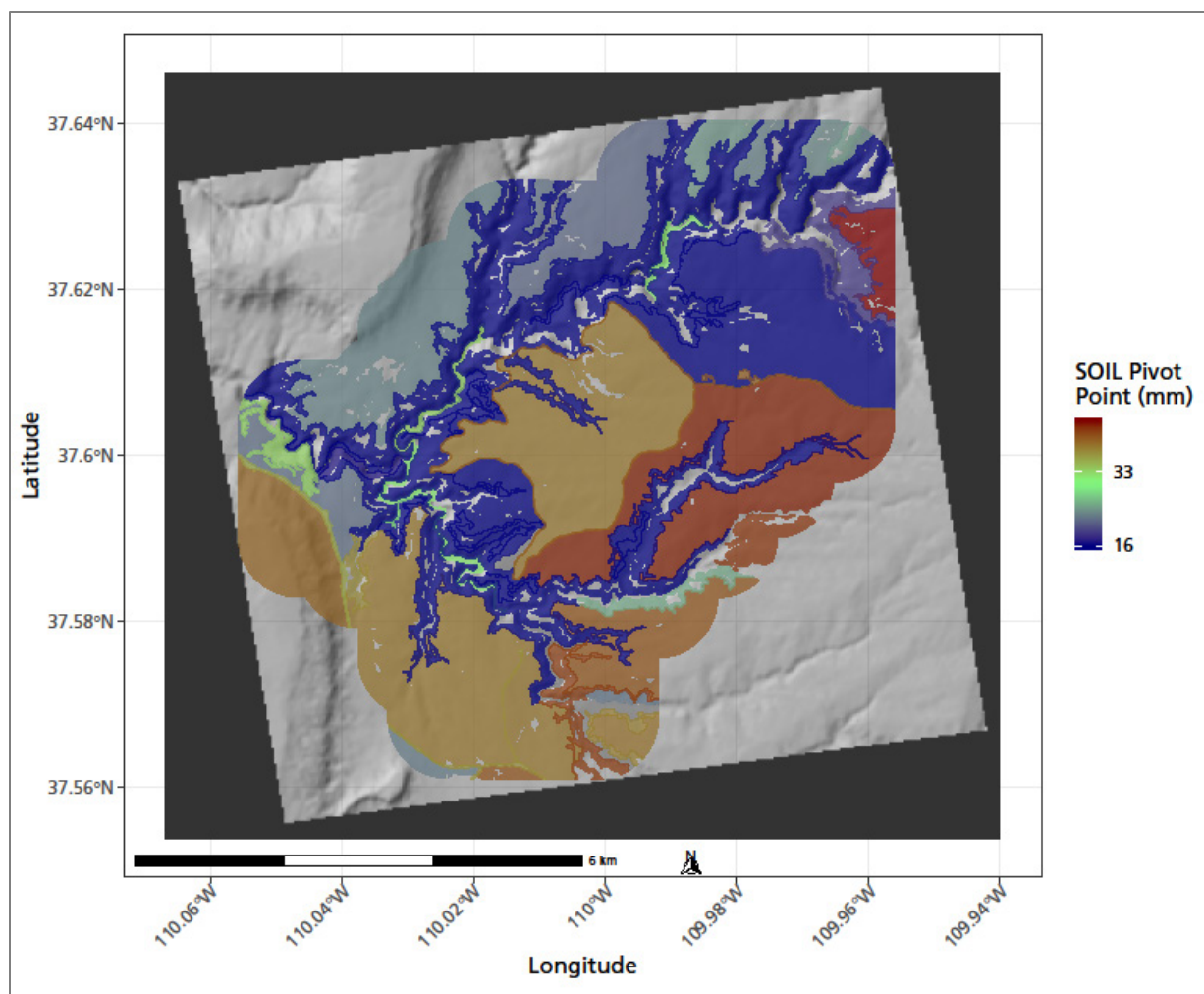
Figure 29. Pivot points for polygons where soil moisture was significantly related to interannual variation in production ( p -value < 0.05 ). Climate data summarized by water year.
