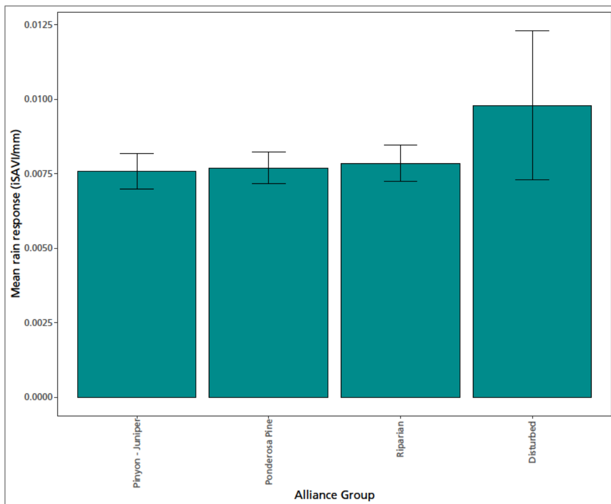
Figure 52. Sensitivity of growing season vegetation production to rain in polygons at Natural Bridges National Monument where the relationship was significant ( p -value < 0.05). Climate data summarized by water year.
