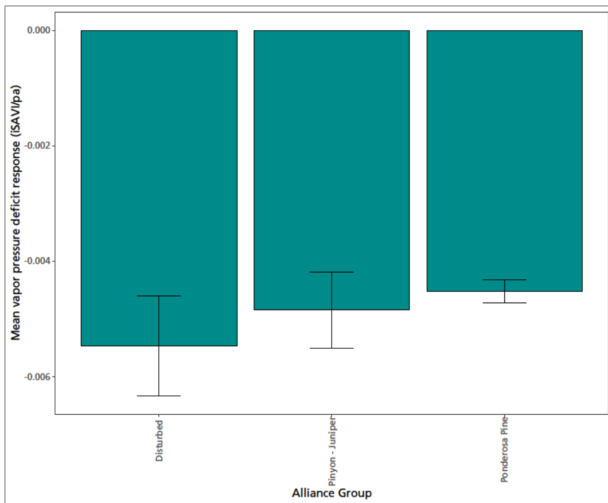
Figure 62. Sensitivity of growing season vegetation production to vapor pressure deficit in polygons at Natural Bridges National Monument where the relationship was significant ( p -value < 0.05). Climate data summarized by water year.
