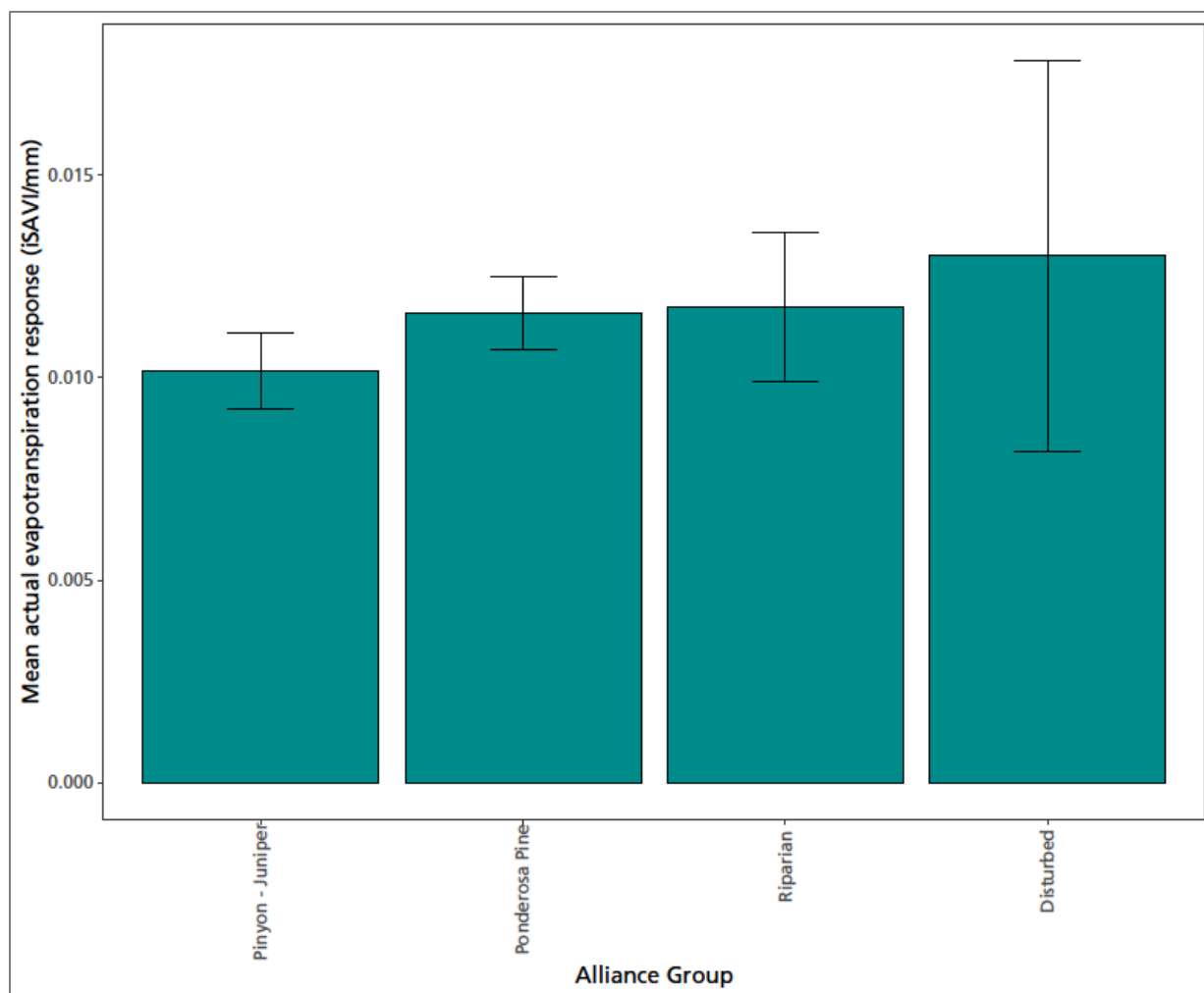
Figure 58. Sensitivity of growing season vegetation production to actual evapotranspiration in polygons at Natural Bridges National Monument where the relationship was significant ( p -value < 0.05). Climate data summarized by water year.
