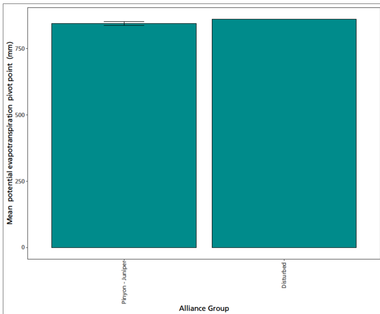
Figure 34. Pivot points for polygons in Natural Bridges National Monument where potential evapotranspiration was significantly related to interannual variation in production (p-value < 0.05). Climate data summarized by water year.
