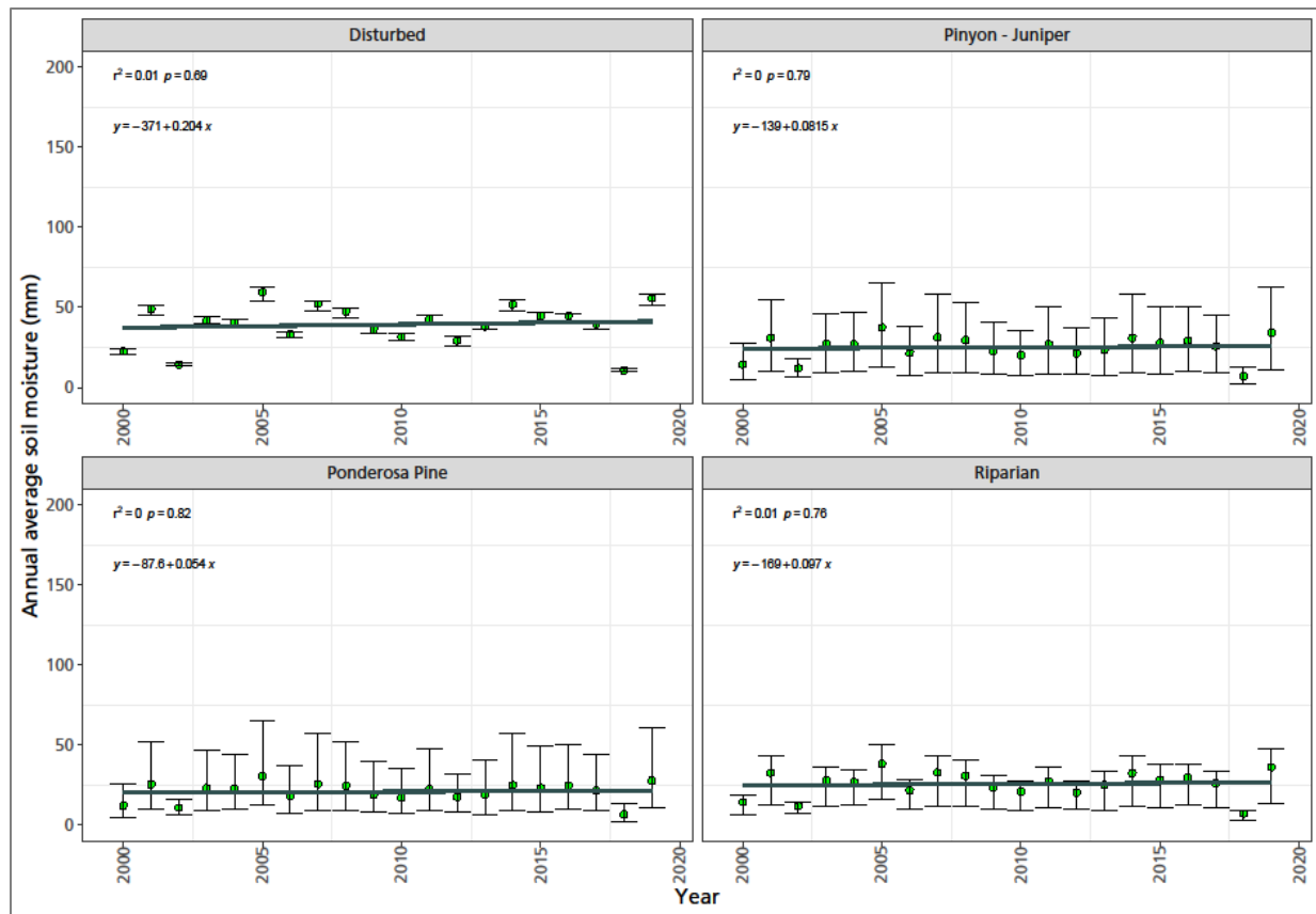
Figure 77. Annual average soil moisture over time (2000 to 2019) in vegetation alliance groups. The trend over time is shown for the period in gray in the previous figure. Error bars are standard error.
