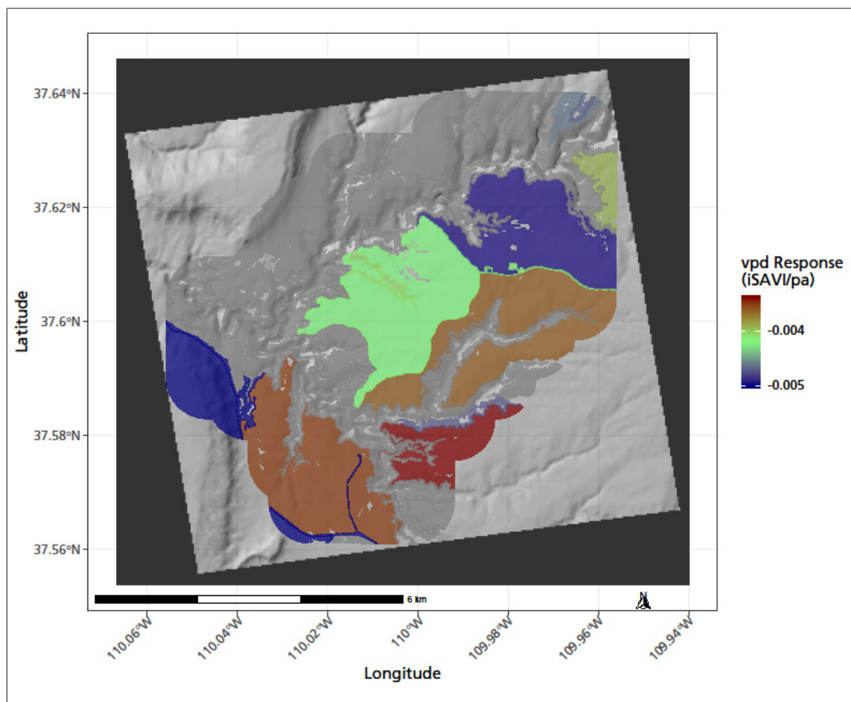
Figure 63. Sensitivity of growing season vegetation production to vapor pressure deficit where the relationship was significant ( p -value < 0.05). Climate data summarized by water year.
