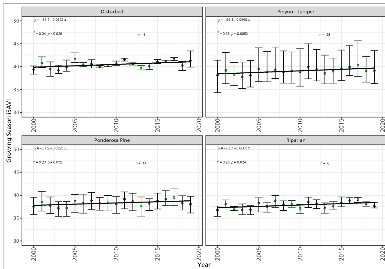
Figure 6. Trends in mean growing-season iSAVI by alliance group, determined via simple linear regression. Bars are standard error among polygons within each alliance group. n = number of polygons analyzed in each alliance group, r^2 = coefficient of determination, p = p-value, y = growing season iSAVI, x = year.
