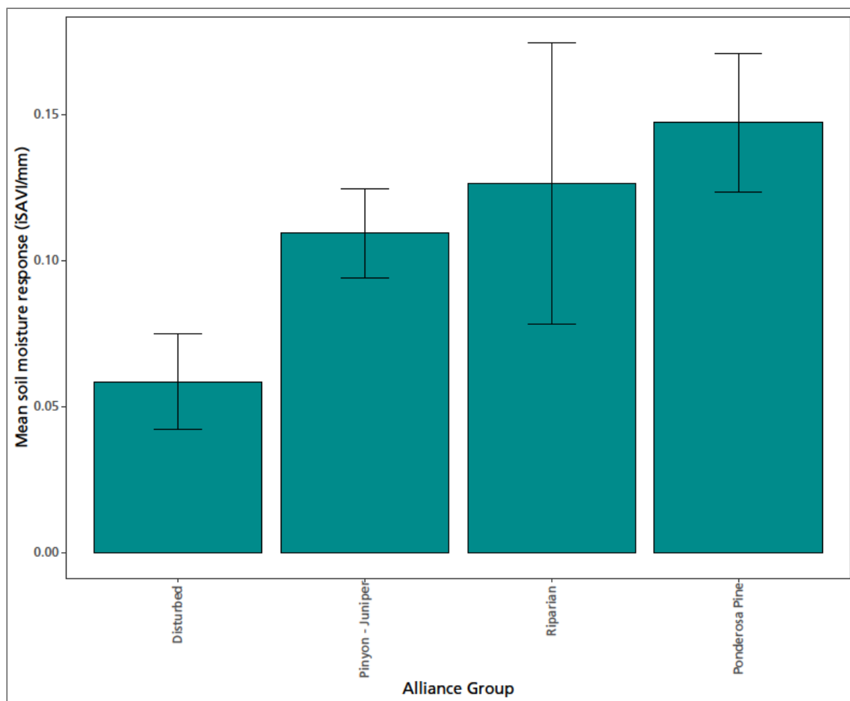
Figure 50. Sensitivity of growing season vegetation production to soil moisture in polygons at Natural Bridges National Monument where the relationship was significant ( p -value < 0.05). Climate data summarized by water year.
