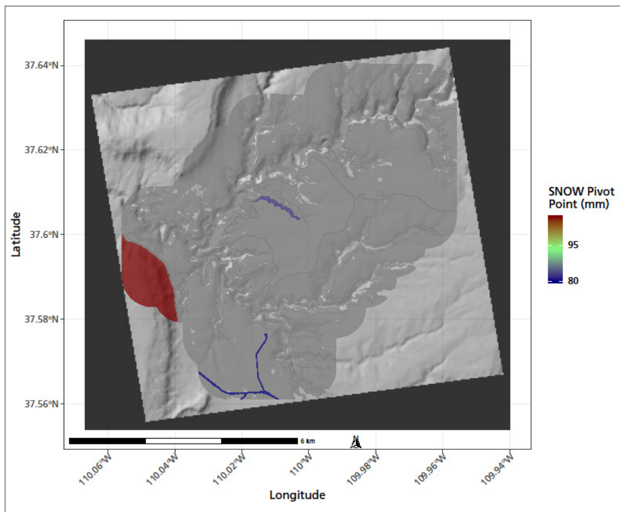
Figure 31. Pivot points for polygons where snow was significantly related to interannual variation in production ( p -value < 0.05). Climate data summarized by water year.
