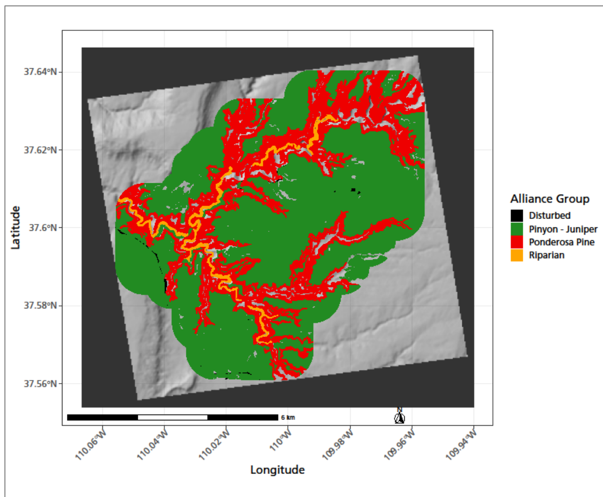
Figure 1. NCPN alliance groups analyzed for trends in production, phenology, and climate relations at Natural Bridges National Monument. Areas not colored within the study boundary are alliance polygons smaller than the minimum target area of 8.3 hectares.
