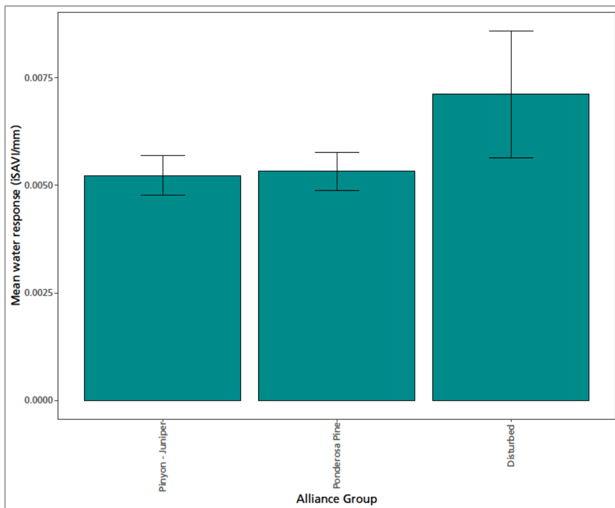
Figure 60. Sensitivity of growing season vegetation production to water in polygons at Natural Bridges National Monument where the relationship was significant ( p -value < 0.05 ). Climate data summarized by water year.
