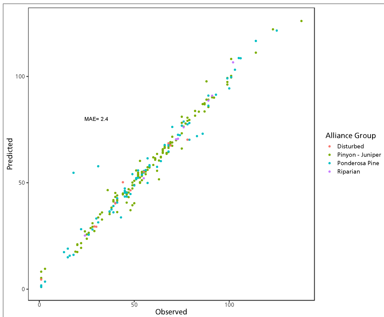
Figure 23. Predicted start-of-season date versus observed start-of-season date in the holdout dataset used for validation of the random-forests model for all polygons in Natural Bridges National Monument. MAE is mean absolute error of prediction in days. Polygons with annual peaks (POP) occurring between November 1 and April 1 were removed prior to this analysis (Norris and Walker 2020).
