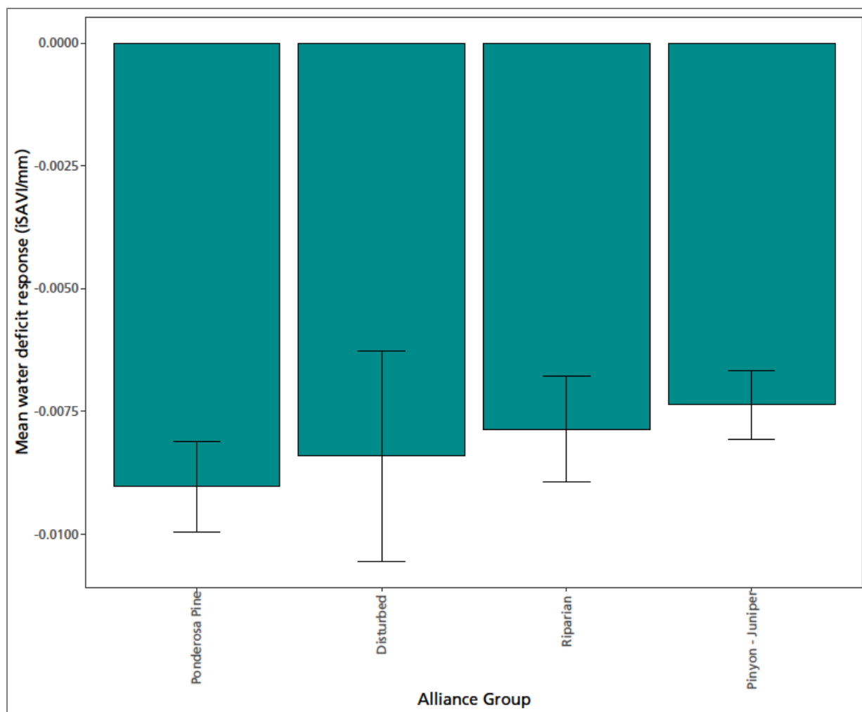
Figure 56. Sensitivity of growing season vegetation production to water deficit in polygons at Natural Bridges National Monument where the relationship was significant ( p -value < 0.05). Climate data summarized by water year.
