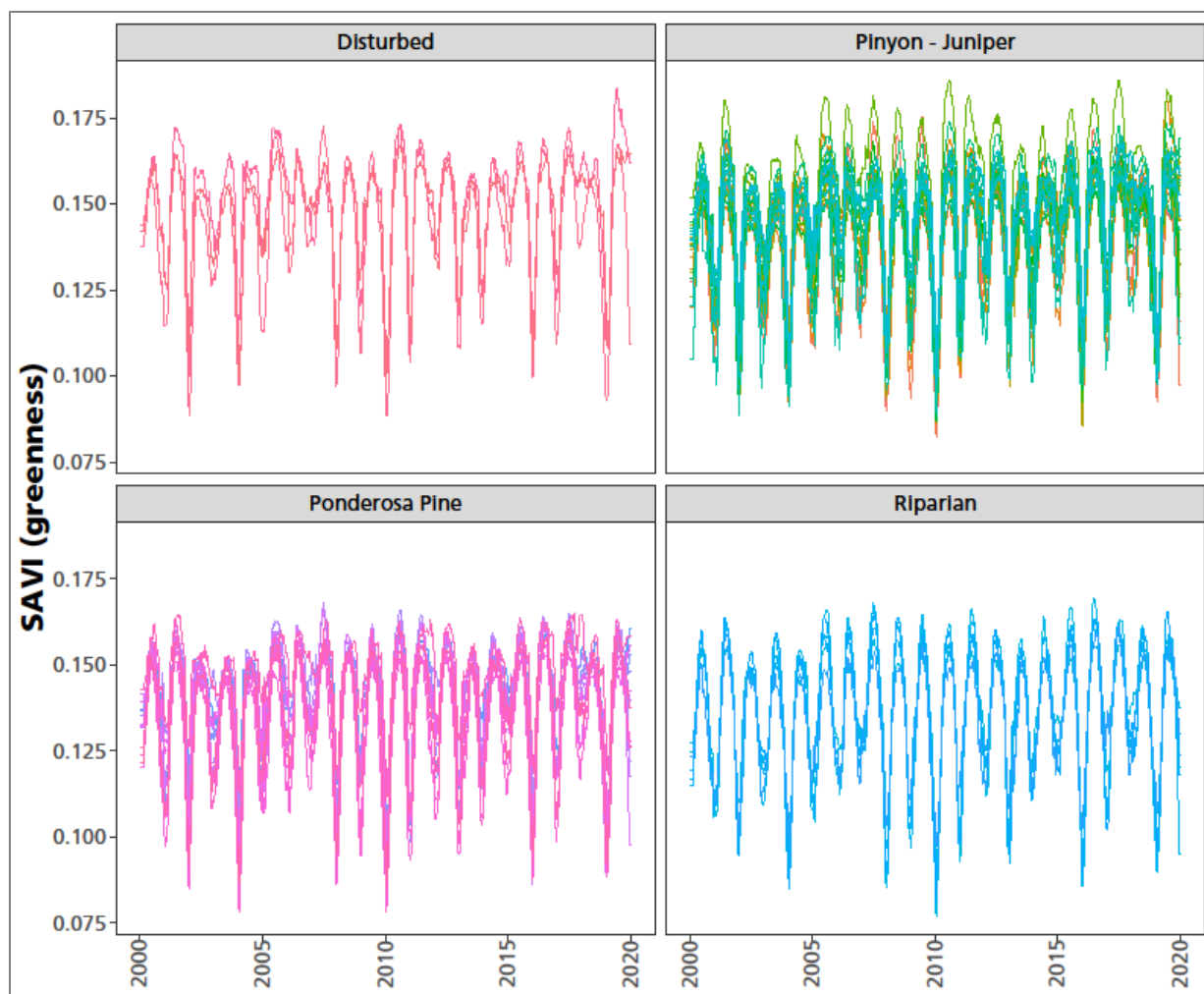
Figure 5. Soil-adjusted vegetation index time series by alliance group for 51 polygons analyzed for 2000–2019. Colors help differentiate individual polygon time series traces. Each polygon time series was filtered to include only high-quality pixel values, with minimum values truncated to winter minimum, gap-filled, and then smoothed with a Savitsky-Golay moving-window filter to remove high-frequency noise. Analysis was limited to polygons of > 8.3 hectares. A single-line trace indicates either all polygon units have similar seasonality and interannual variation, or only one polygon of the alliance group was sampled.
