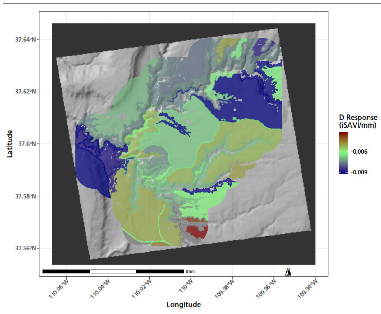
Figure 57. Sensitivity of growing season vegetation production to water deficit where the relationship was significant ( p -value < 0.05). Climate data summarized by water year.
