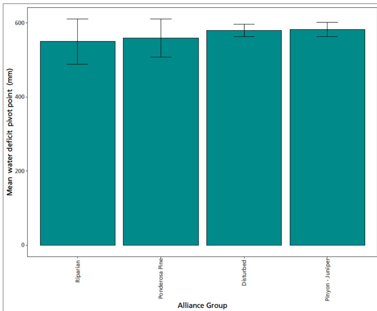
Figure 40. Pivot points for polygons in Natural Bridges National Monument where water deficit was significantly related to interannual variation in production ( p -value < 0.05 ). Climate data summarized by water year.
