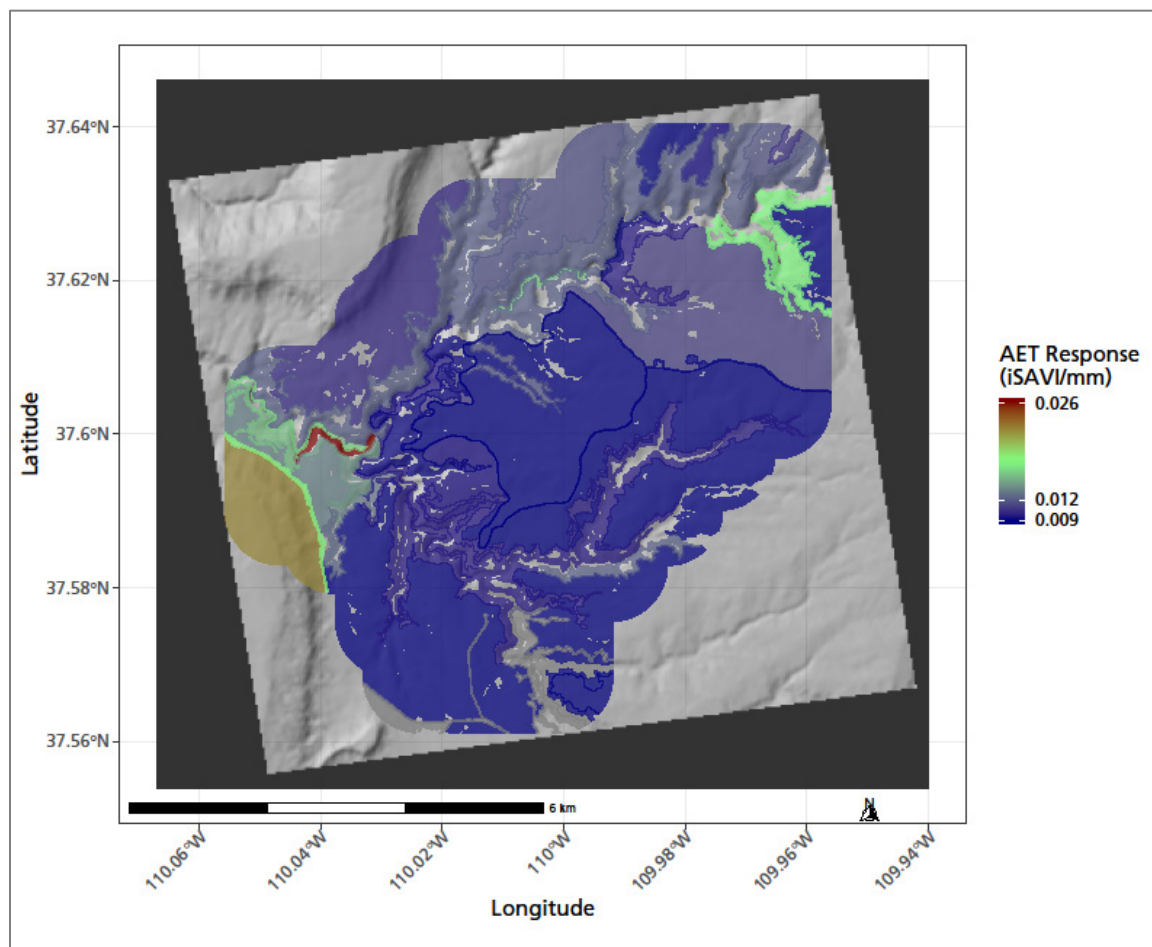
Figure 13. Actual evapotranspiration response for polygons with a significant relationship ( p -value < 0.05) between annual precipitation and change in annual vegetation production, assessed as the interannual difference in iSAVI. The \Delta iSAVI/mm values shown here represent spatial patterns in vegetation sensitivity to precipitation across the landscape.
