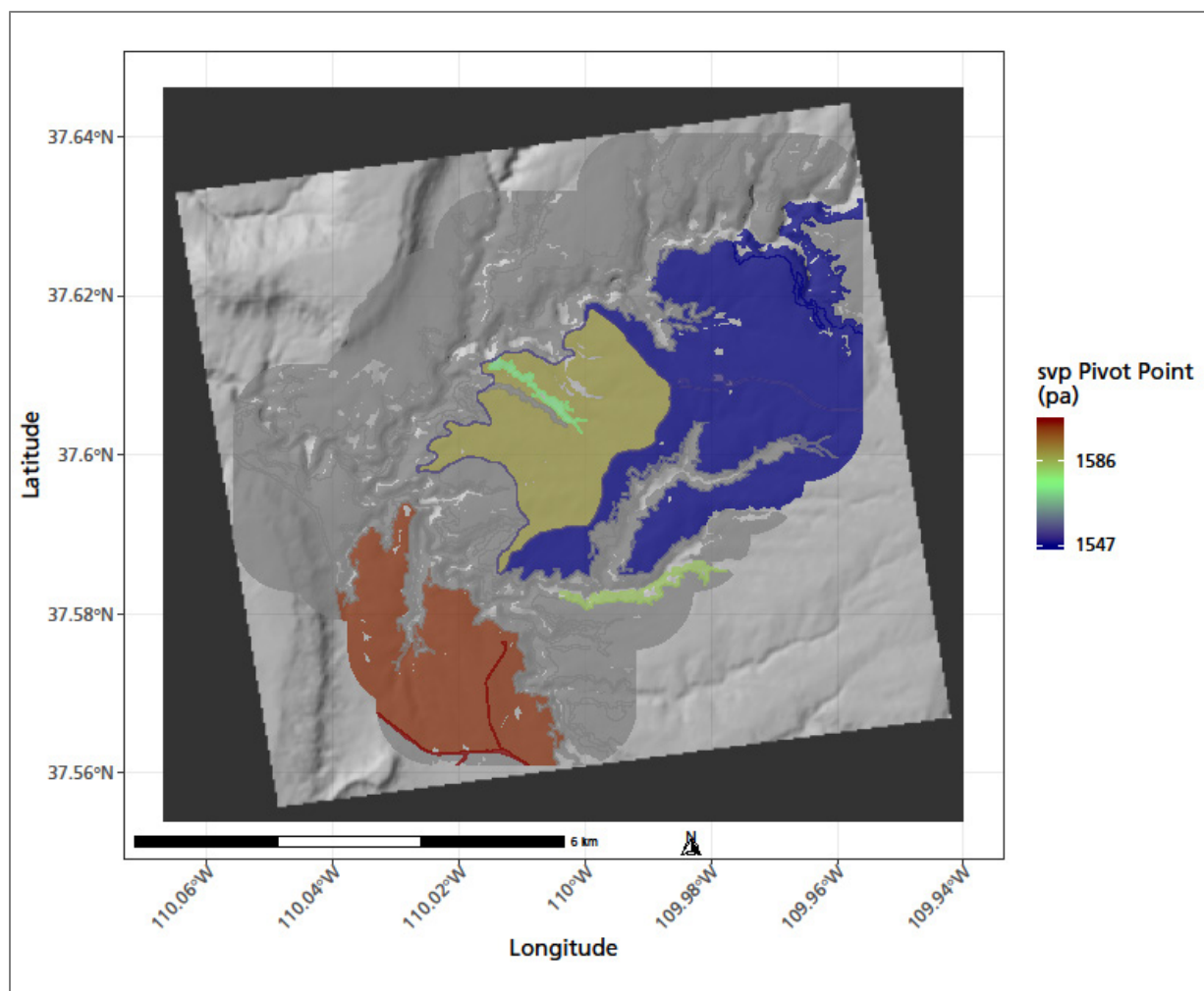
Figure 49. Pivot points for polygons where saturation vapor pressure was significantly related to interannual variation in production (p-value < 0.05). Climate data summarized by water year. NPS / DAVID THOMA
