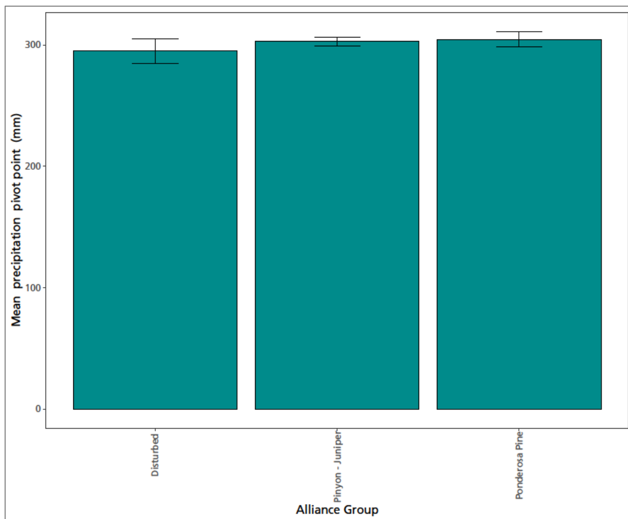
Figure 36. Pivot points for polygons in Natural Bridges National Monument where precipitation was significantly related to interannual variation in production ( p -value < 0.05). Climate data summarized by water year.
