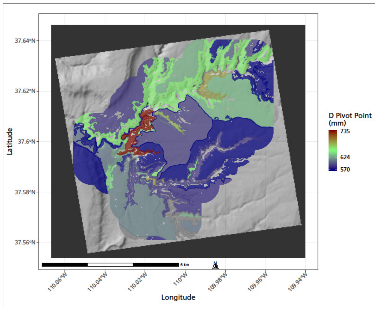
Figure 41. Pivot points for polygons where water deficit was significantly related to interannual variation in production ( p -value < 0.05). Climate data summarized by water year.
