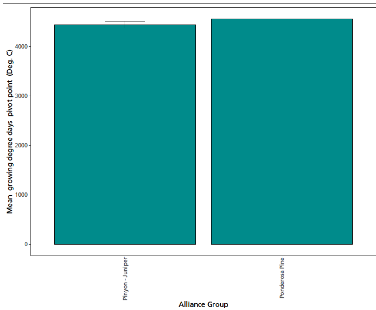
Figure 38. Pivot points for polygons in Curecanti NRA where growing degree days were significantly related to interannual variation in production ( p -value < 0.05 ). Climate data summarized by water year. NPS / DAVID THOMA
