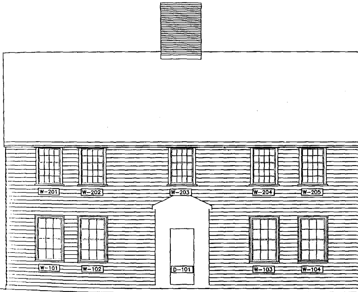
SOUTH ELEVATION OLIVE STOW HOUSE MINUTE MAN NHP NORTHEAST CULTURAL RESOURCES CENTER BUILDING CONSERVATION BRANCH SCALE: NOT TO SCALE
