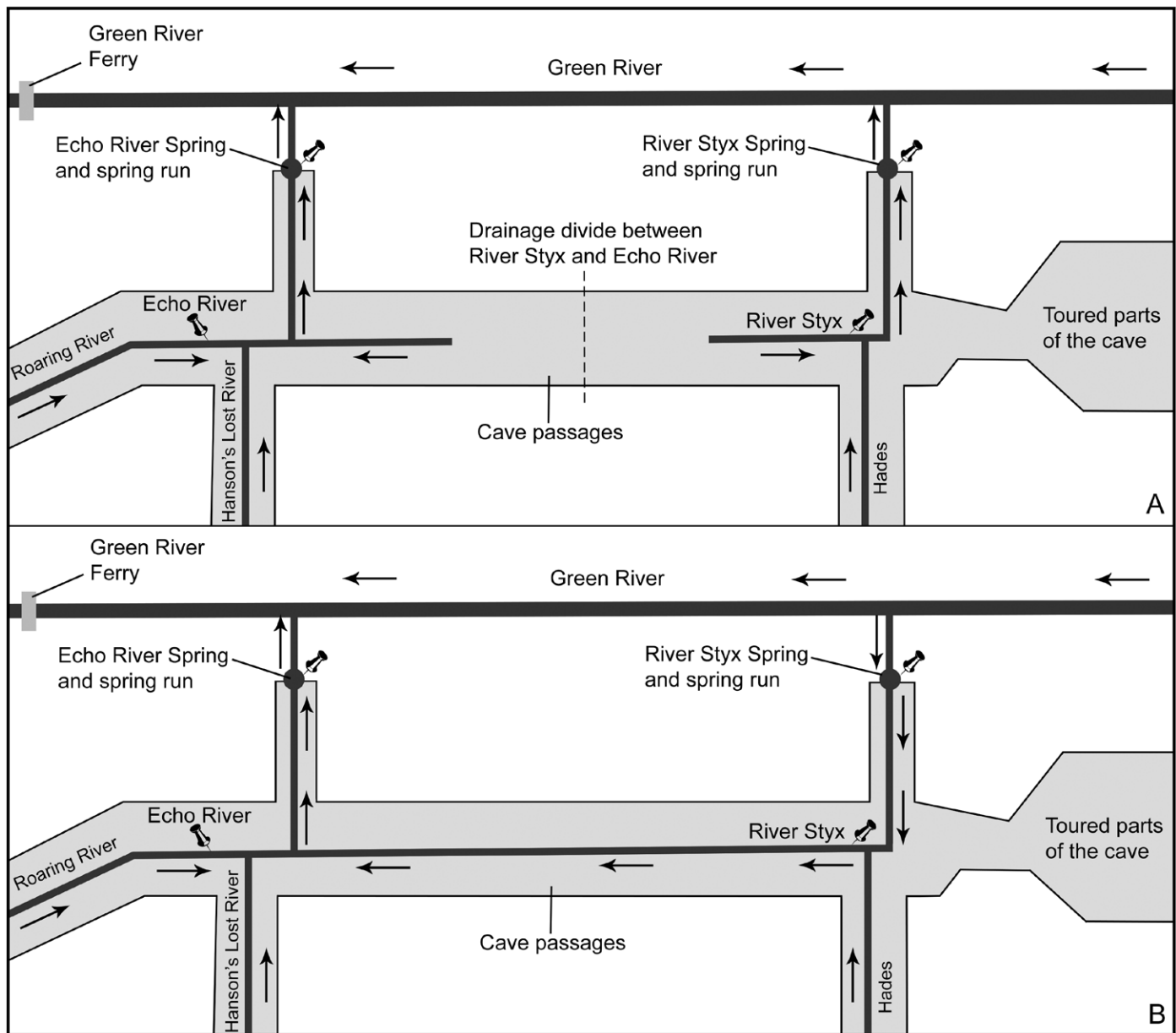
Figure 4. Schematic diagrams illustrating a) the normal flow pattern of River Styx out of the cave, and b) the reverse-flow pattern of River Styx into the cave. In diagram A, River Styx and Echo River are separated by a low, wide sandbar, which serves as a divide between the two karst drainage basins. When the River Styx reverses direction, it flows over the sandbar and into Echo River, as illustrated in diagram B. Pushpins show the study sites at River Styx, Echo River, and the two springs. Diagrams are highly simplified and not drawn to scale.
