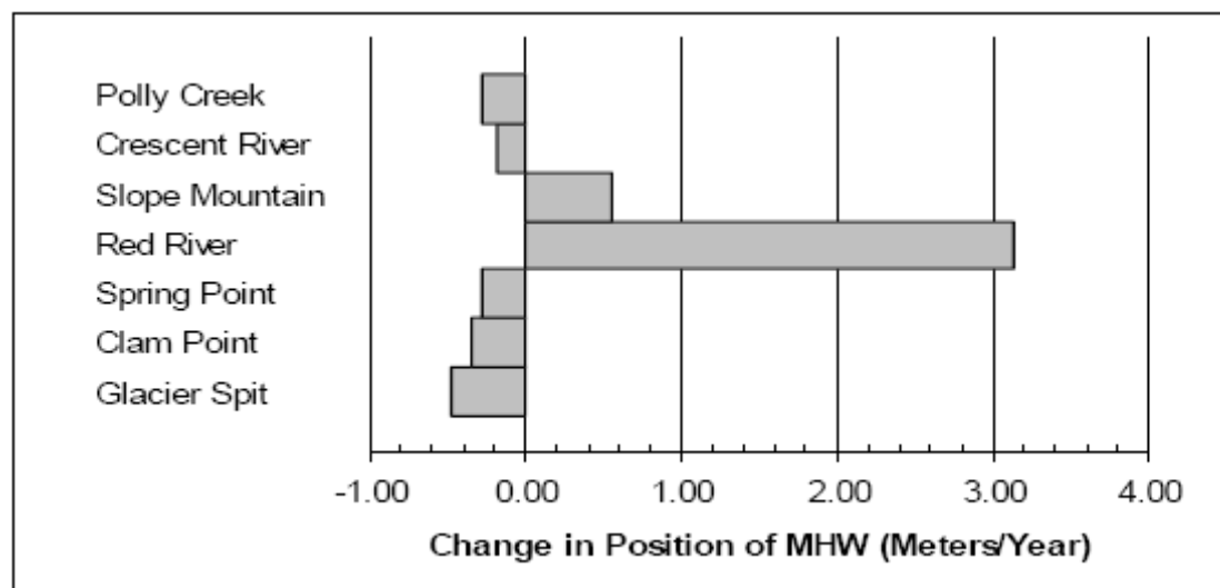
Figure 55. Annual rates of erosion and accretion (in terms of change in position of mean high water) from 1992-2004 at the seven cross-shore beach profiles measured by Cusick and Bennett (2005).
