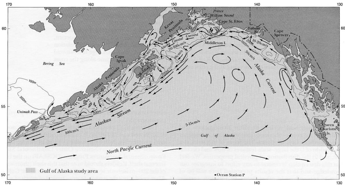
Figure 3. Predominant currents in the GOA (Reed and Schumacher, 1986).
