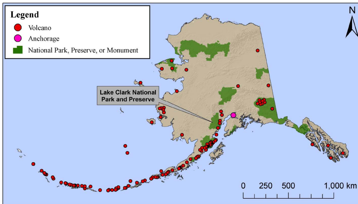
Figure 52. Location of volcanoes in Alaska.
