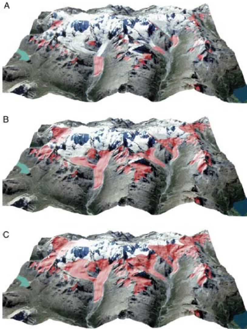
Figure 51. Visualization of new modeled glacier size in the Swiss Alps for Equilibrium Line Altitude upward shifts of 100m (a), 300 m (b), and 500 m (c). Areas of ice lost are shown in the red shaded color.
