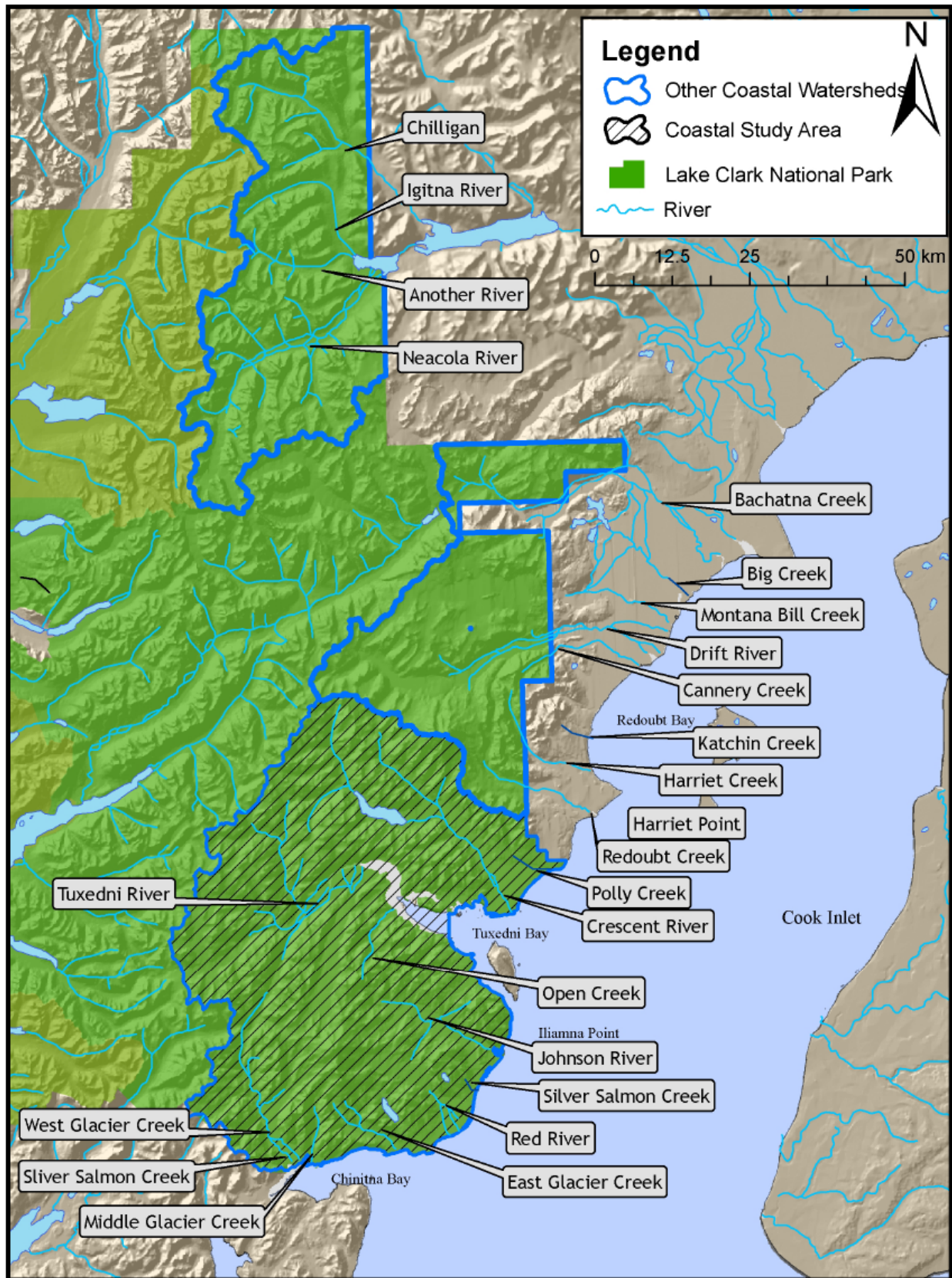
Figure 11. Major streams within the LACL coastal study area.
