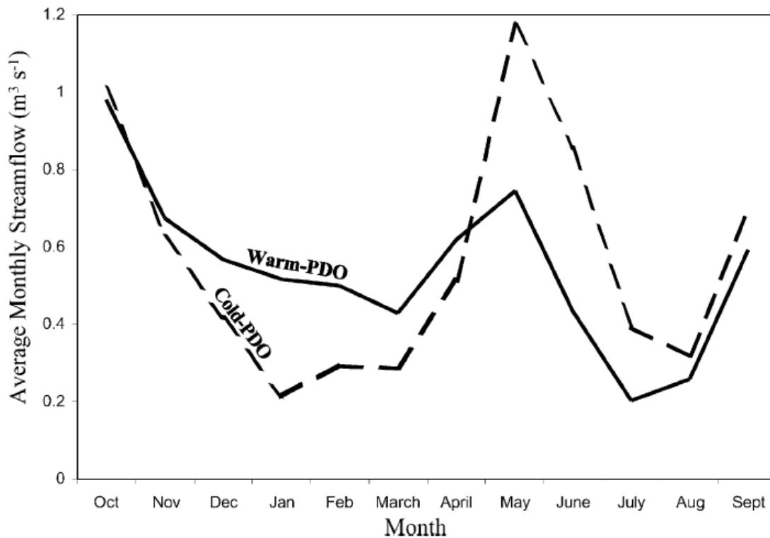
Figure 50. Annual streamflow patterns for the Kadashan River near Tenakee, Alaska during warm and cold periods of the Pacific Decadal Oscillation (Neal et al., 2002). Warm PDO years are associated with an increase in winter streamflow and a decrease in summer streamflow.
