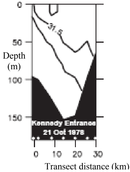
Figure 4. Cross-shelf transect at Kennedy Entrance Demonstrating shelf structure of salinity (psu) during October 1978. Contours are in 0.5 unit increments (Stabeno et al., 2004).
