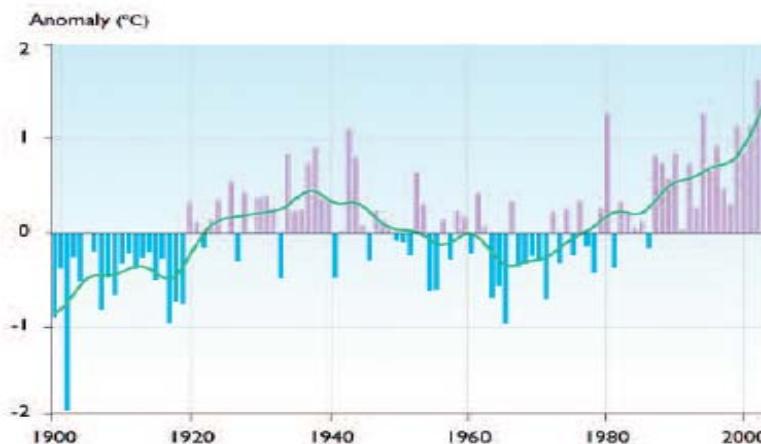
Figure 49. Annual anomalies of land-surface air temperature in the Arctic (60° to 90° N) for the period 1900 to 2003. From the Arctic Climate Impact Assessment (ACIA [300 authors], 2006).
