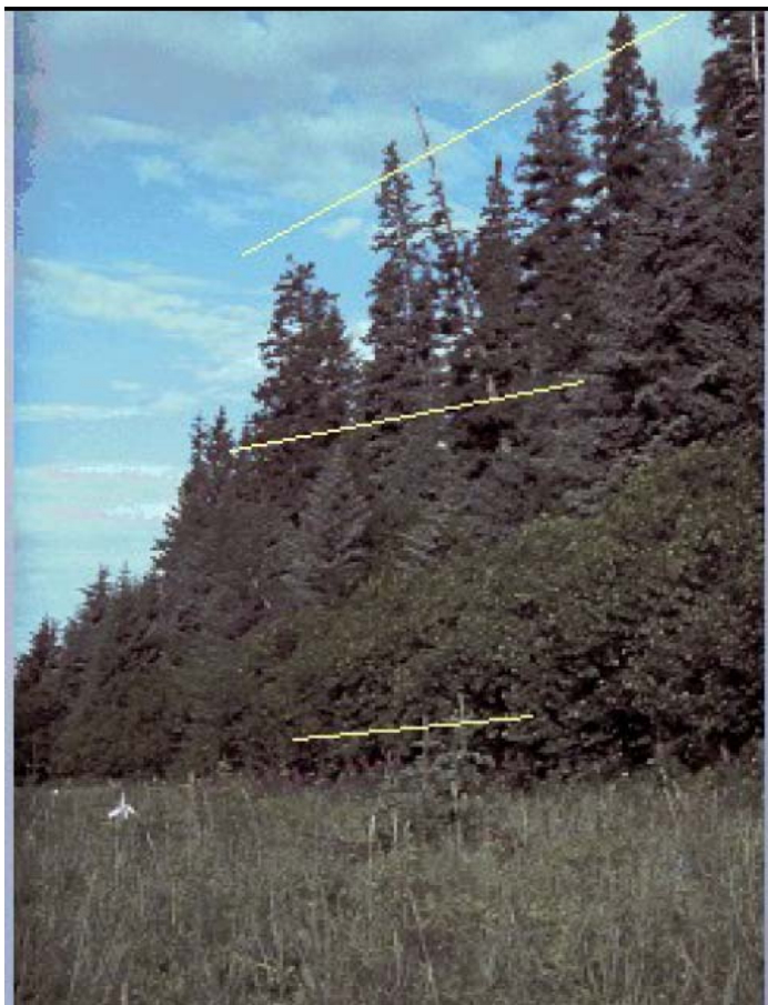
Figure 56. Terraced age layers of young sitka spruce along the LACL coast. Uplift of the land is causing loss of salt marshes and sequential transitions into Sitka spruce forest. Photo courtesy of Page Spencer, NPS, 2007.
