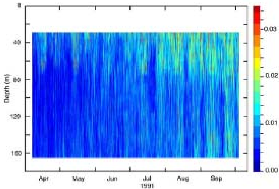
Figure 5. Vertical shear ( s^{-1} ), which is a reflection of current speed, at Kennedy Entrance from Acoustic Doppler Current Profiler. Blue indicates low shear and warmer colors indicate higher shear. Note that the highest shears are observed in the top 80 m of the water column and that shear is higher in the fall compared to the spring and summer (Stabeno et al., 2004).
