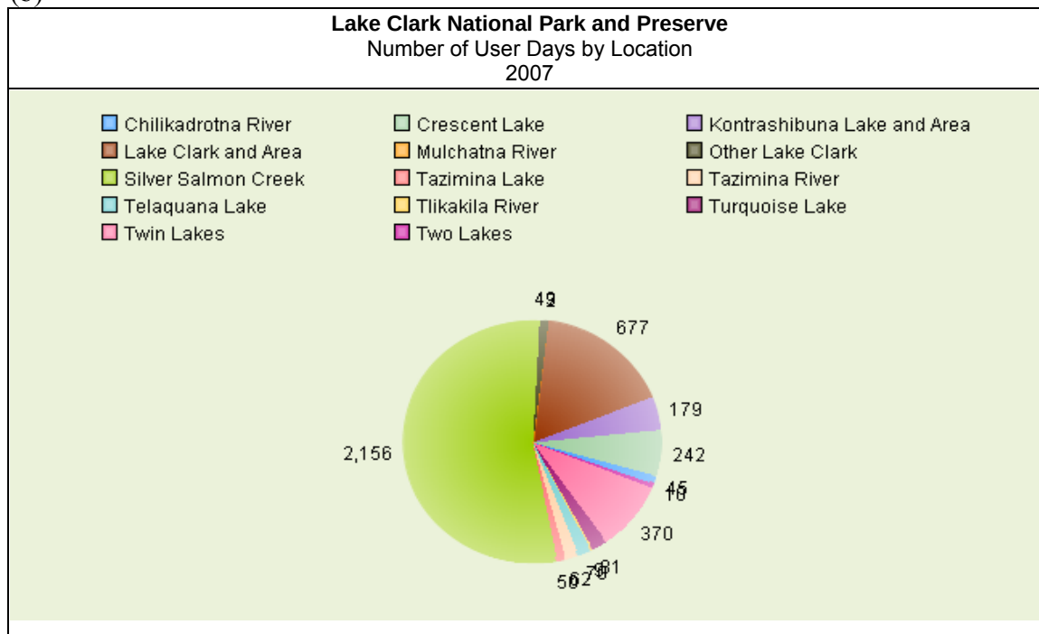
Figure 57. Pie charts showing commercial use data by (a) activity and (b) location at LACL for 2007, the most recent year for which data are available. Source: http://science.nature.nps.gov/im/units/swan/vs/hum_visit_use/cua_index.cfm?theme=cua_location_park_activity&park_code=LACL&year=2007
