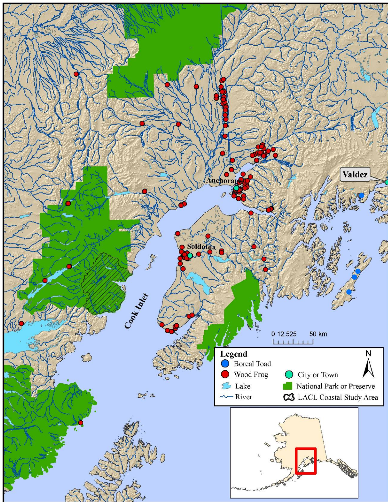
Figure 31. Location of amphibian reports in Southcentral Alaska. (Source: Alaska Natural Heritage Program).
