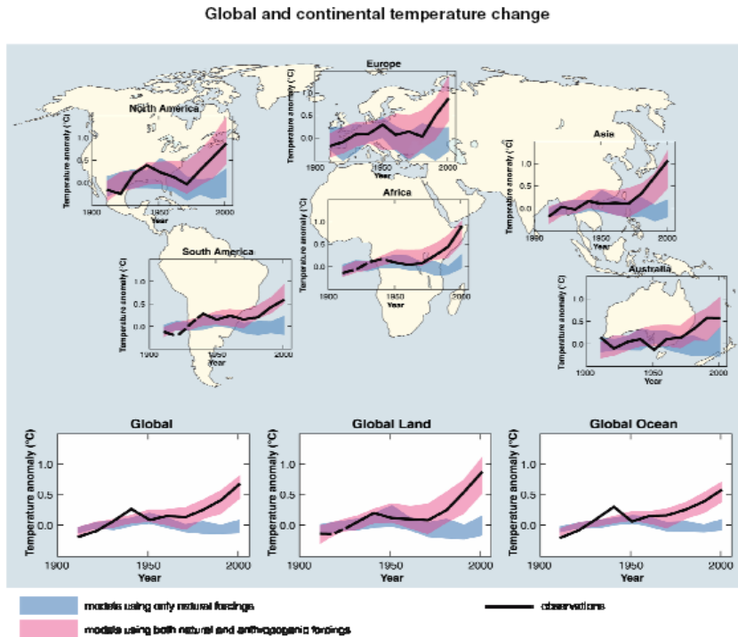
Figure 48. Comparison of observed continental- and global-scale changes in surface temperature with results simulated by climate models using either natural or both natural and anthropogenic forcings. Decadal averages of observations are shown for the period 1906-2005 (black line) plotted against the centre of the decade and relative to the corresponding average for the period 1901-1950. Lines are dashed where spatial coverage is less than 50%. Blue shaded bands show the 5-95% range for 19 simulations from five climate models using only the natural forcings due to solar activity and volcanoes. Red shaded bands show the 5-95% range for 58 simulations from 14 climate models using both natural and anthropogenic forcings (IPCC, 2007).
