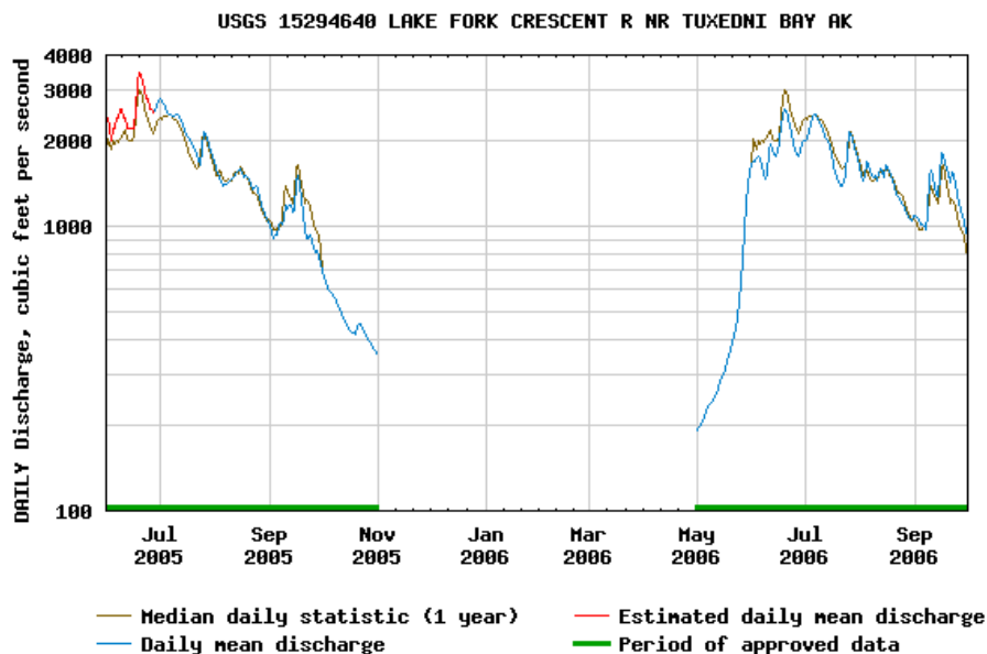
Figure 16. Discharge on the Lake Fork of the Crescent River (USGS gage site number 15294640) from June 2005 - September 2006. Source: USGS Alaska Science Center.
