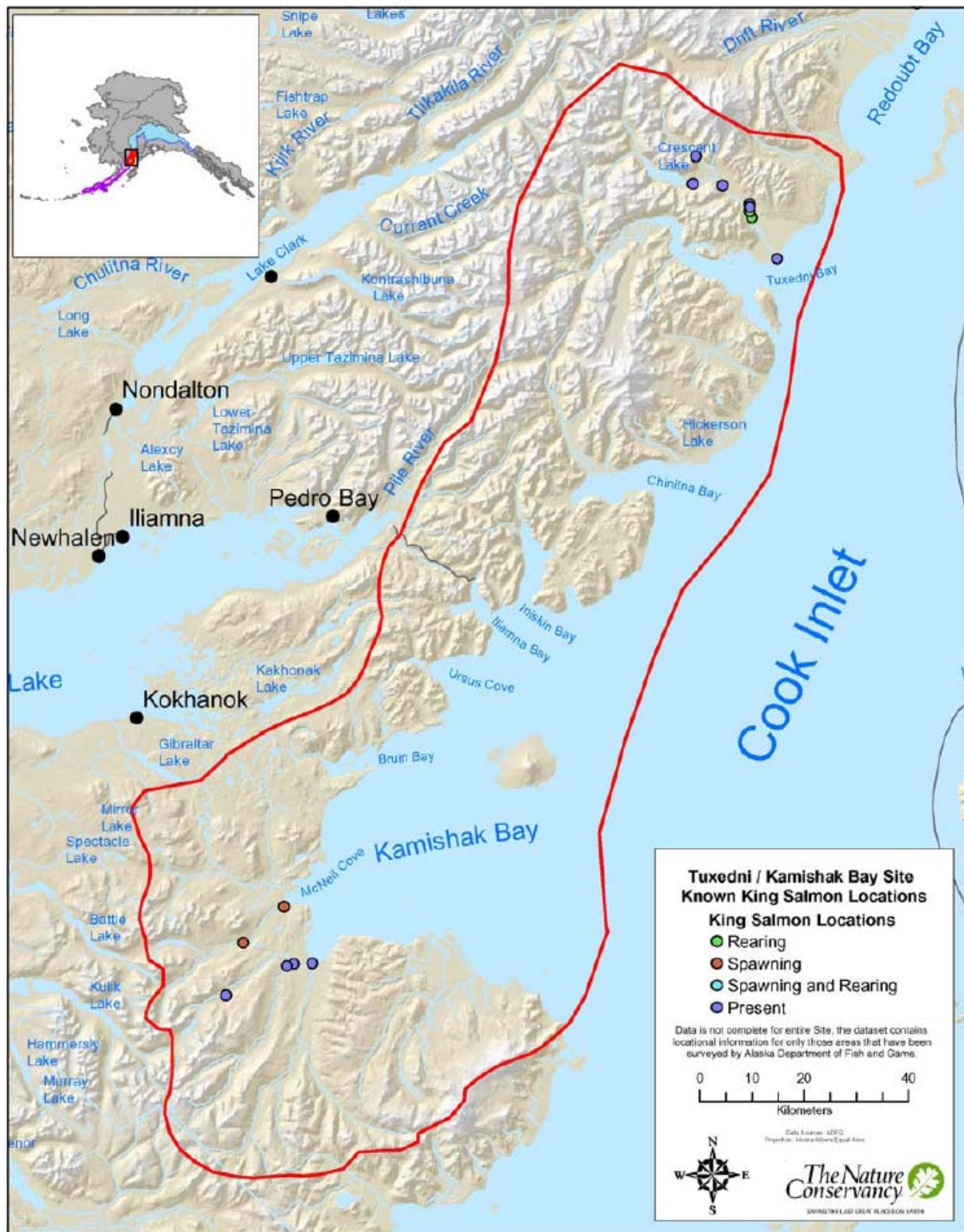
Figure 28. King salmon rearing and spawning habitats and presence (Witten, 2003).
