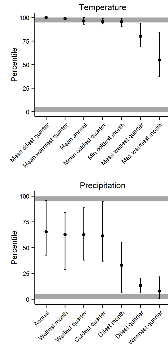
Figure 2. Recent temperature and precipitation percentiles at Lava Beds National Monument (including areas within 30-km [18.6-mi] of the park’s boundary). Black dots indicate average recent percentiles across the 10, 20, and 30-year intervals (moving windows). Variables are considered “extreme” if the mean percentiles are <5 th percentile or >95 th percentile (i.e., the gray zones, where recent climate is pushing the limits of all observed climates since the year 1901). Black bars indicate the range of recent percentiles across 10, 20, and 30-year moving windows (larger bars indicate higher sensitivity to moving window size).
