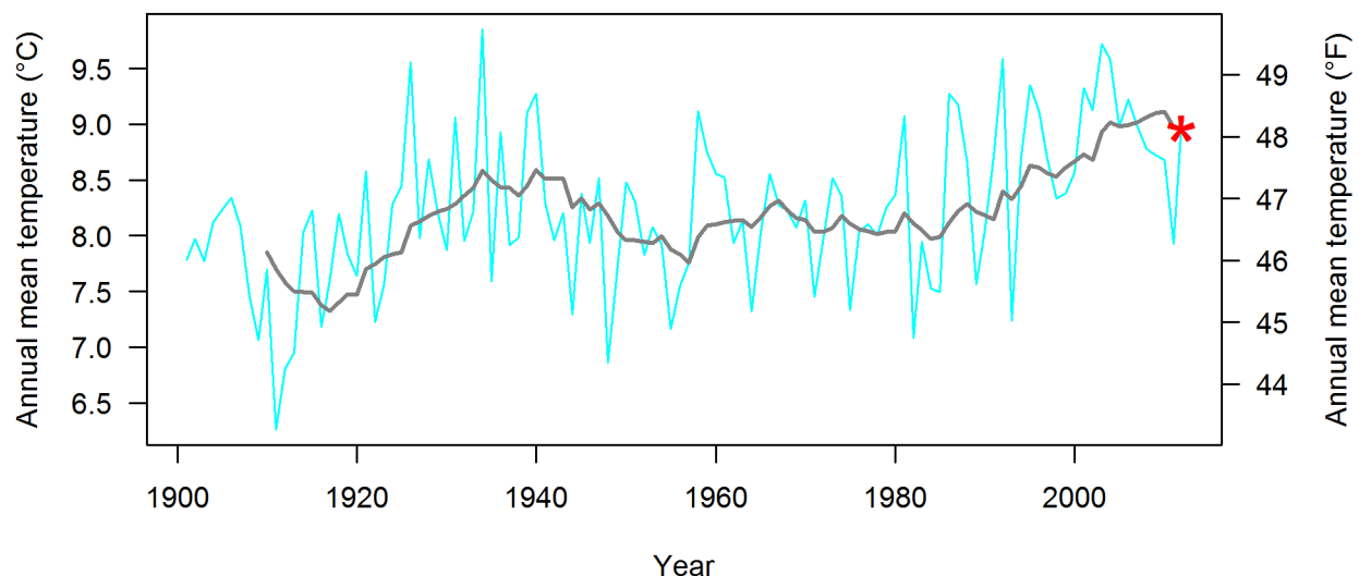
Figure 1. Time series used to characterize the historical range of variability and most recent percentile for annual mean temperature at Lava Beds National Monument (including areas within 30-km [18.6-mi] of the park’s boundary). The blue line shows temperature for each year, the gray line shows temperature averaged over progressive 10-year intervals (10-year moving windows), and the red asterisk shows the average temperature of the most recent 10-year moving window (2003–2012). The most recent percentile is calculated as the percentage of values on the gray line that fall below the red asterisk (see results of most recent percentiles for all temperature and precipitation variables in Figure 2).
