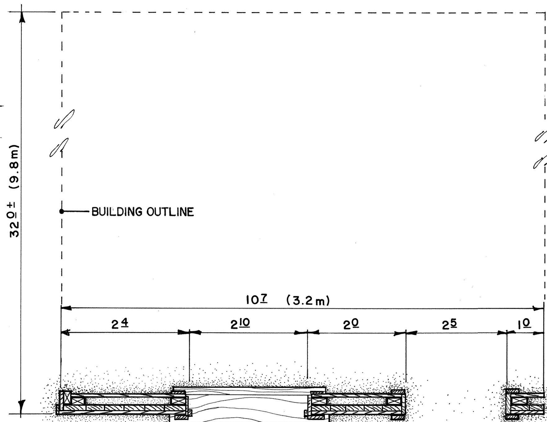
FLOOR PLAN SCALE: \frac{3}{4}'' = 1'-0'' ft 10 m 3.0
