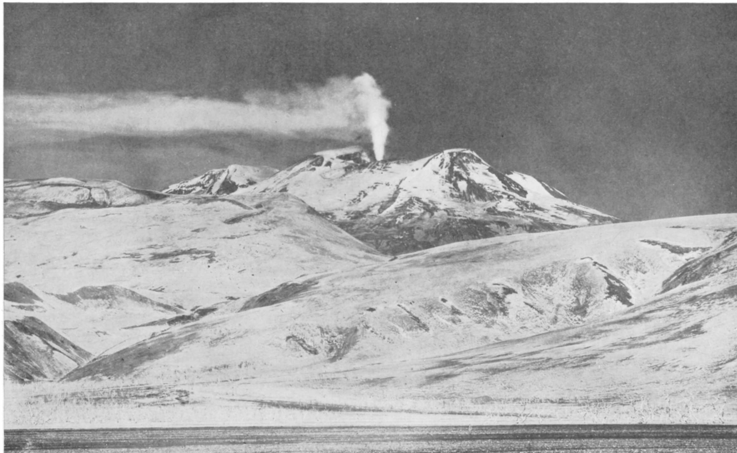
MOUNT MAGEIK FROM KATMAI VALLEY Before the eruption Katmai must have looked much like this.
