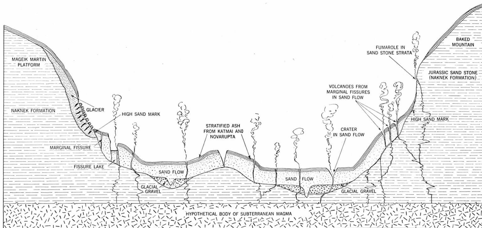
A GENERALIZED SECTION OF THE VALLEY OF TEN THOUSAND SMOKES
