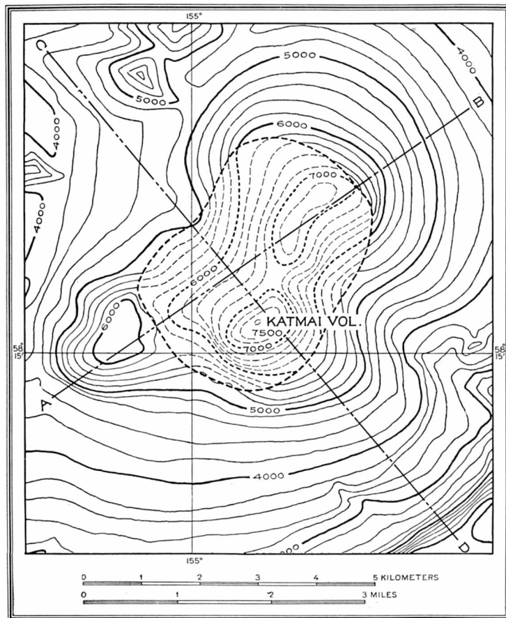
A RECONSTRUCTION OF MOUNT KATMAI AS IT WAS BEFORE THE ERUPTION
