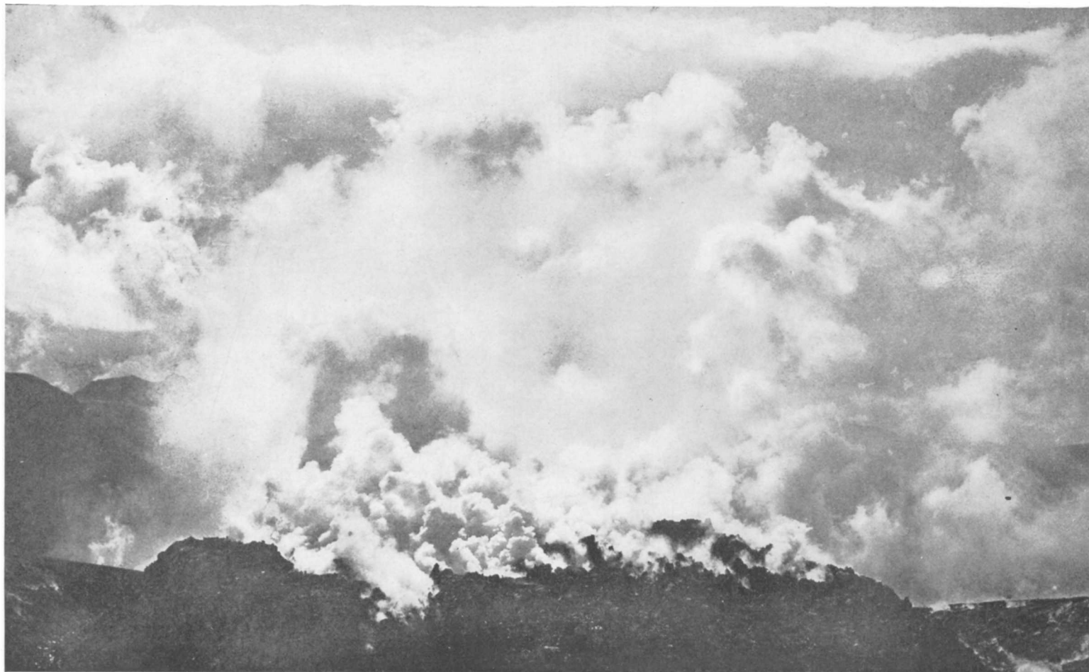
STEAM FROM THE LAVA PLUG OF NOVARUPTA, 1917
