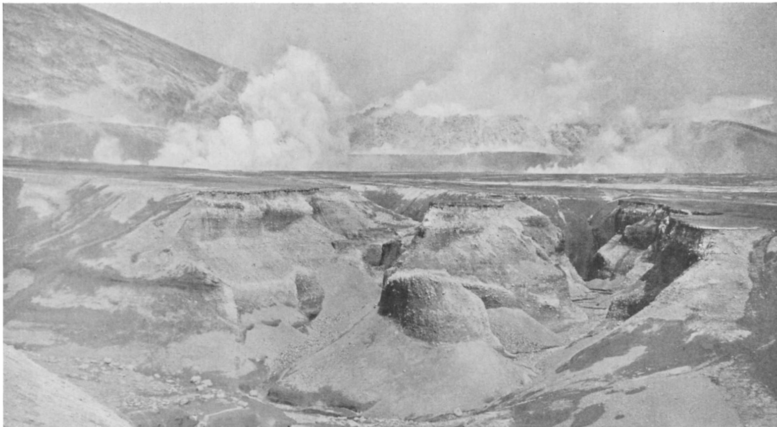
BAD LANDS CUT BY GULLIES, IN THE ASH DEPOSITS NEAR NOVARUPTA
