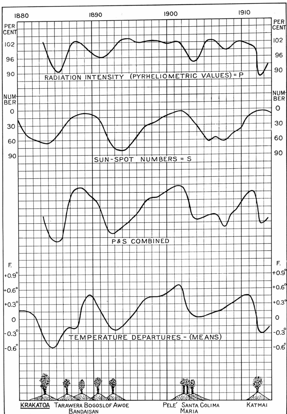
CURVES SHOWING THE RELATIONS OF TEMPERATURE, SUNSPOT NUMBERS AND RADIATION INTENSITY (PYRHELIOMETRIC VALUES) AS AFFECTED BY VOLCANIC ERUPTIONS (After Humphreys.)
