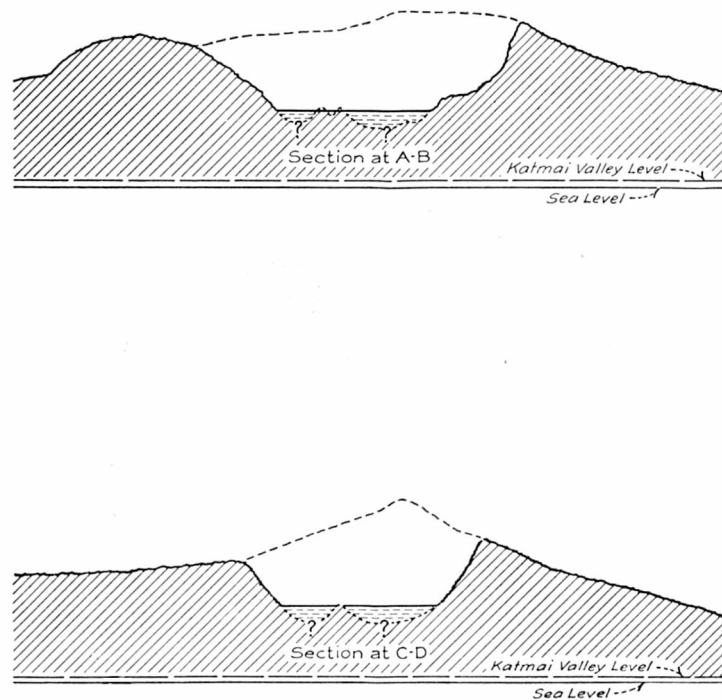
SECTIONS OF MOUNT KATMAI BEFORE AND AFTER THE ERUPTION
