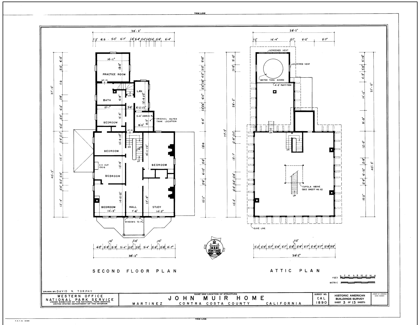
Figure 6: Strentzel-Muir House floor plan, second floor and attic. Historic American Buildings Survey Collection, HABS CA-1890.
