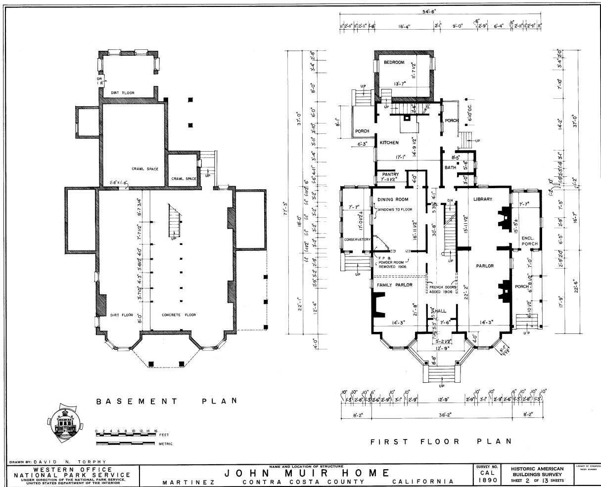
Figure 5: Strentzel-Muir House floor plan, basement and first floor. Historic American Buildings Survey Collection, HABS CA-1890.
