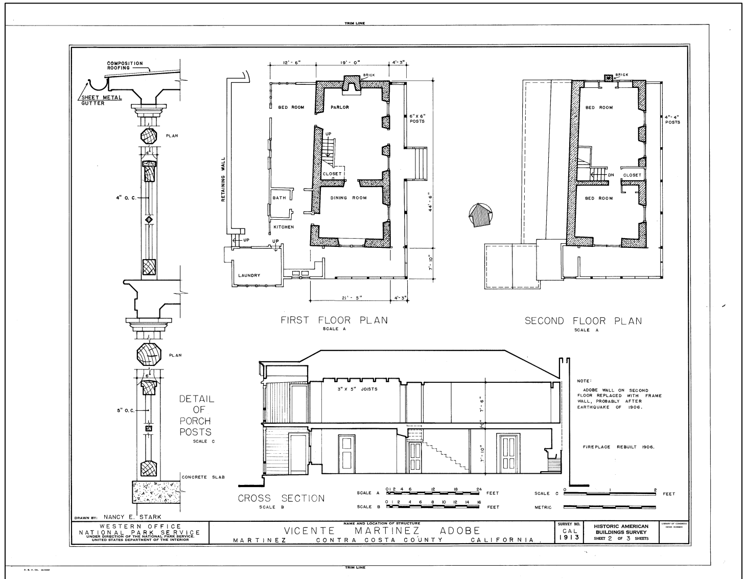
Figure 7: Martinez Adobe floor plan, cross section, and detail of porch posts. Historic American Buildings Survey Collection, HABS CA-1913.
