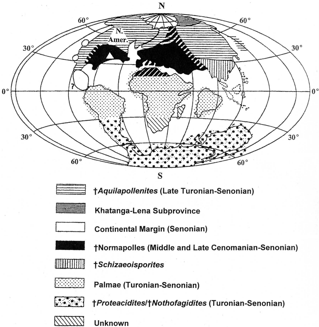
Figure 3. Late Cretaceous palynofloral provinces of the world. Open triangle shows approximate location of Kentucky in the †Normapolles Palynofloral Province (from Herngreen et al., 1996: 1162, with permission for re-use from the American Association of Stratigraphic Palynologists Foundation, Dallas, Texas, < www.schweizerbart.de >).
