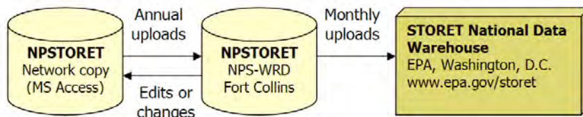
Figure 6.9.1. Data flow diagram for water quality data.
