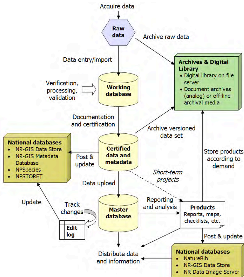
Figure 6.8.1. Diagram of project data life cycle.
