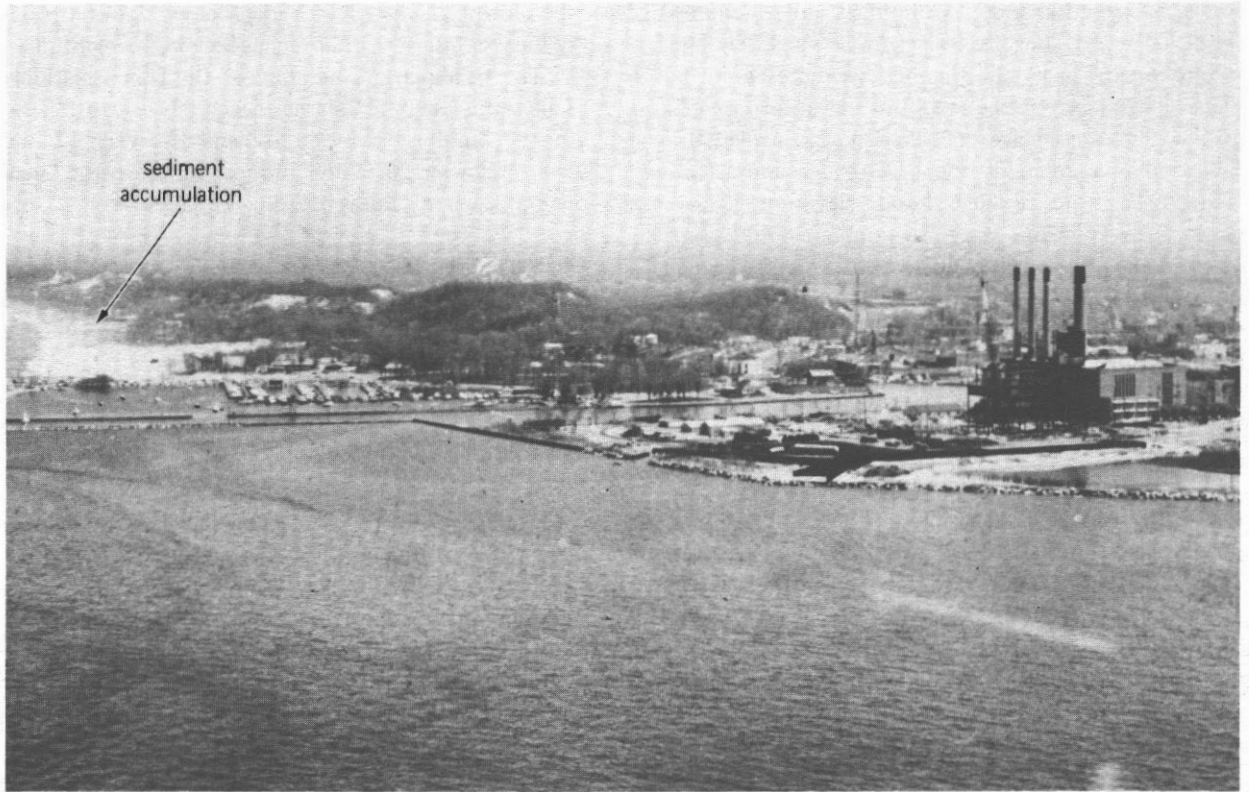
Figure 4. Sediments borne by longshore currents trapped on the up-current side of the groyne at Michigan City harbor.
