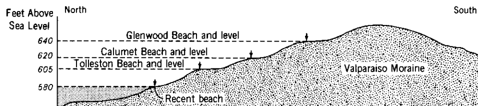
Figure 2. Cross section illustrating the three major beaches and corresponding levels of glacial Lake Chicago.
