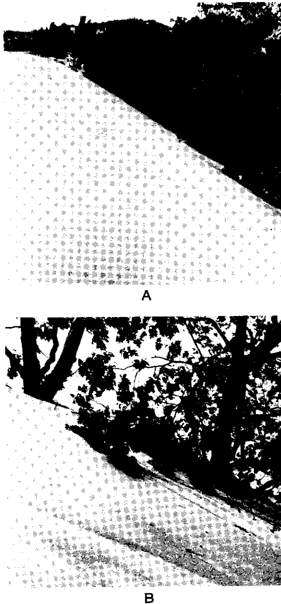
Figure 10. Migrating sand burying a living forest at West Beach. A , View of encroaching dune from crest. B , View of lee slope of the same dune midway between its base and crest.
