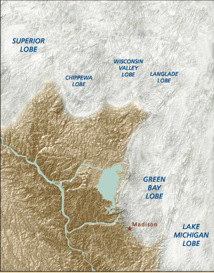
Glacial Lobes of the Wisconsin Glaciation
