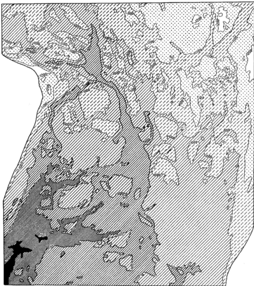
FIG. 20—Hypsometric map of a part of Drumheller Channels. Distribution of higher and lower tracts is more graphically shown than by the intricate and unusual contour pattern of the map, Figure 21. The contour interval is 100 feet. The highest areas (blank) are over 1200 feet; the lowest (solid black) less than 700 feet A.T. Comparison with Figure 19 will show the location of several of the largest (including the deepest) rock basins and many of the channels on the higher part of the scabland plexus.
