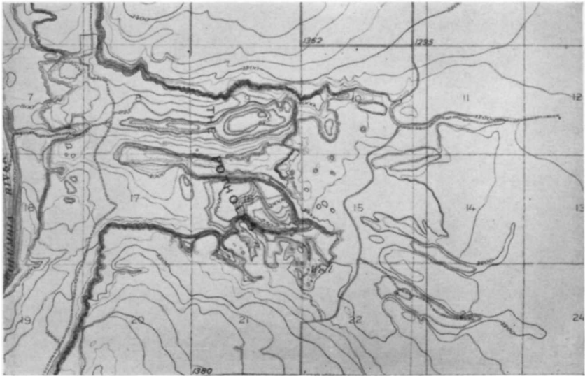
FIG. 18—Potholes Cataract, one of three cataract spillways from the west side of Quincy Basin. (From Quincy sheet, U. S. Geological Survey.)
