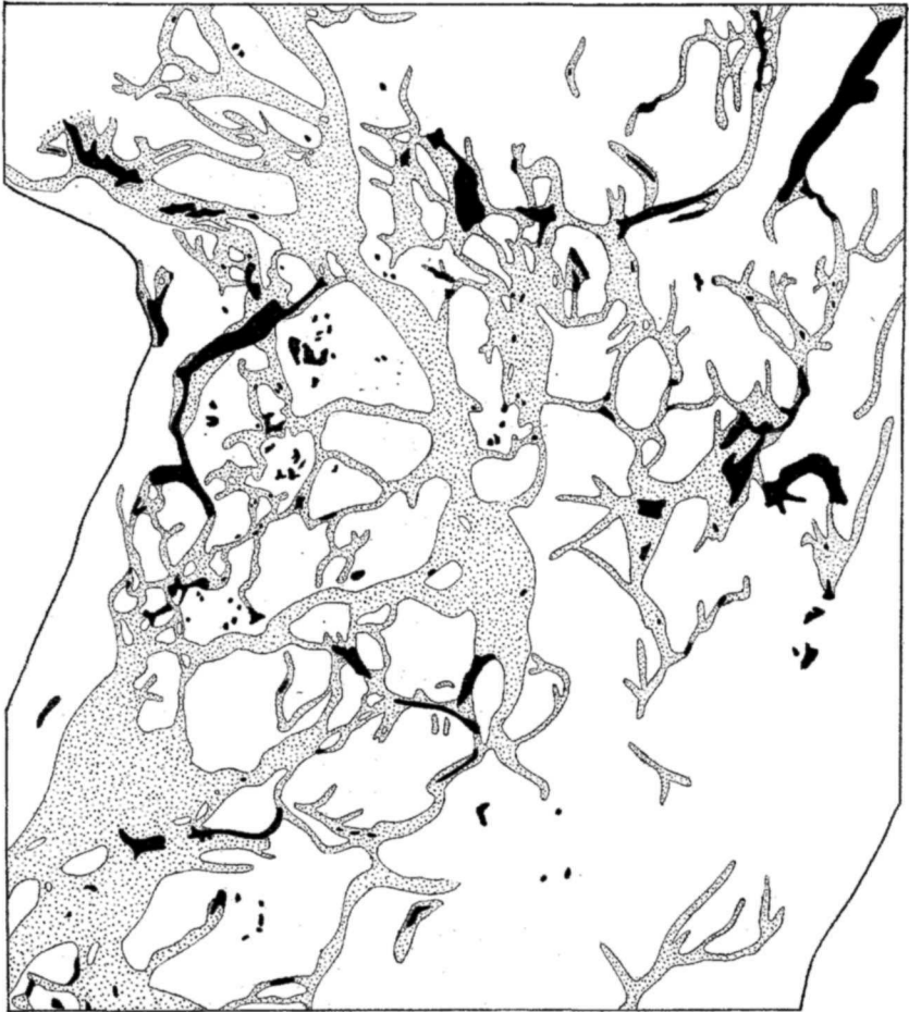
FIG. 19.—Channels, rock basins, buttes, and general scabland of a part of the Drumheller Channels. Rock basins black, channels stippled, buttes and general scabland blank. The beginning and ending of many channels in the plexus is better shown here than on the contour map, Figure 21, as also is the extreme irregularity of the channel pattern. The larger rock basins are notably linear and are largely in channels. It must be understood, however, that the highest scabland is itself channel floor of the great spillway. Scale approximately 1:120,000, slightly more than half an inch to a mile.
