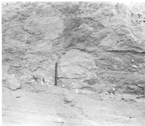
Figure 9.4. Sand block above silt block at same horizon as the granitic erratic in Fig. 9.3. The blocks may have been frozen during transport.
