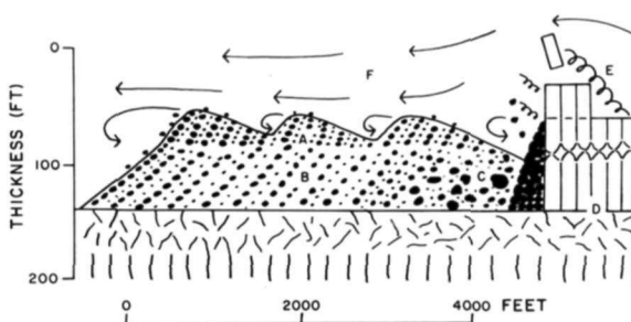
Figure 5.17. Schematic development of a hypothetical pendant bar. Bedload is transported across the surface of the bar by giant ripples and deposited at the downstream end of the bar. Explanation: A—foreset bedding associated with giant current ripples, B—foreset bedding within the bar, C—chaotically deposited flood gravel, D—basalt bedrock, E—erosion of basalt columns by kolks, F—flow directions.
