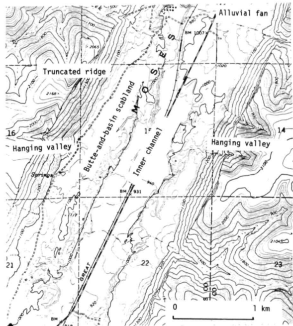
Figure 5.28. Topographic map of lower Moses Coulee showing the relationships discussed in Fig. 5.27. The contour interval is 10 feet (elevations in feet).
