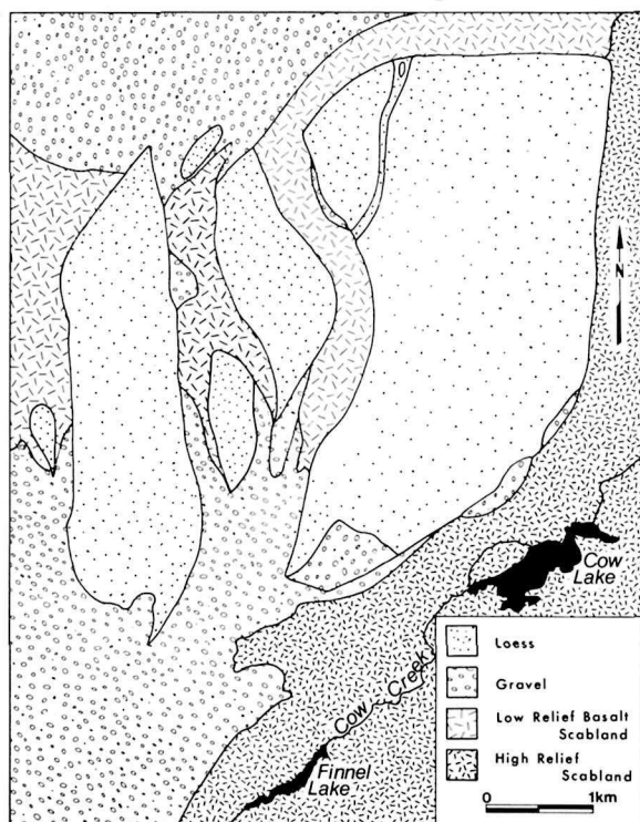
Figure 6.8. Map of the Karakul Hills loess islands.
