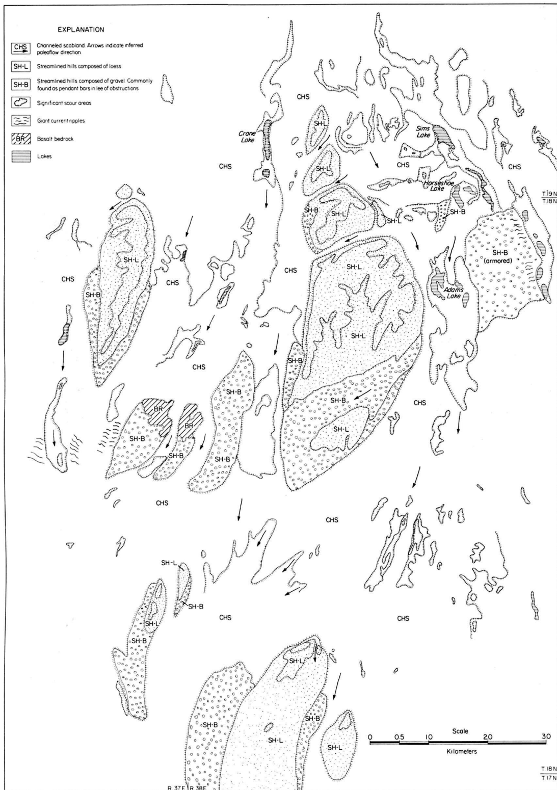
Figure 6.7. Geomorphic map of the Macall area in the central Cheney-Palouse tract.
