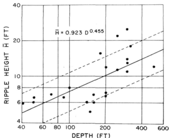
Figure 5.44. Logarithmic regression of ripple height as a function of depth. The dashed lines represent one standard error.
