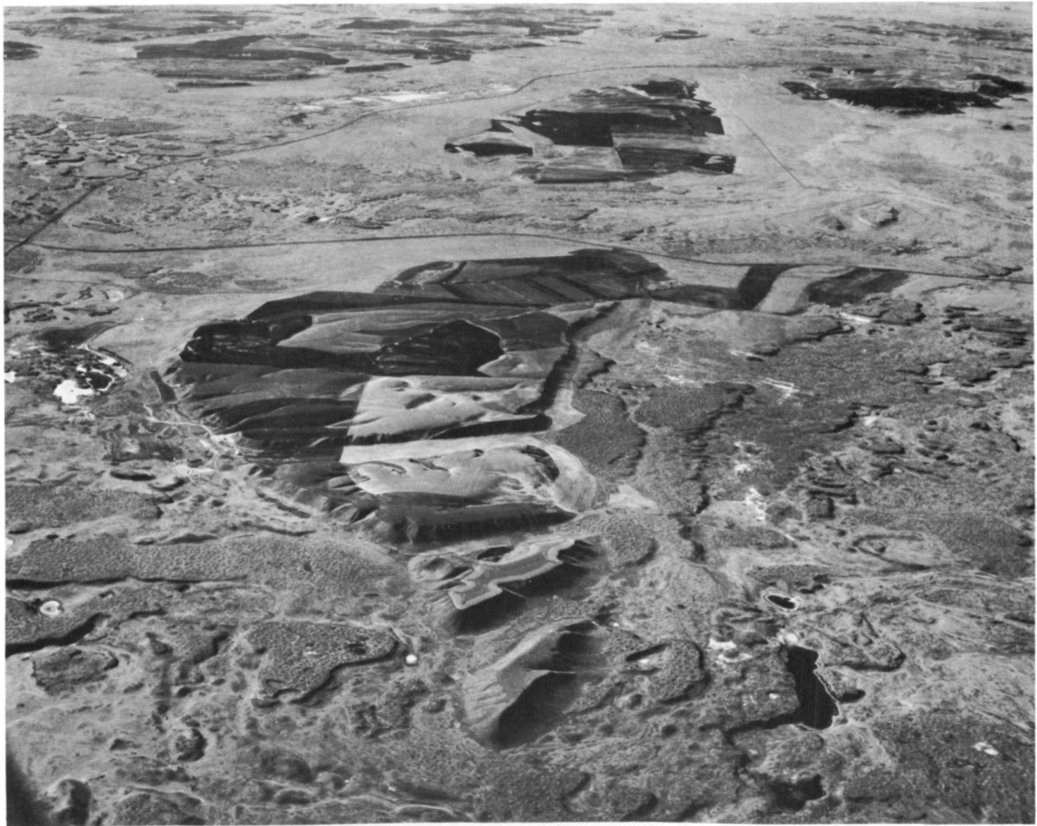
Figure 7.8. Oblique aerial view toward the south of the Macall area. See maps in Fig. 7.6 for location (photograph 6235 by John S. Shelton).
