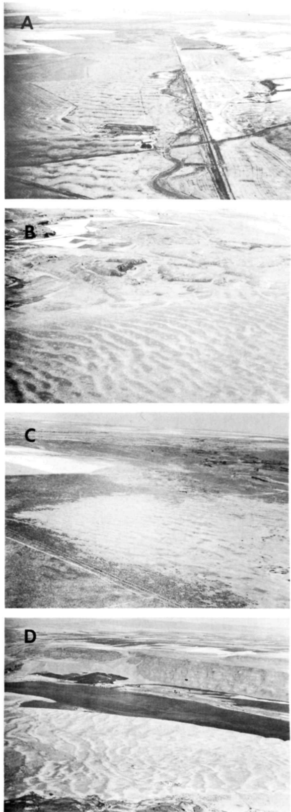
Figure 5.34. Typical sets of giant current ripples in the Channeled Scabland: A. Lind Coulee, B. Marlin, C. Artesian Lake, D. West Bar. Locations for these ripple trains are given in Baker (1973a).
