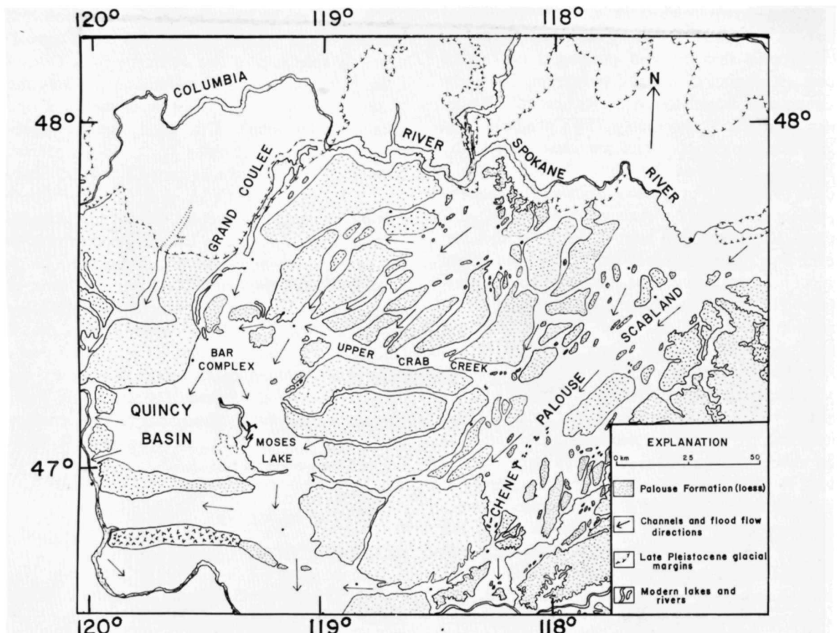
Figure 2.1. Map of the Channeled Scabland in eastern Washington showing the distribution of channels and the
