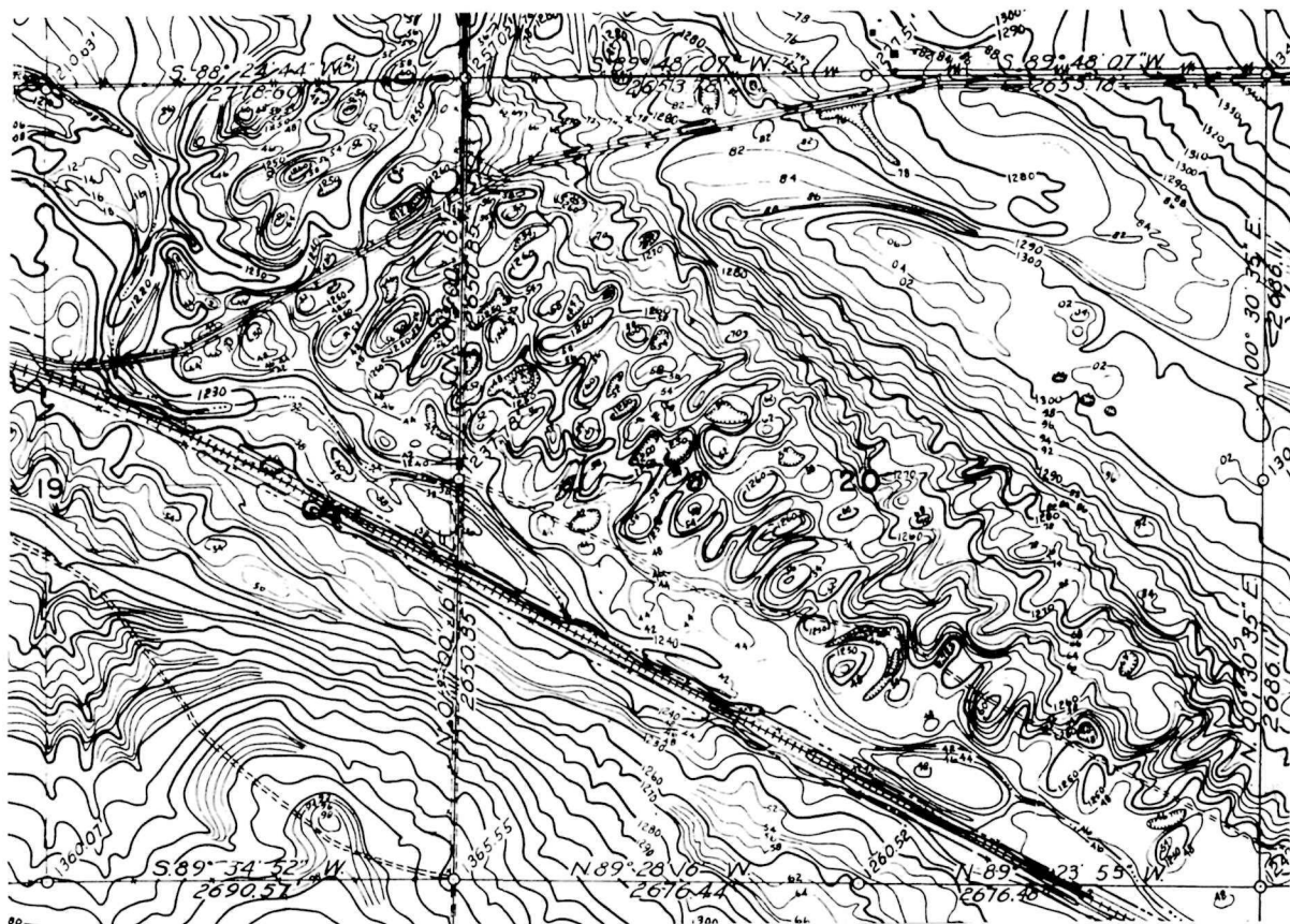
Figure 7.23. Part of U.S. Bureau of Reclamation topographic map of the Columbia Basin Project. The 2-foot contour interval provides an excellent display of the
