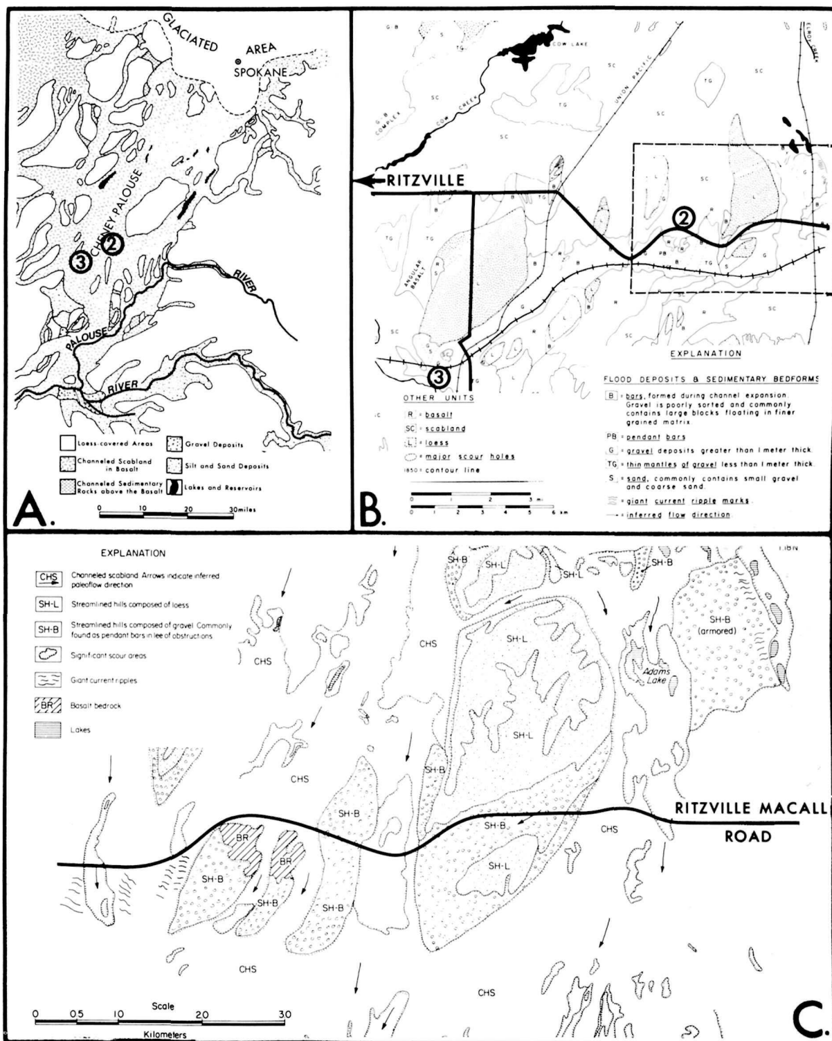
Figure 7.6. Morphological maps of the Ritzville-Macall road traverse across the Cheney-Palouse scabland tract. A is a part of Fig. 7.1 for location. B identifies the setting of Stops 2 and 3 relative to bars and loess hills
