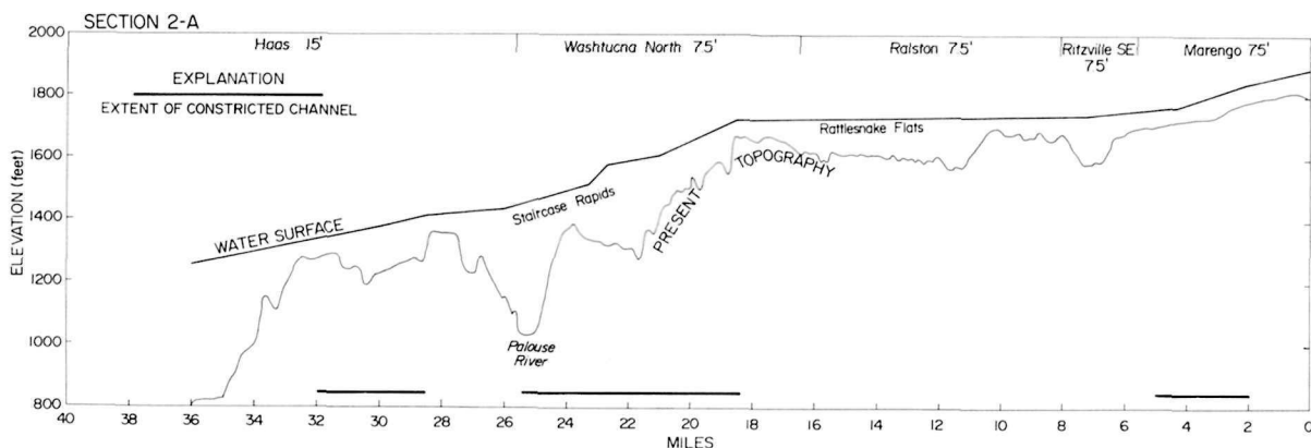
Figure 6.4. Profile 2-A through the western part of the Cheney-Palouse tract (see Fig. 6.1 for location). Note
