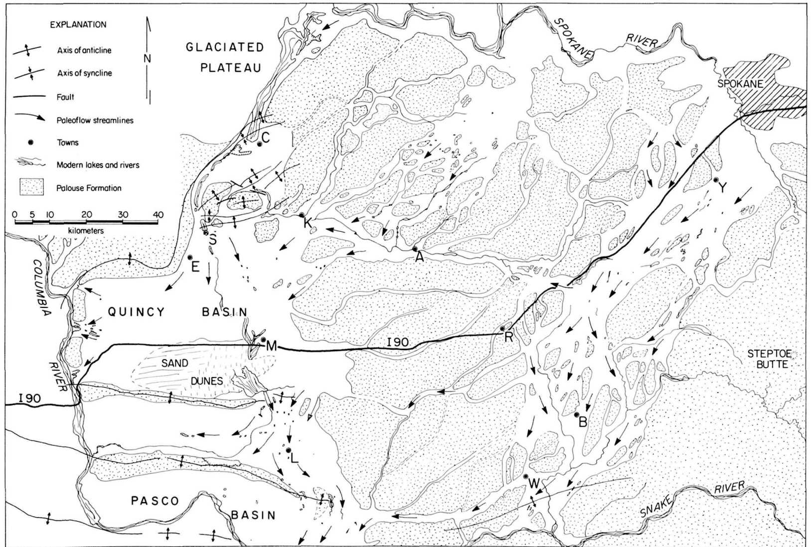
Figure 5.2. Regional pattern of the Channeled Scabland as mapped from LANDSAT imagery (E-1039-1843-5 and E-1004-18201-7). (Y) Cheney, (R) Ritzville, (B) Benge, (W) Washtucna, (M) Moses Lake, (E) Ephrata, (S) Soap Lake, (C) Coulee City.
