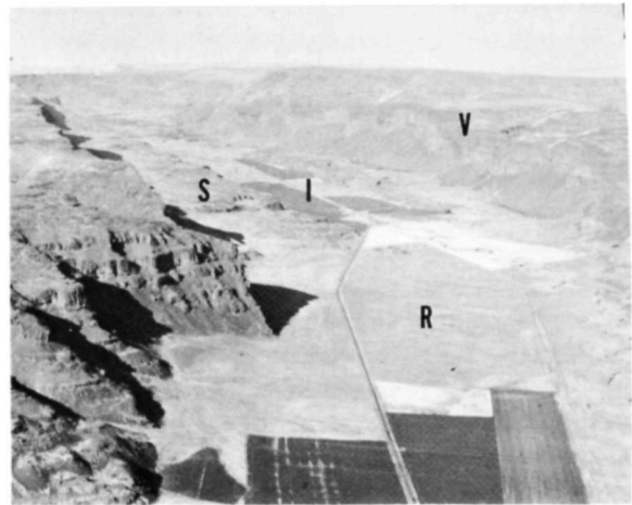
Figure 5.27. Inner channel development in Moses Coulee. This oblique aerial photograph shows a distinct inner channel (I) on the coulee floor with marginal butte-and-basin scabland (S). Giant current ripples (R) occur on the surface of a flood gravel bar at the mouth of the inner channel. Preflood tributaries to the drainage were truncated by flood erosion to form hanging valleys (V) separated by truncated spurs.
