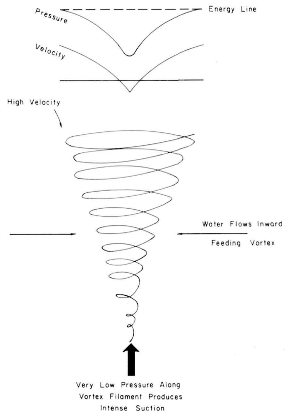
Figure 4.20. Characteristics of a hydraulic vortex ("kolk"). Such macroturbulent effects are set up by flow obstructions. The intense pressure and velocity gradients of the vortex produce a hydraulic lift. Alternatively, Jackson (1976) ascribes "kolks" to the turbulent bursting phenomenon.
