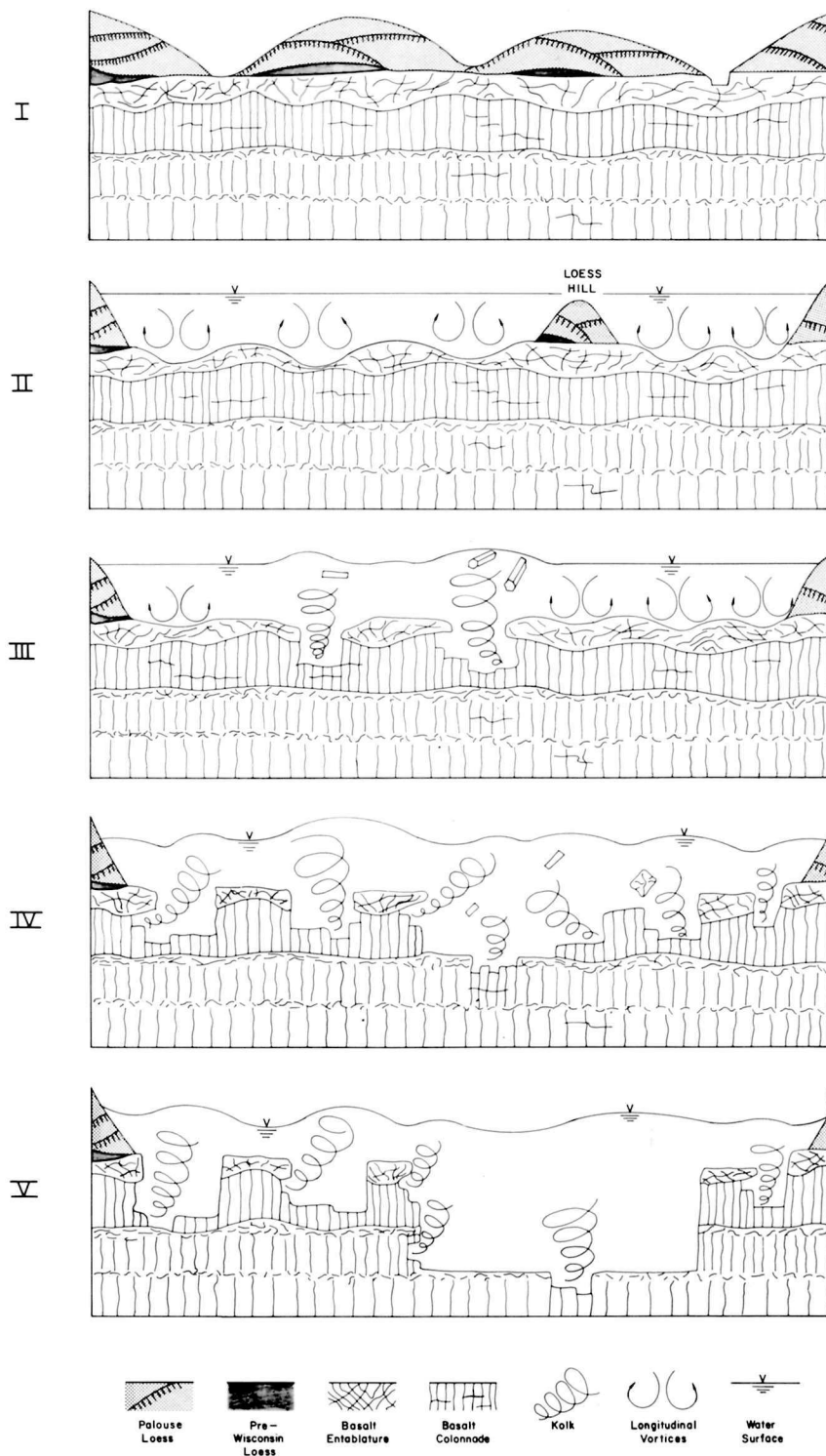
Figure 5.32. Hypothetical sequence of flood erosion for a typical scabland divide crossing. See text for discussion.
