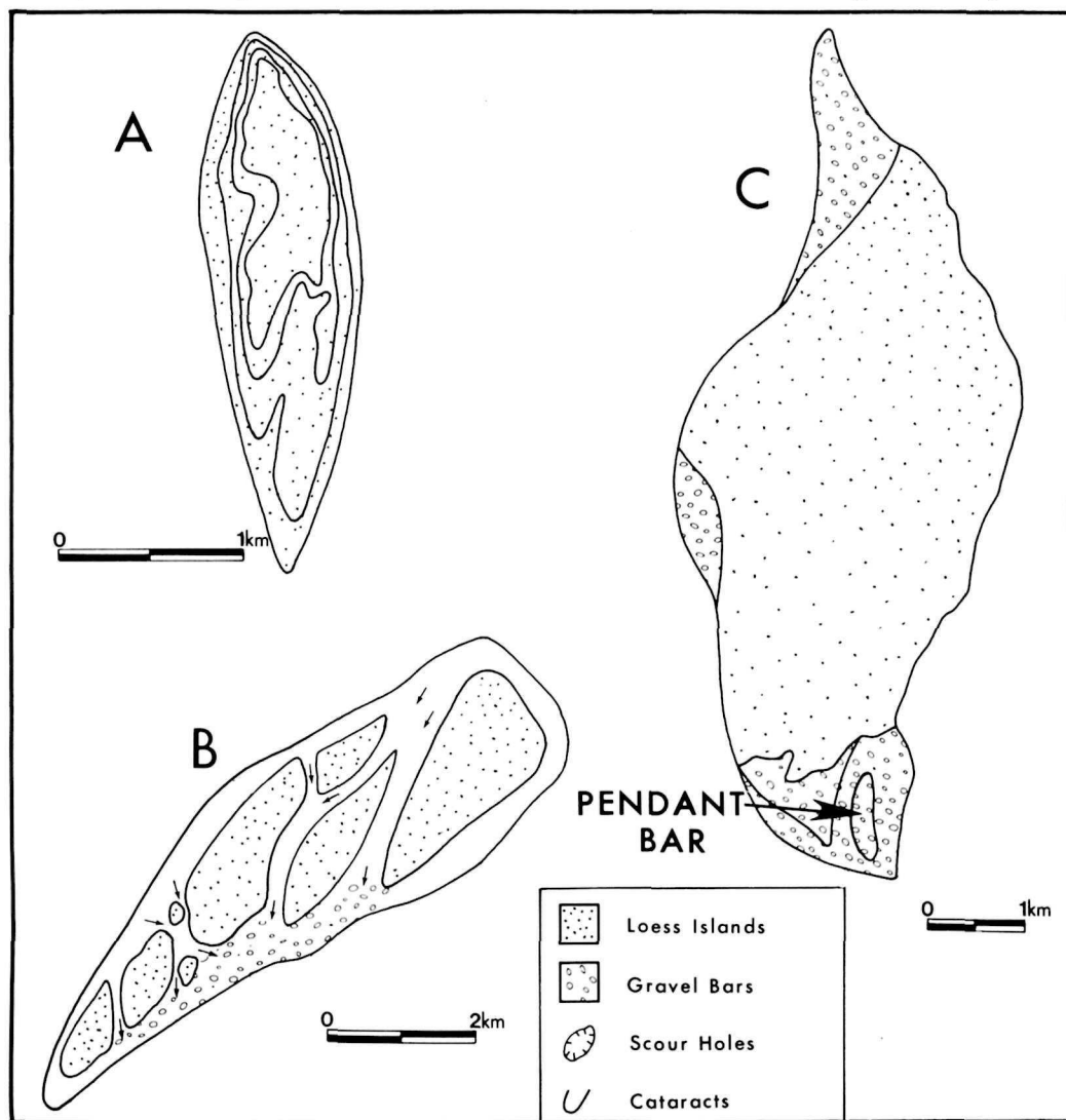
Figure 6.5. Loess island forms in the Cheney-Palouse scabland tract illustrating the three major morphologic types. A. Subfluvially eroded loess island located in the Karakul Hills (Secs. 2, 11, and 14; T. 19N., R. 36E.). B. Partially submerged loess island near Amber Lake
