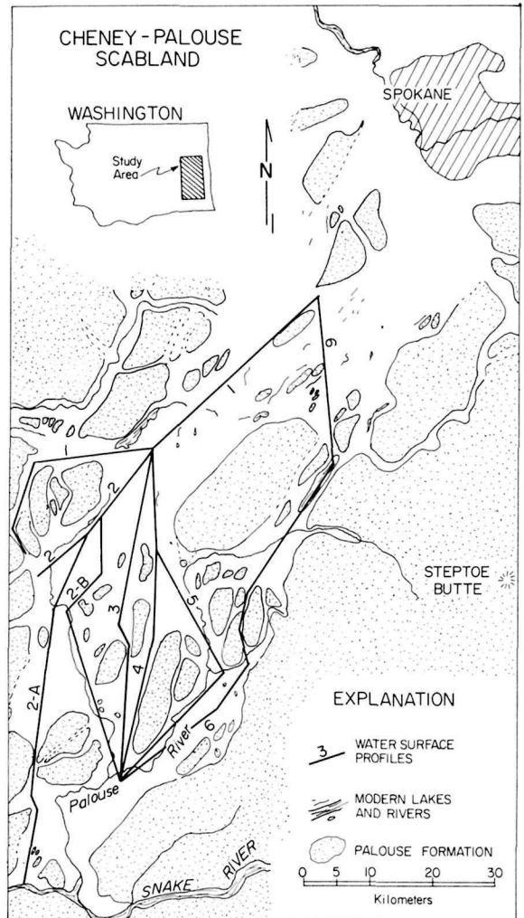
Figure 6.1. Highly generalized sketch map of the Cheney-Palouse scabland tract showing the location of various water-surface profiles that have been determined for the last major Pleistocene flood. Many of the small residual hills of Palouse Formation ("loess islands") have been omitted for simplicity.
