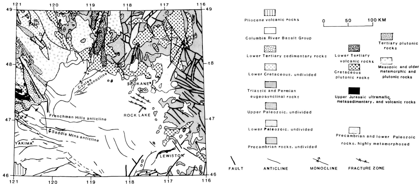
Figure 3.2. Geologic map of northern part of Columbia Plateau and surrounding area, simplified from King and Beikman (1974). Anticlinal axes, shown only on Columbia Plateau, from Newcomb (1970) with additions from Bond (1963), Griggs (1973), Swanson and others (1977), and Tabor and others (1977).
