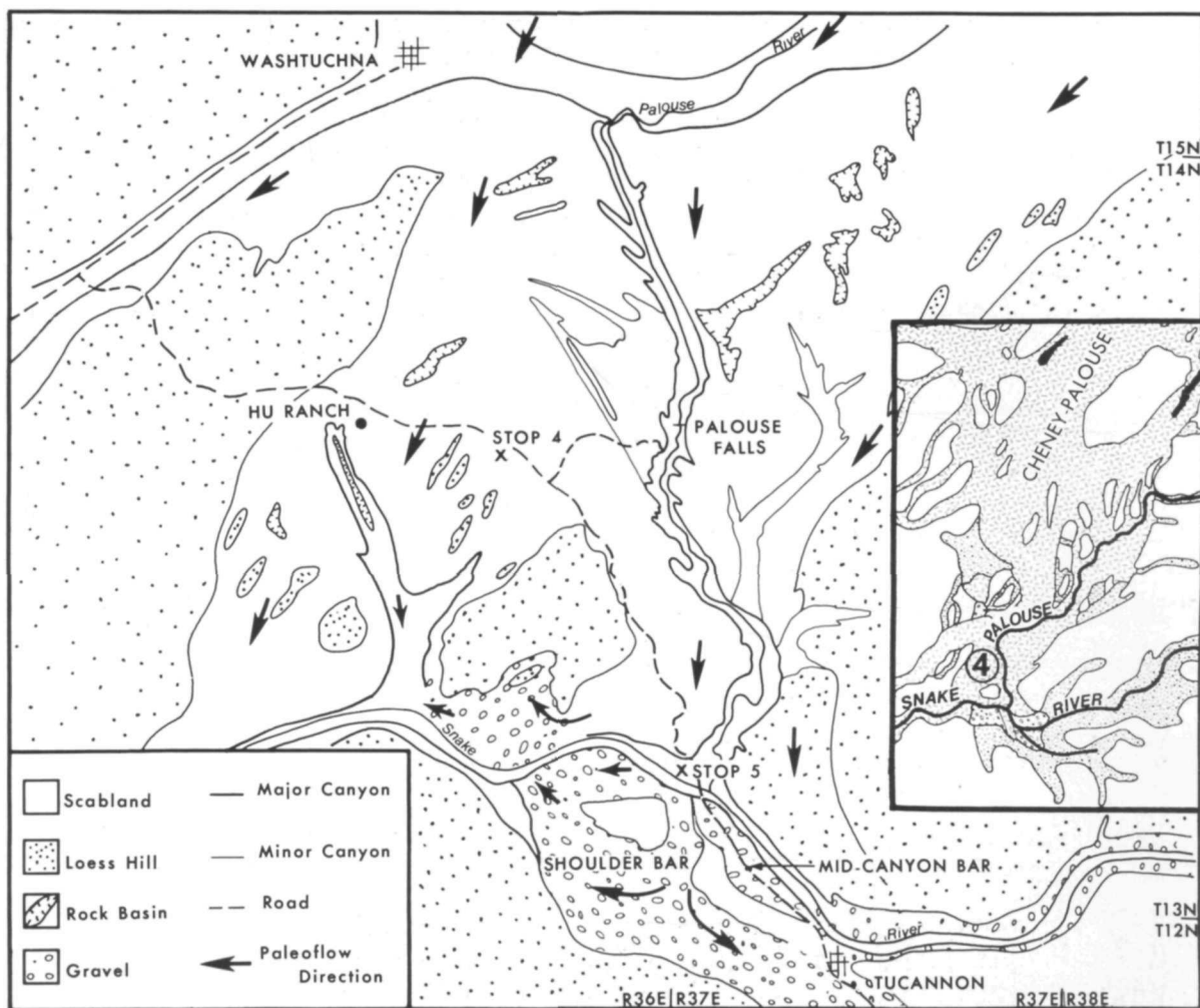
Figure 7.14. Generalized morphological map of the region surrounding the Snake-Palouse River junction. Mapped from U.S.G.S. 15' topographic maps, Starbuck
