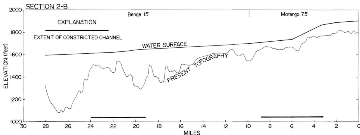
Figure 6.6. Profile 2-B along Cow Creek, a prominent inner channel of the Cheney-Palouse tract (see Fig. 6.1 for location).
