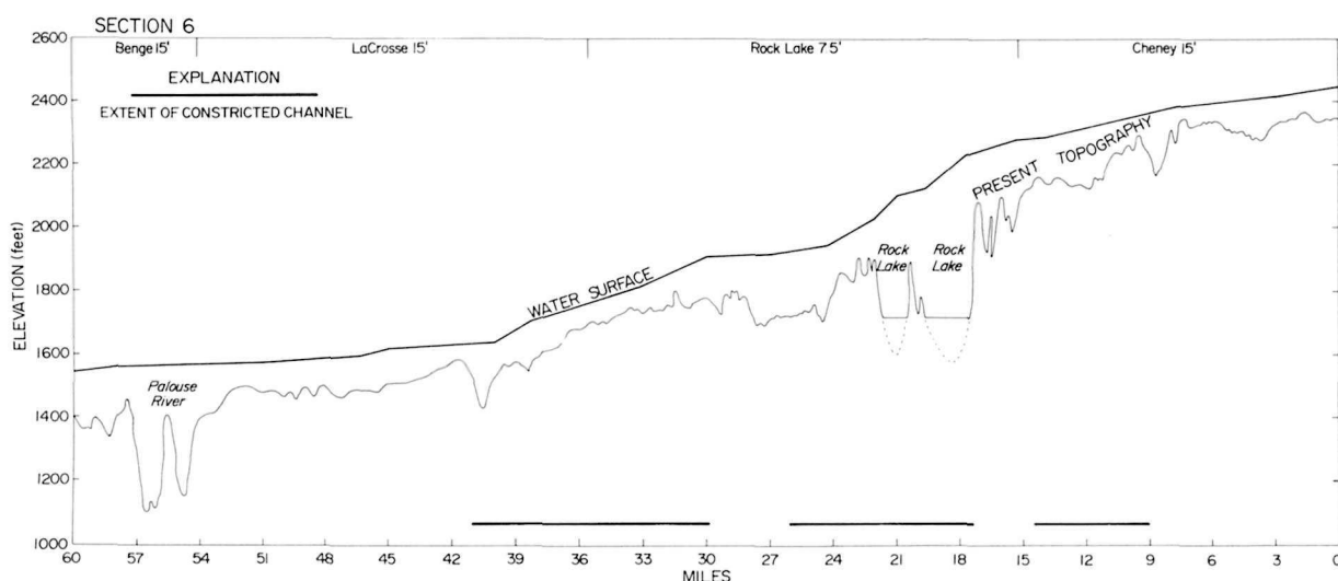
Figure 6.3. Profile 6 through the eastern part of the Cheney-Palouse tract (see Fig. 6.1 for location). Note
