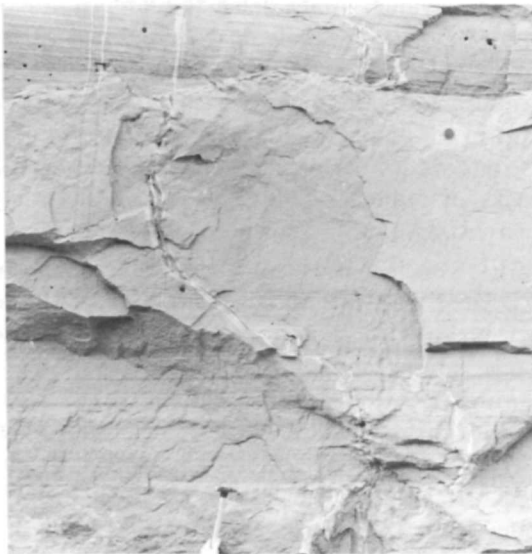
Figure 9.2. Graded beds separated by disconformities (Burlingame Canyon, 4 km south of Lowden). Each rhythmite here grades from stratified sand at the base to massive silt and clay at the top. Note the thin sinuous clastic dike.
