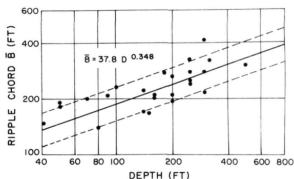
Figure 5.45. Logarithmic regression of ripple chord as a function of depth. The dashed lines represent one standard error.
