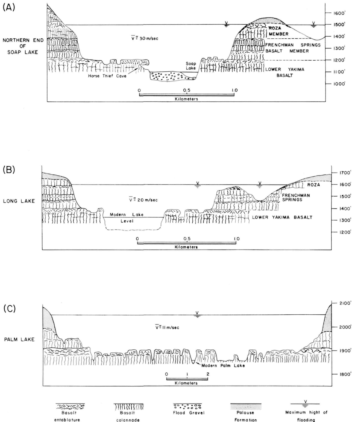
Figure 5.26. Representative cross sections of scabland channels showing structural characteristics of basalt, erosional features, and flood stage plus maximum mean flow velocity ( \bar{V} ). The sections at Soap Lake (A) and Long Lake (B) show inner channels with flanking butte-and-basin scabland topography. The section at Palm Lake (C) shows longitudinal groove topography.
