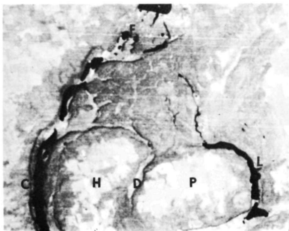
Figure 4.7. LANDSAT image of the Hartline Basin and the scabland channels leading from its southern margin: C-Lenore Canyon, D-Dry Coulee, and L-Long Lake. Other features are Dry Falls (F), High Hill (H), and Pinto Ridge (P). The scene measures 35 x 25 km. Compare to Fig. 4.6.
