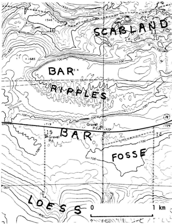
Figure 5.40. Topographic map of giant current ripples shown in Fig. 5.36.
