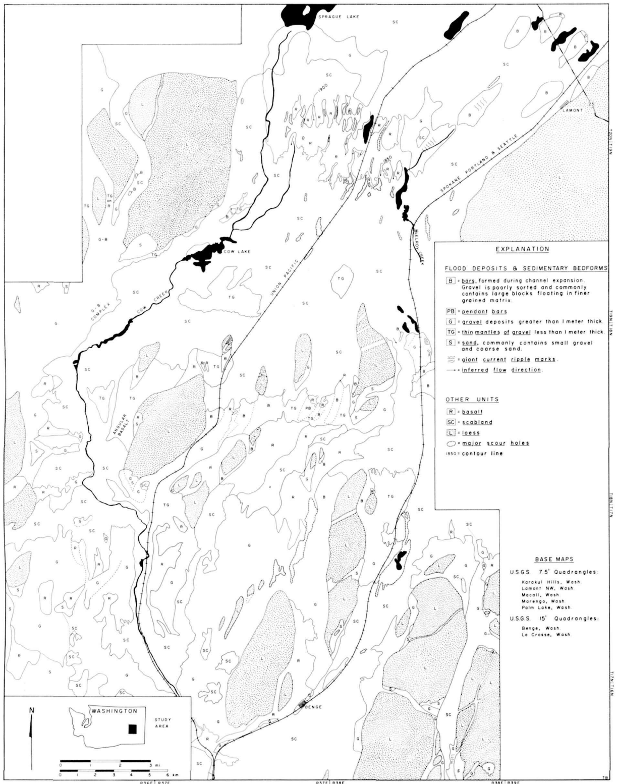
Figure 6.2. Geomorphic map of the central portion of the Cheney-Palouse scabland tract between Sprague Lake
