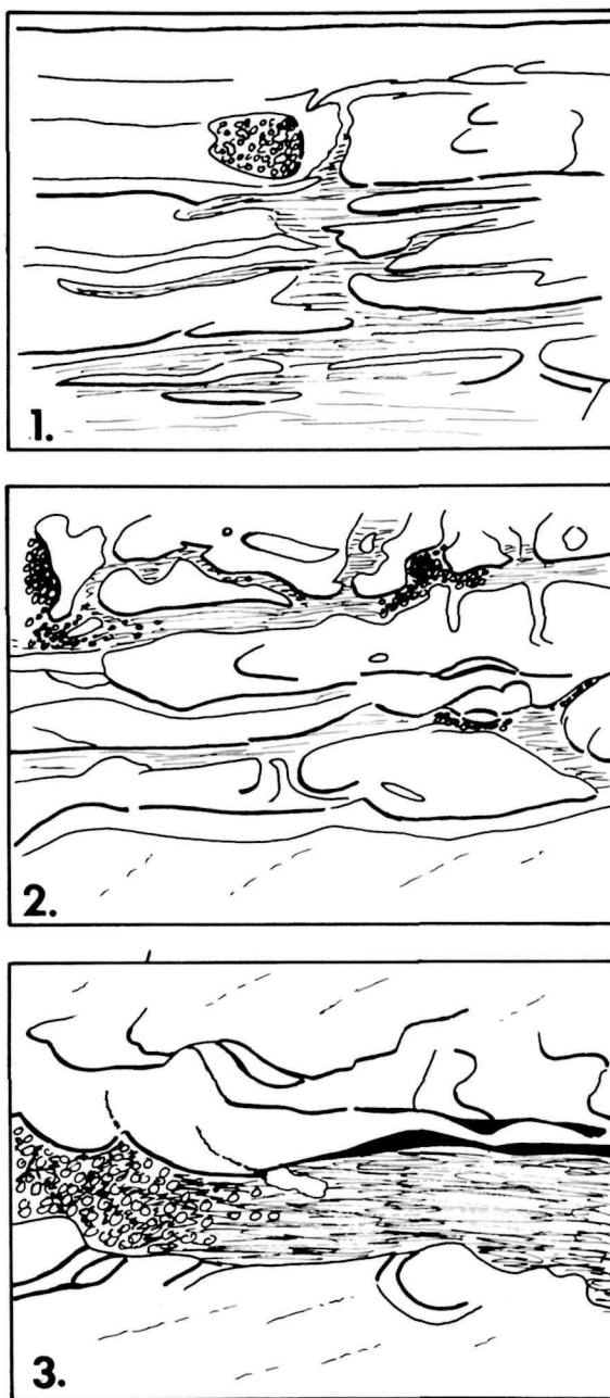
Figure 7.42. Development of experimental scour features in consolidated material through time. 1. Development of linear grooves by longitudinal vortices. 2. Groove enlargement and reduction in number by non-uniform shear stress at the bed. 3. Coalescence of grooves into single channel. Each frame measures about 30 x 40 cm. Redrawn from Shepherd and Schumm (1974, their Fig. 4).
