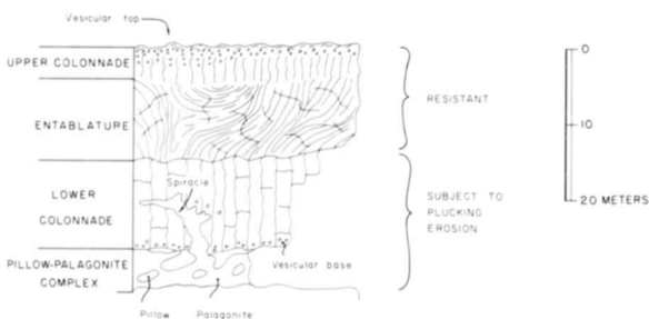
Figure 4.12. Cross section of an idealized Yakima basalt flow showing structural features important to flood erosion processes. The upper colonnade and the pillow-palagonite complex are only present in some basalt flows. Diagram is modified from Swanson (1967) and Schmincke (1967a) and uses the terminology of Tomkeieff (1940), Waters (1960) and Spry (1962).
