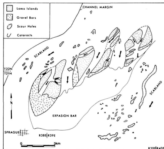
Figure 6.9. Map of the Sprague loess island assemblage.
