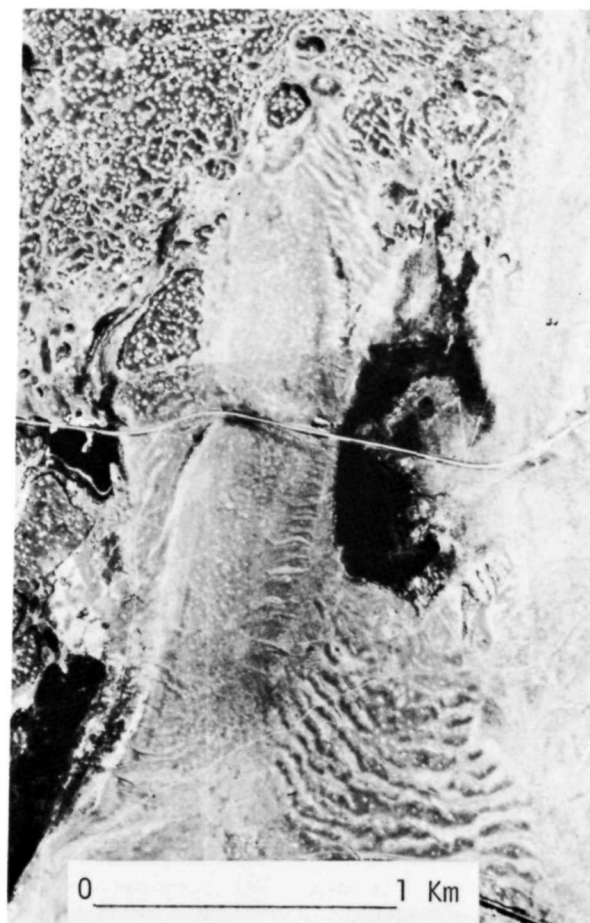
Figure 5.15. Vertical aerial photograph and topographic map of a small pendant bar in the Cheney-Palouse scabland near Macall, Washington. Contour interval is ap-
