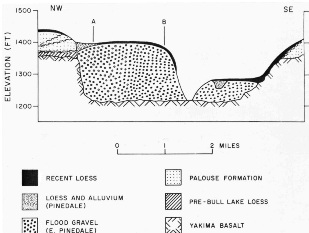
Figure 2.13. Diagrammatic cross section showing stratigraphic relationships at Staircase Rapids Bar. Thickness of the loess is slightly exaggerated.
