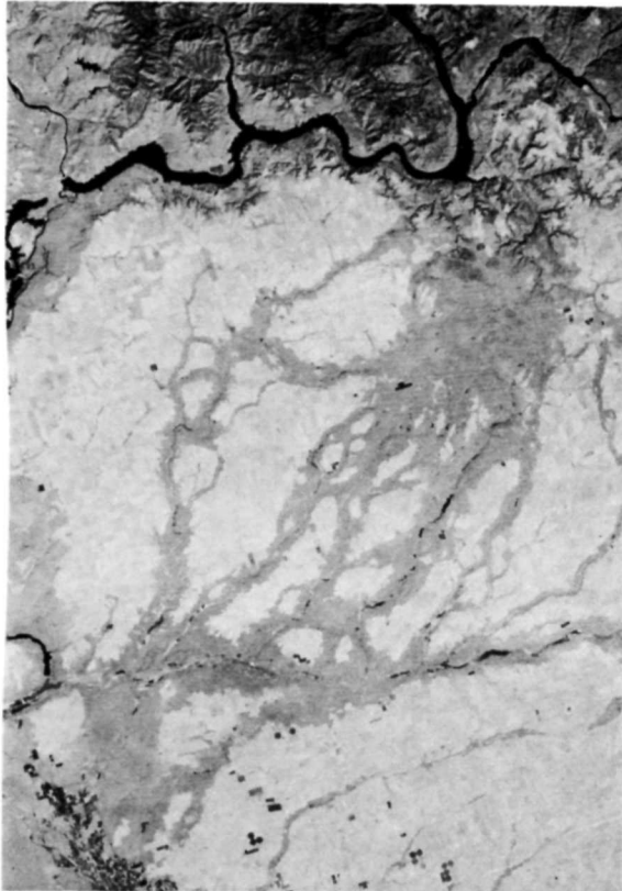
Figure 5.1. Anastomosing channel pattern in the Telford-Crab Creek scabland complex. This LANDSAT image depicts a scene 70 x 150 km (LANDSAT E-1039-18143-5, 31 August 1972).
