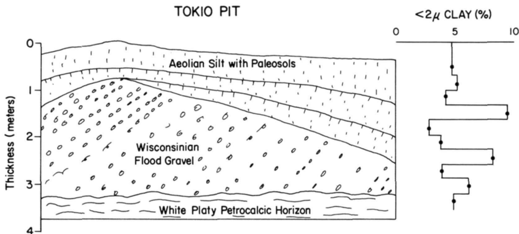
Figure 2.15. Stratigraphic relationships at the Tokio section.
