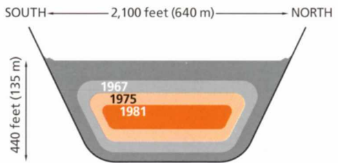
Cross section of lava lake (vertical exaggeration 2:1)
