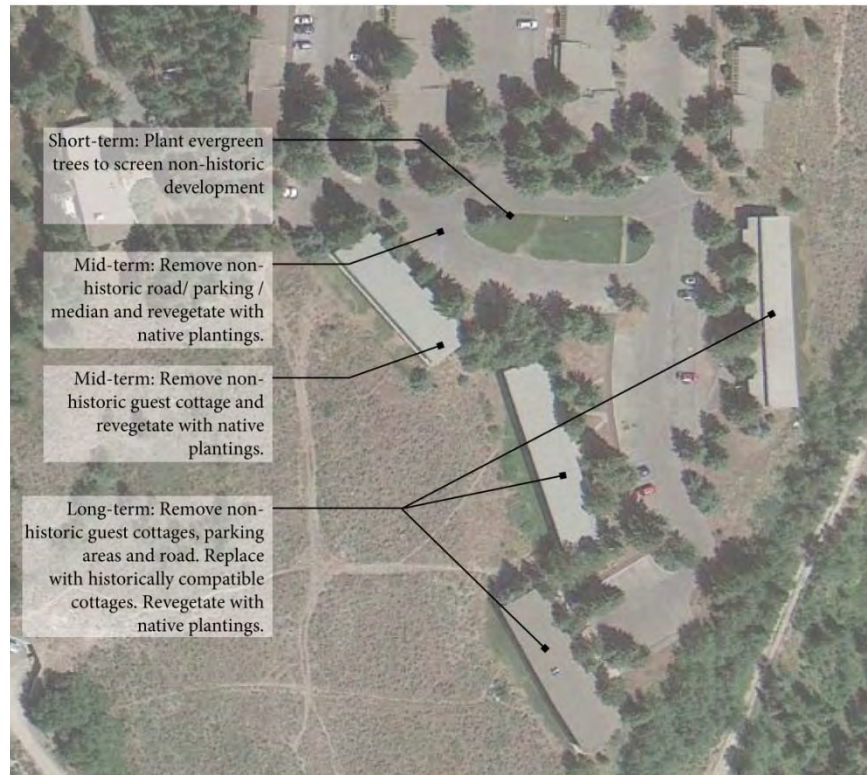
Figure 4.3. Treatment recommendations for south guest cottage area. See Figure 4.2 for recommended plant list. (Source: Logan Simpson).
