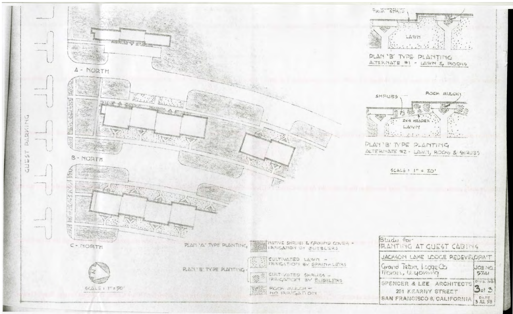
Figure 4.6. Recommended groundcover and two shrub planting schemes for Guest Cottage areas which is based on 1957 Spencer and Lee historic landscape plans and historic photography. Note turf areas denoted on plan. See Figure 4.3 for recommended species list. (Source: NPS).
