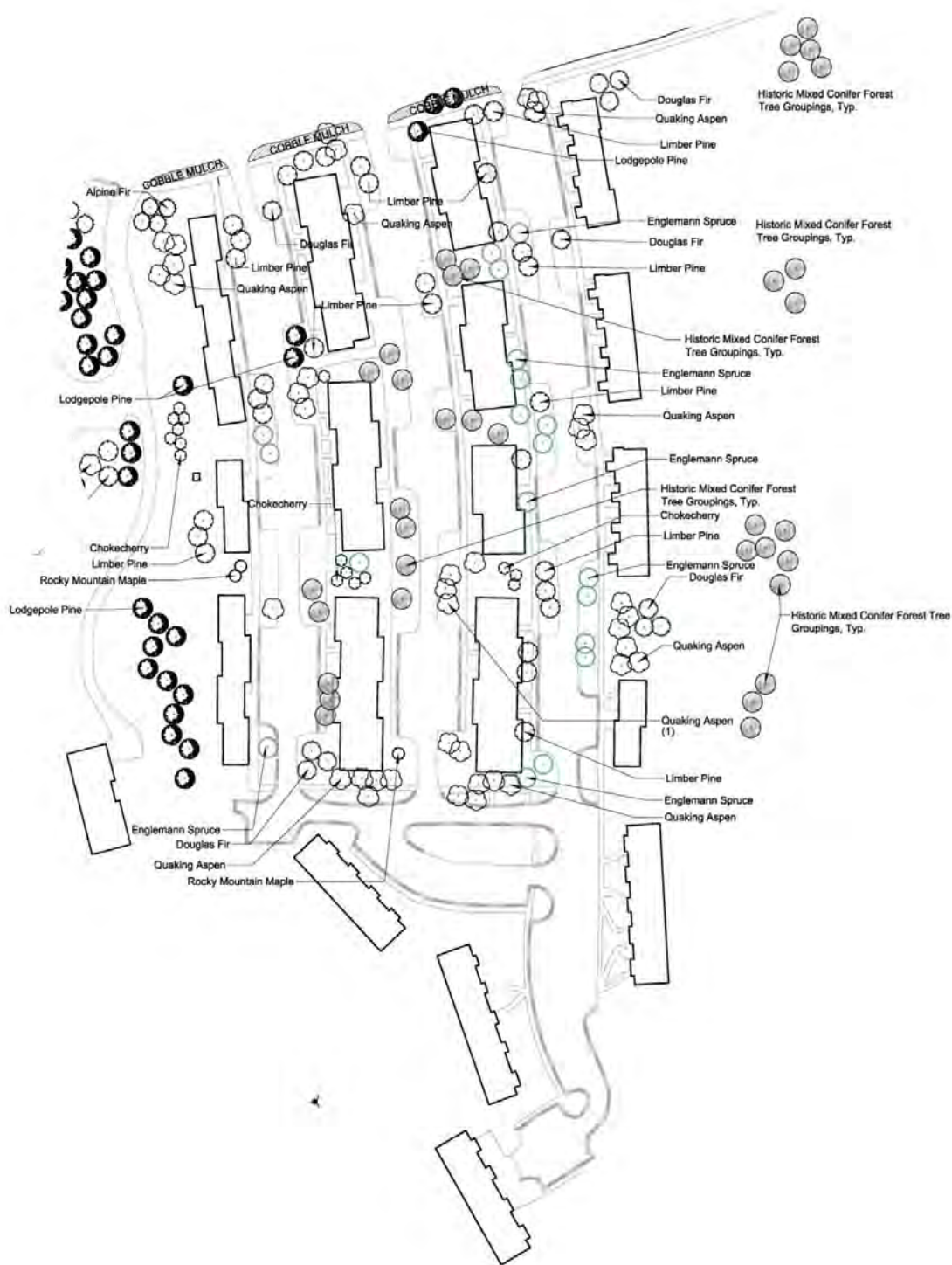
Figure 4.7. Recommended tree landscape treatment for the South Guest Cottages which is based on historic photography and the 1955 Mortimore and Wirth landscape plan, as no information related to trees or shrubs was provided in Spencer and Lee landscape plans. Refer to Figure 4.3 for recommended areas to be screened and Figure 4.2 for recommended plant list. Refer to Figure 4.6 for historic groundcover and shrub plantings. (Source: Logan Simpson).
