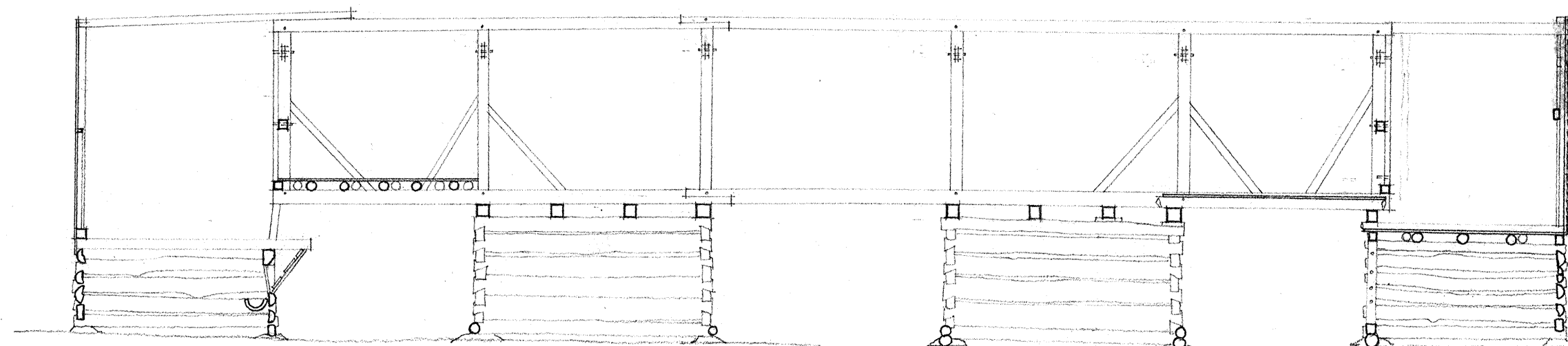
SECTION B-B
