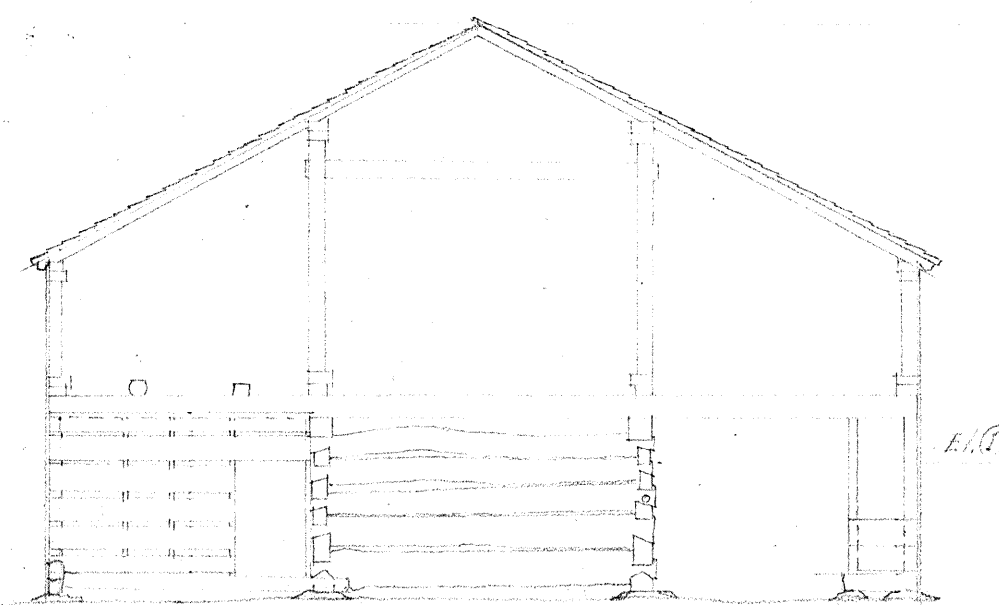
SECTION G-G
