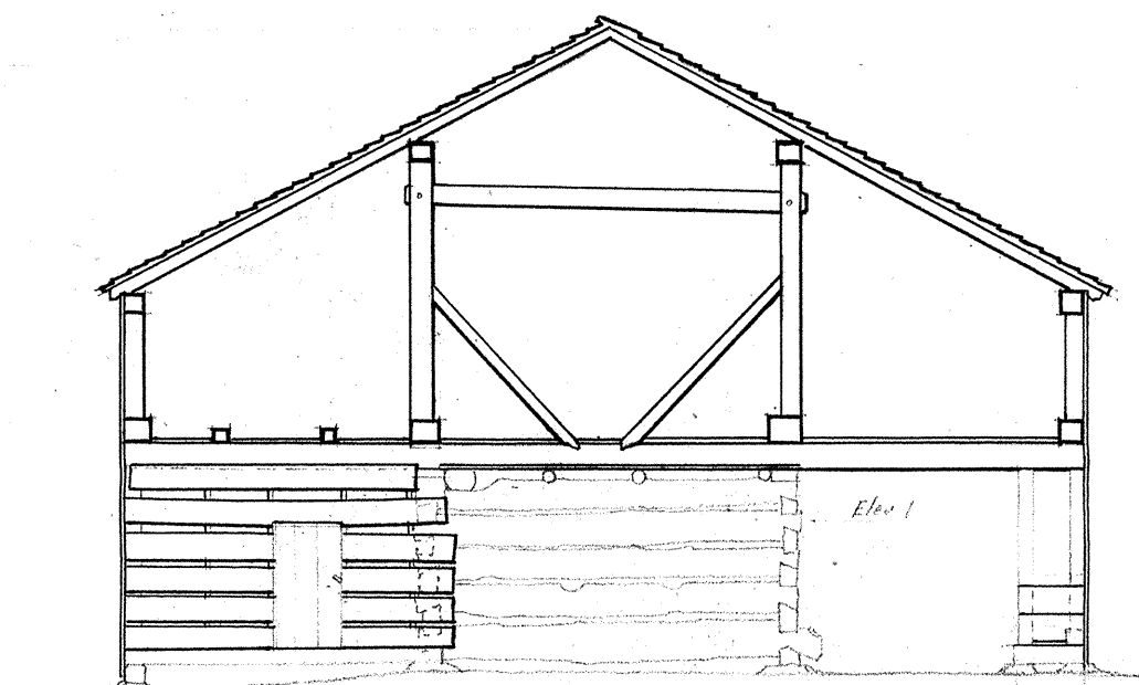
SECTION E-E
