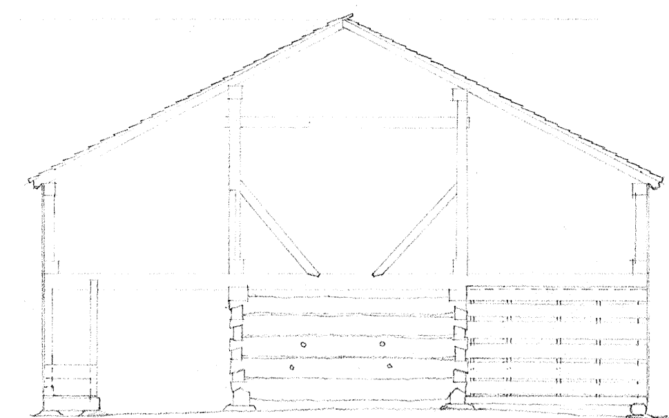
SECTION H-H
