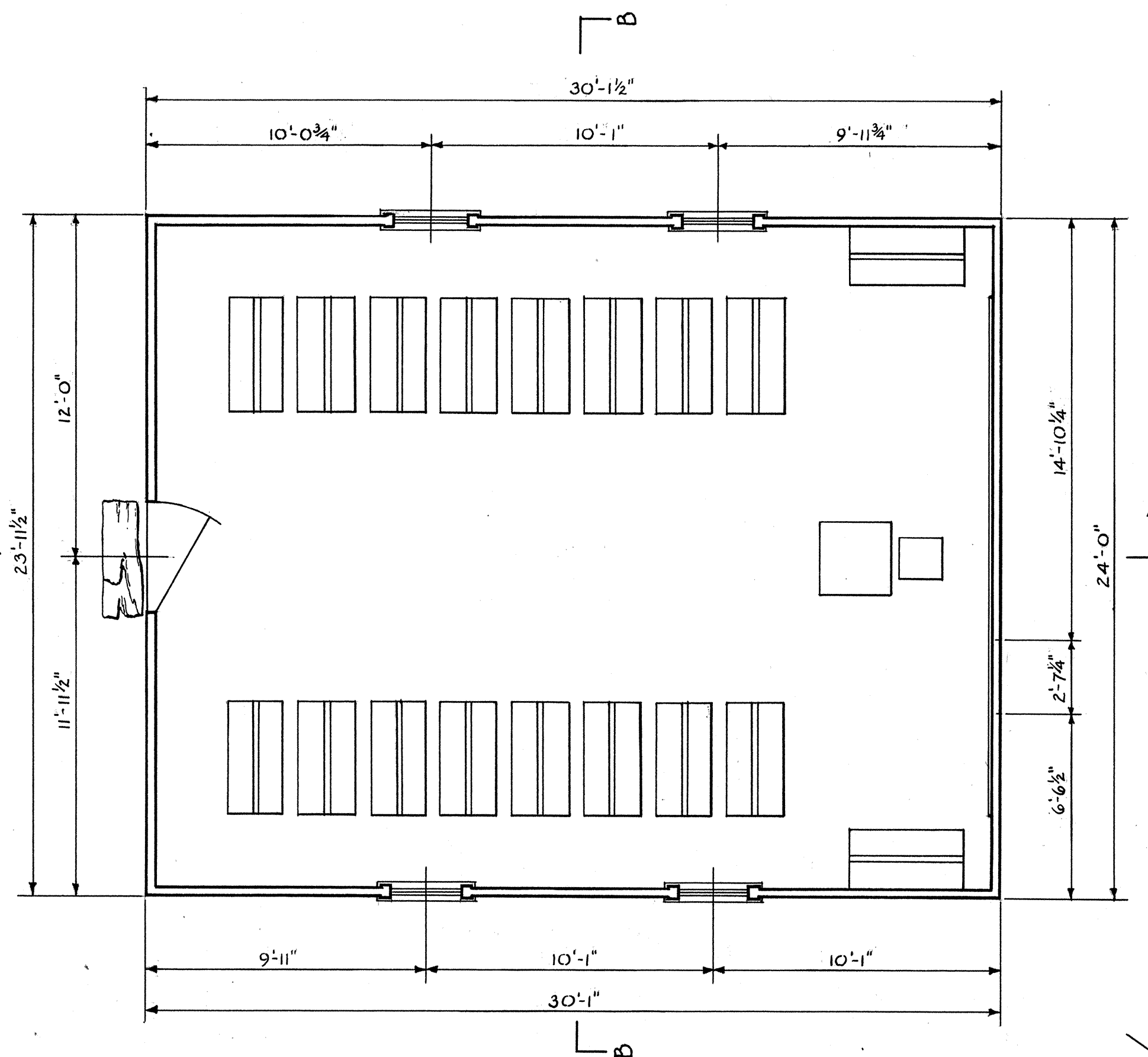
PLAN
