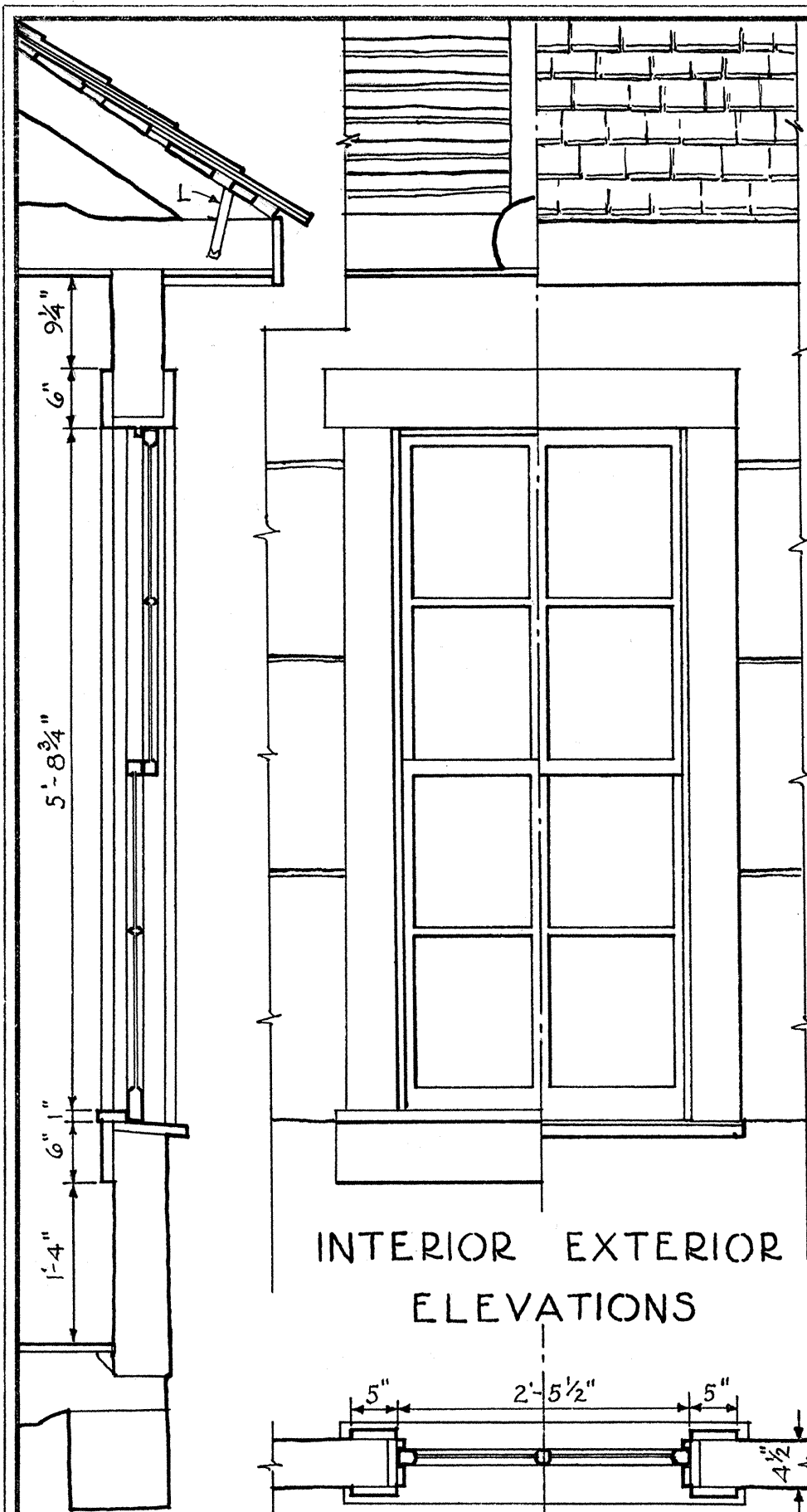
SECTION PLAN WINDOW DETAILS
