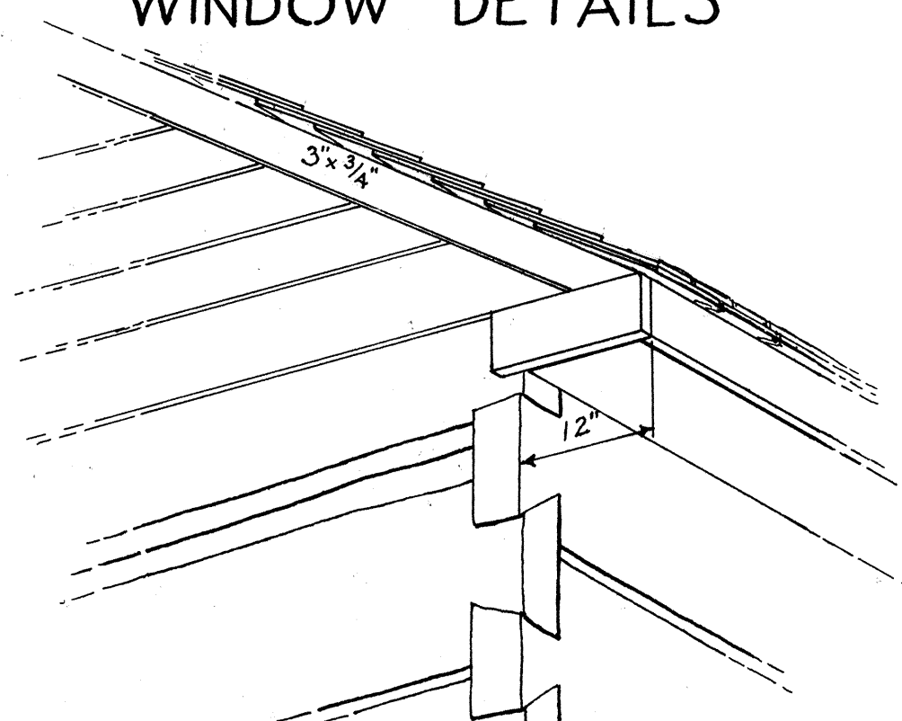
CORNER DETAIL
