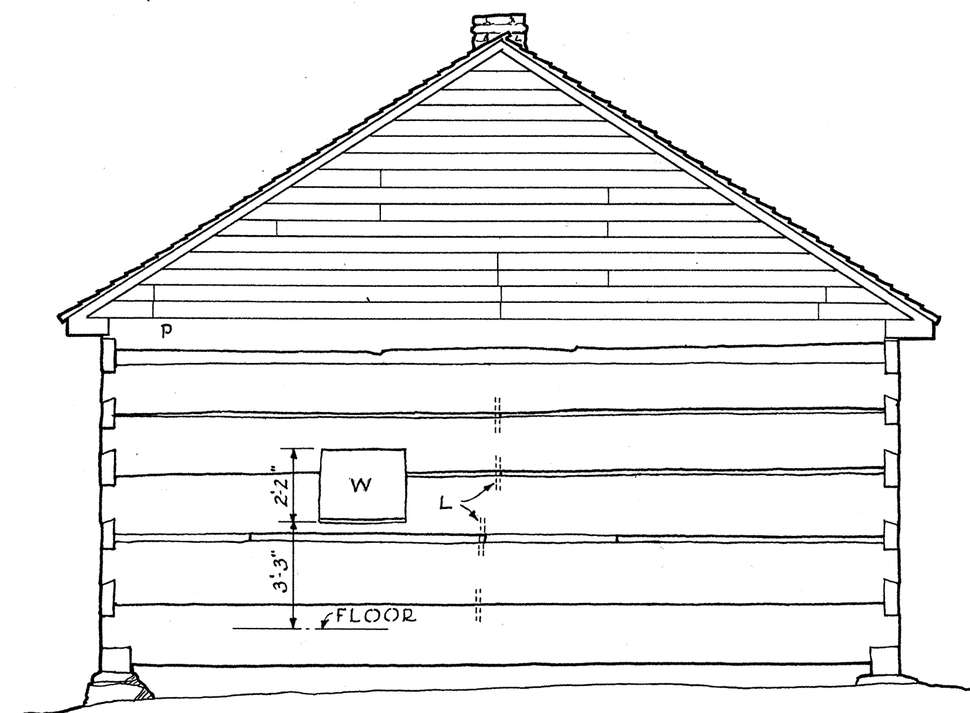
SOUTH ELEVATION
