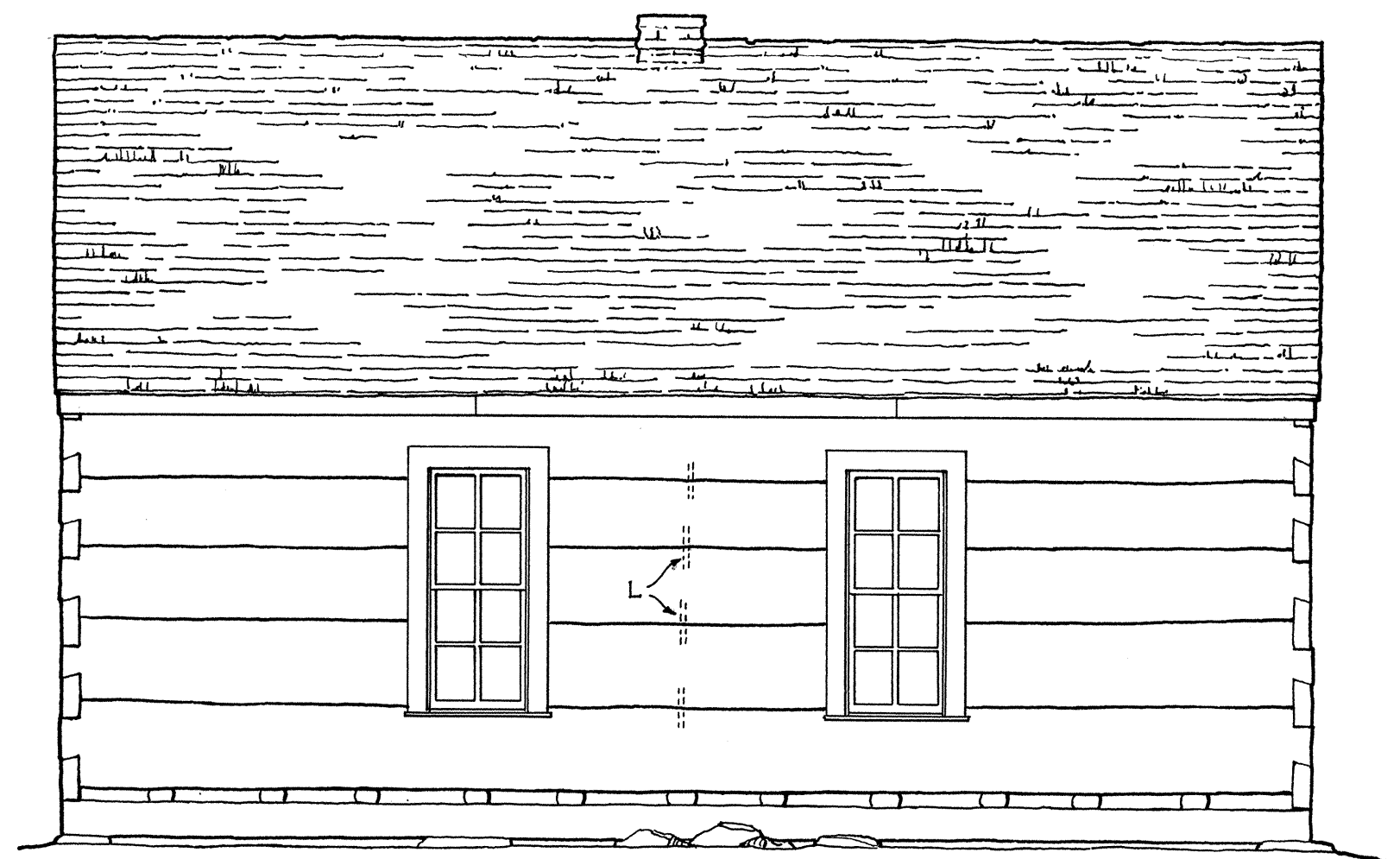
EAST ELEVATION
