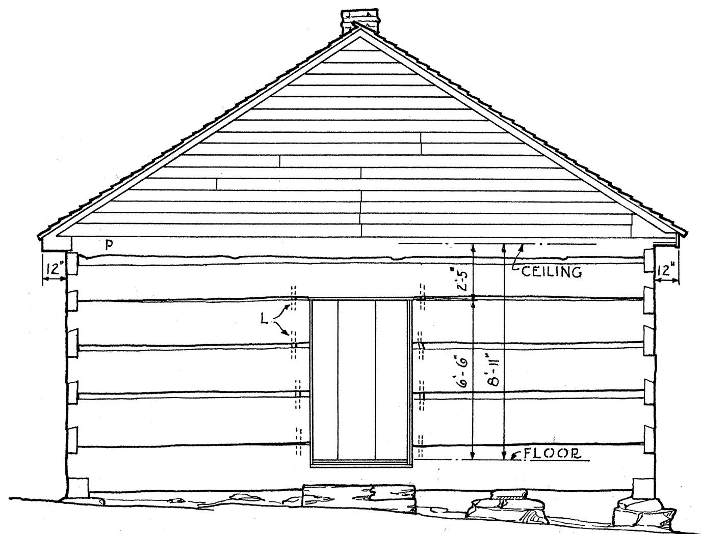
NORTH ELEVATION
