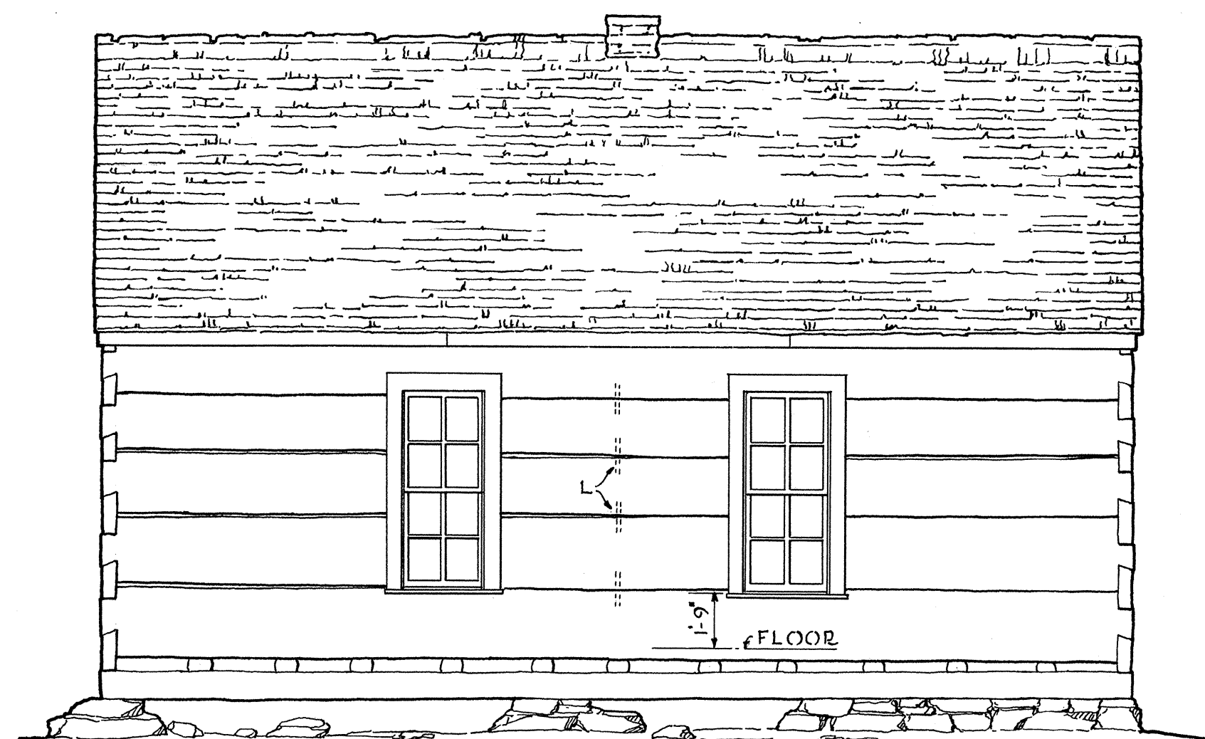
WEST ELEVATION
