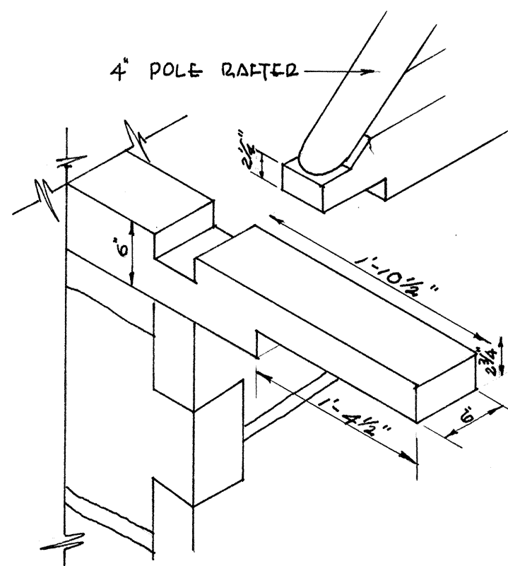
DETAIL AT "C"
