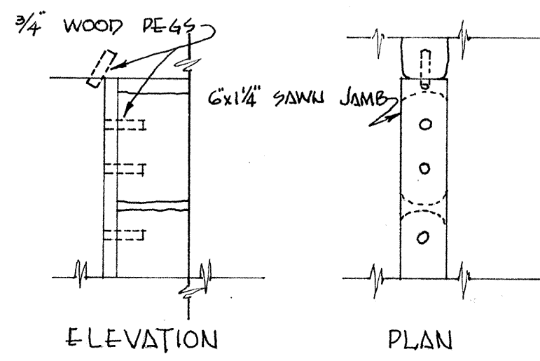
DETAIL AT "D"
