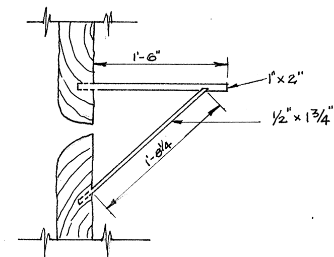
DETAIL AT "F"
