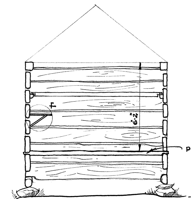
SECTION B-B
