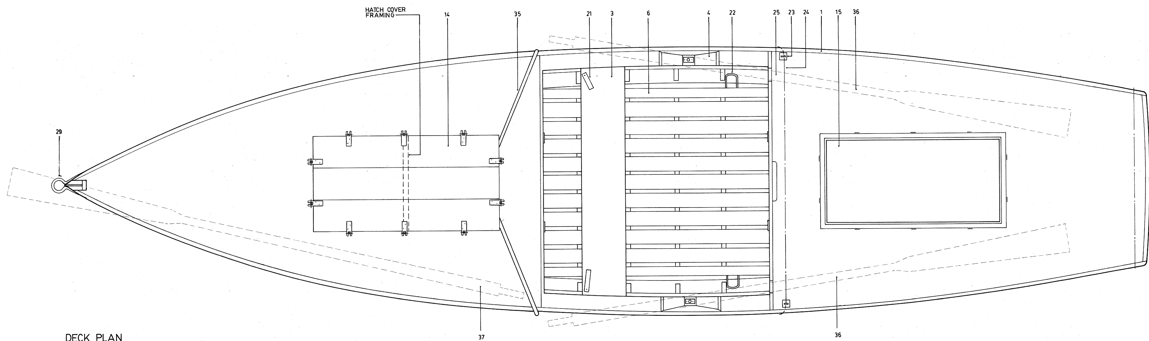
DECK PLAN
