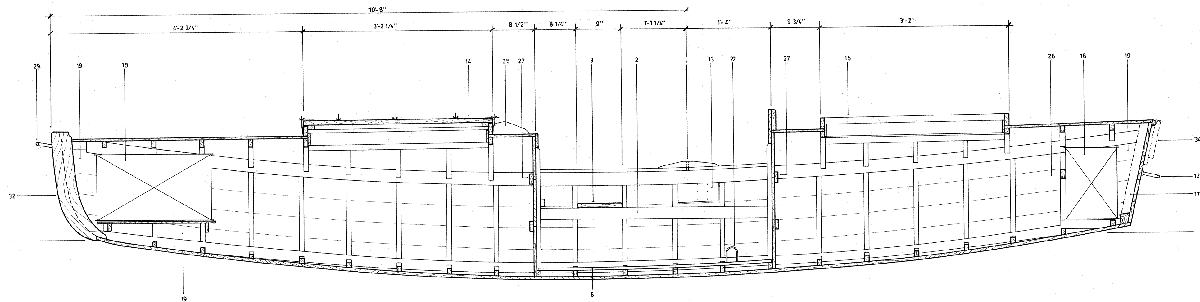
LONG SECTION
