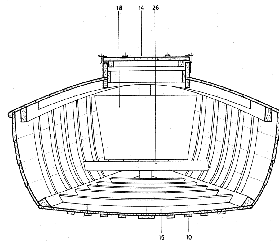
SECTION AT HATCH
