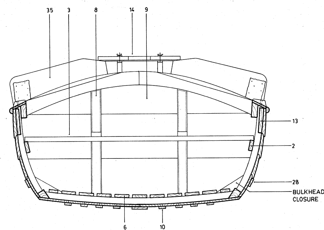
MID-SHIPS SECTION LOOKING FORWARD
