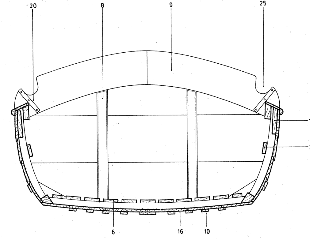
MID-SHIPS SECTION LOOKING AFT
