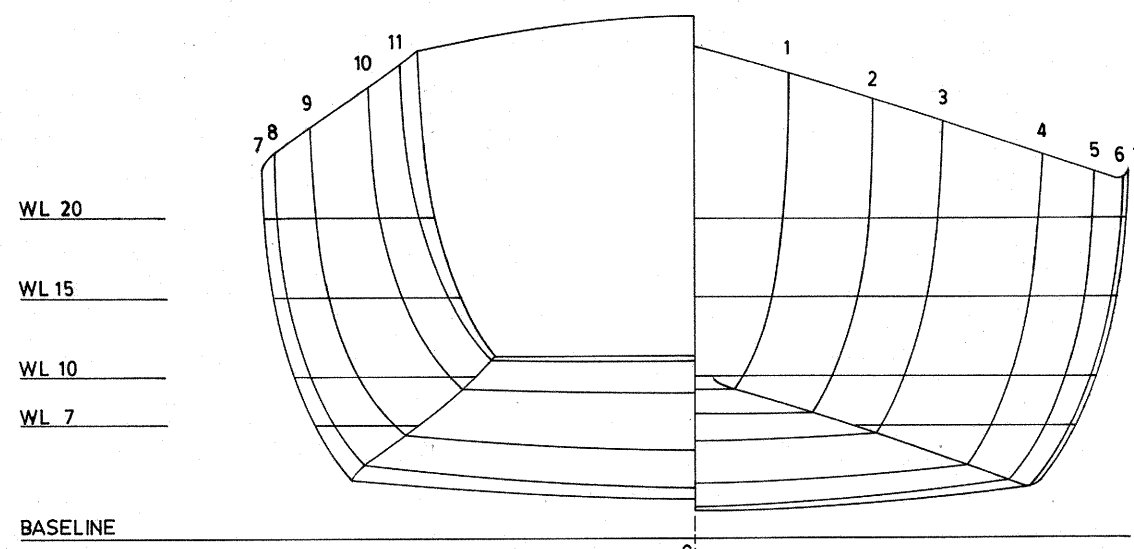
BODY PLAN
