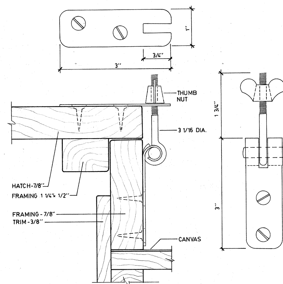
HATCH DETAILS
