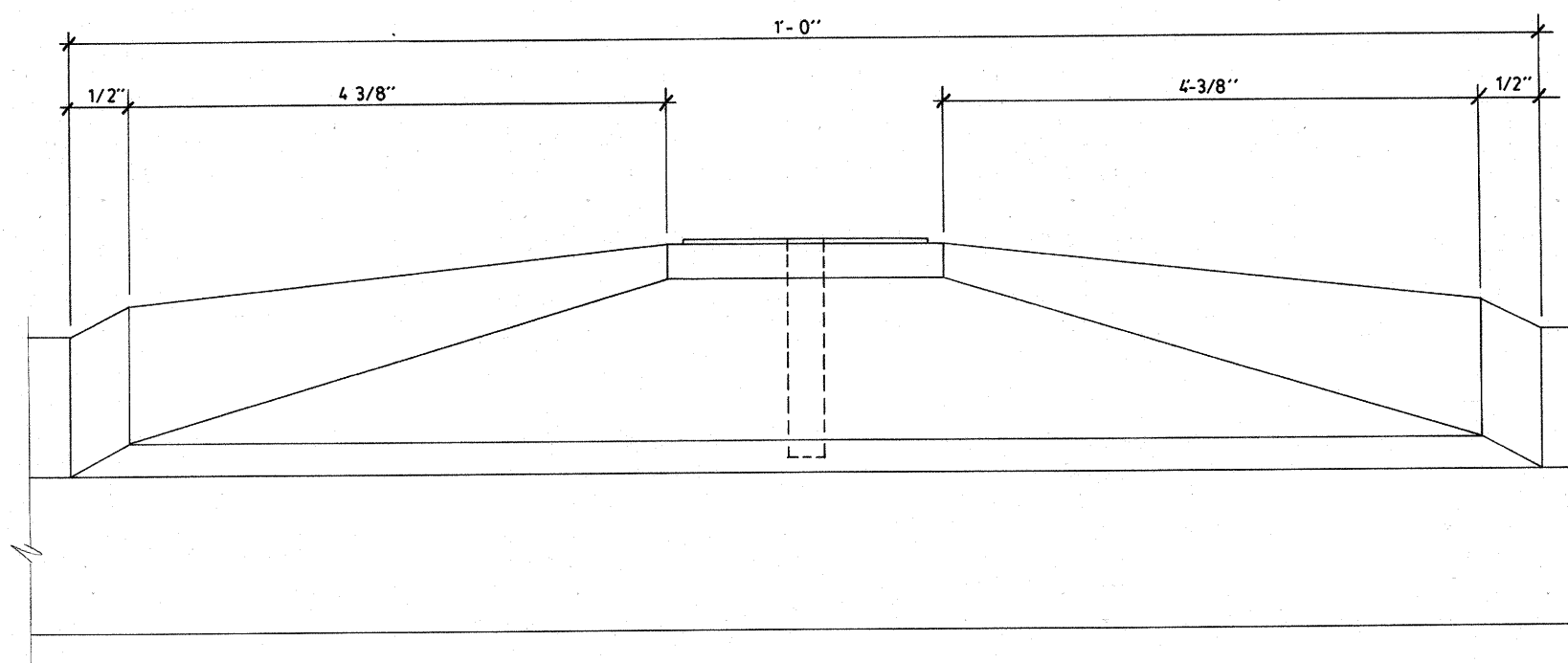
OARLOCK PAD DETAILS
