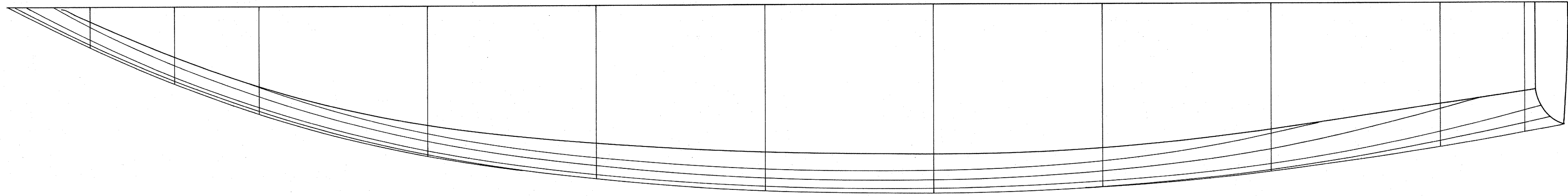
HALF BREADTHS PLAN
