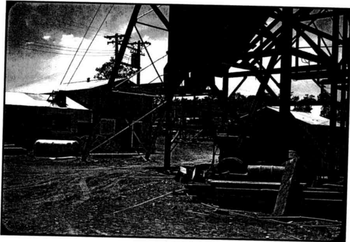
Photo 2. Ore bin attached to headframe of Orphan Mine. Note back bracing strut bisects angle formed by hoisting rope and rear legs of headframe (Source: NPS, 1959).
