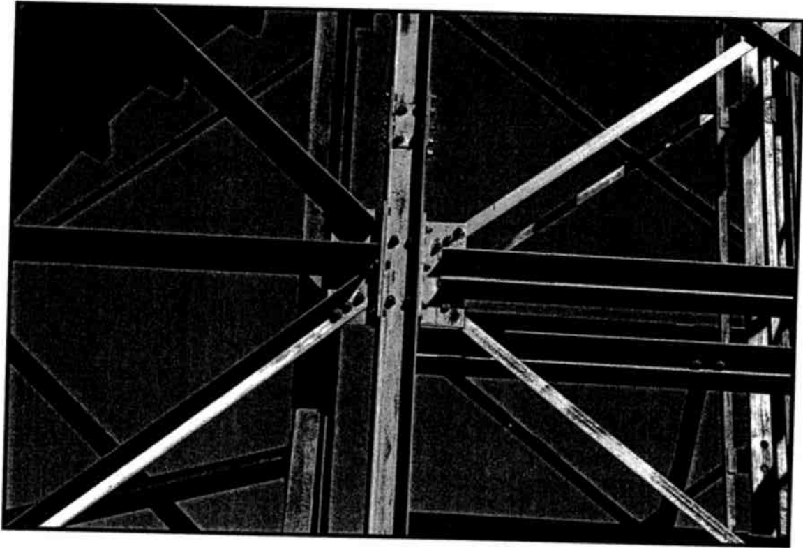
Photo 3. View of typical bolted connection of struts and bracing members to headframe leg (Source: George Weaver, 2005. No copyright restrictions).
