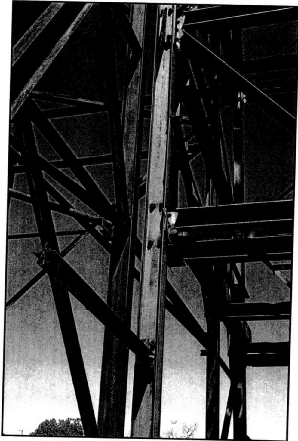
Photo 5. View of cut members remaining attached to rear leg of headframe (Source: George Weaver, 2005. No copyright restrictions).
