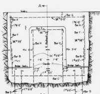
Steel abutments Scale 1"-1'
