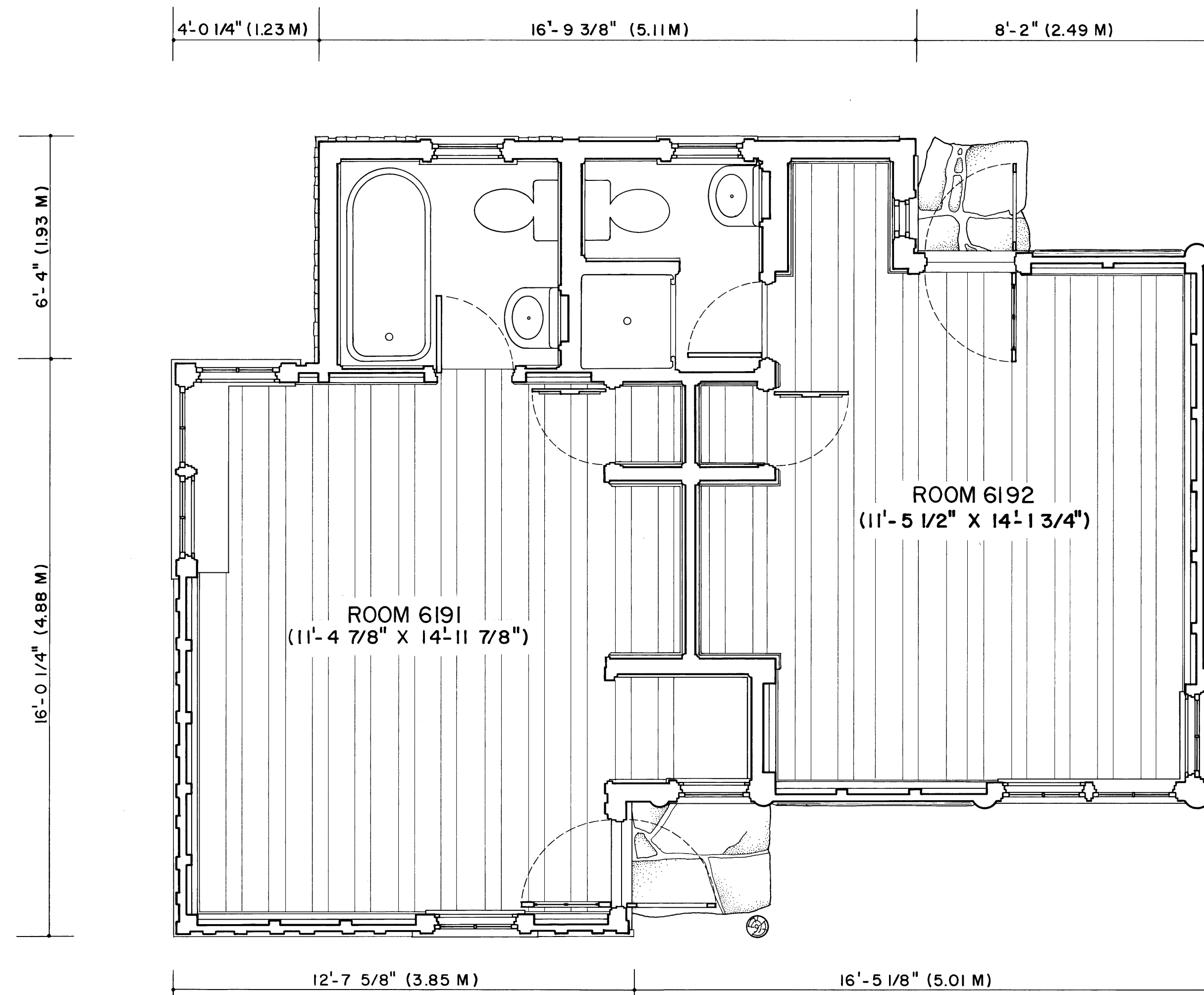
FLOOR PLAN
