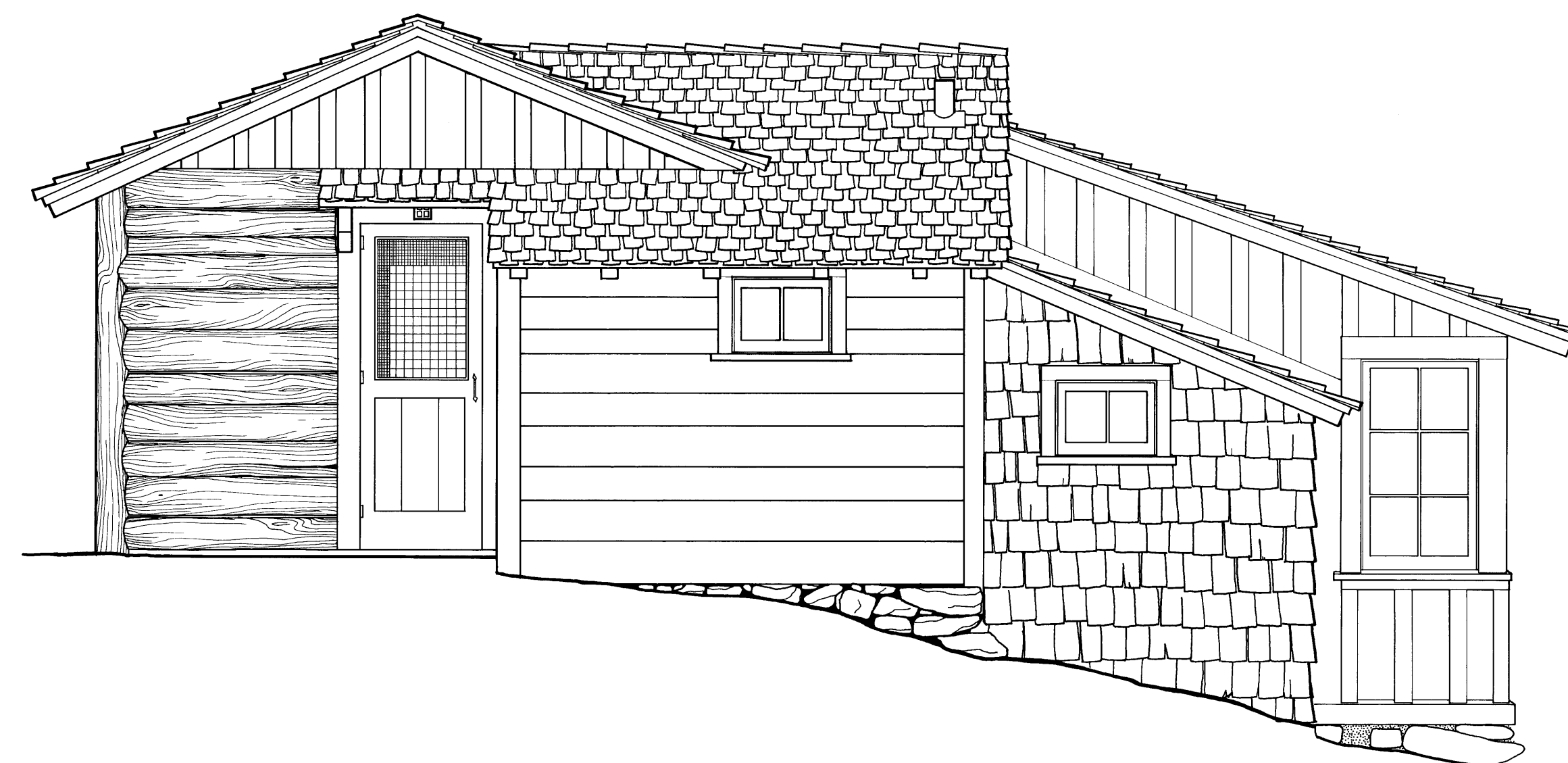
NORTH ELEVATION
